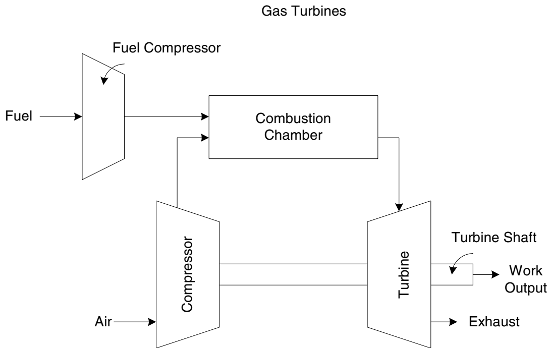
Figure 2-1. Simple-Cycle Gas Turbine
