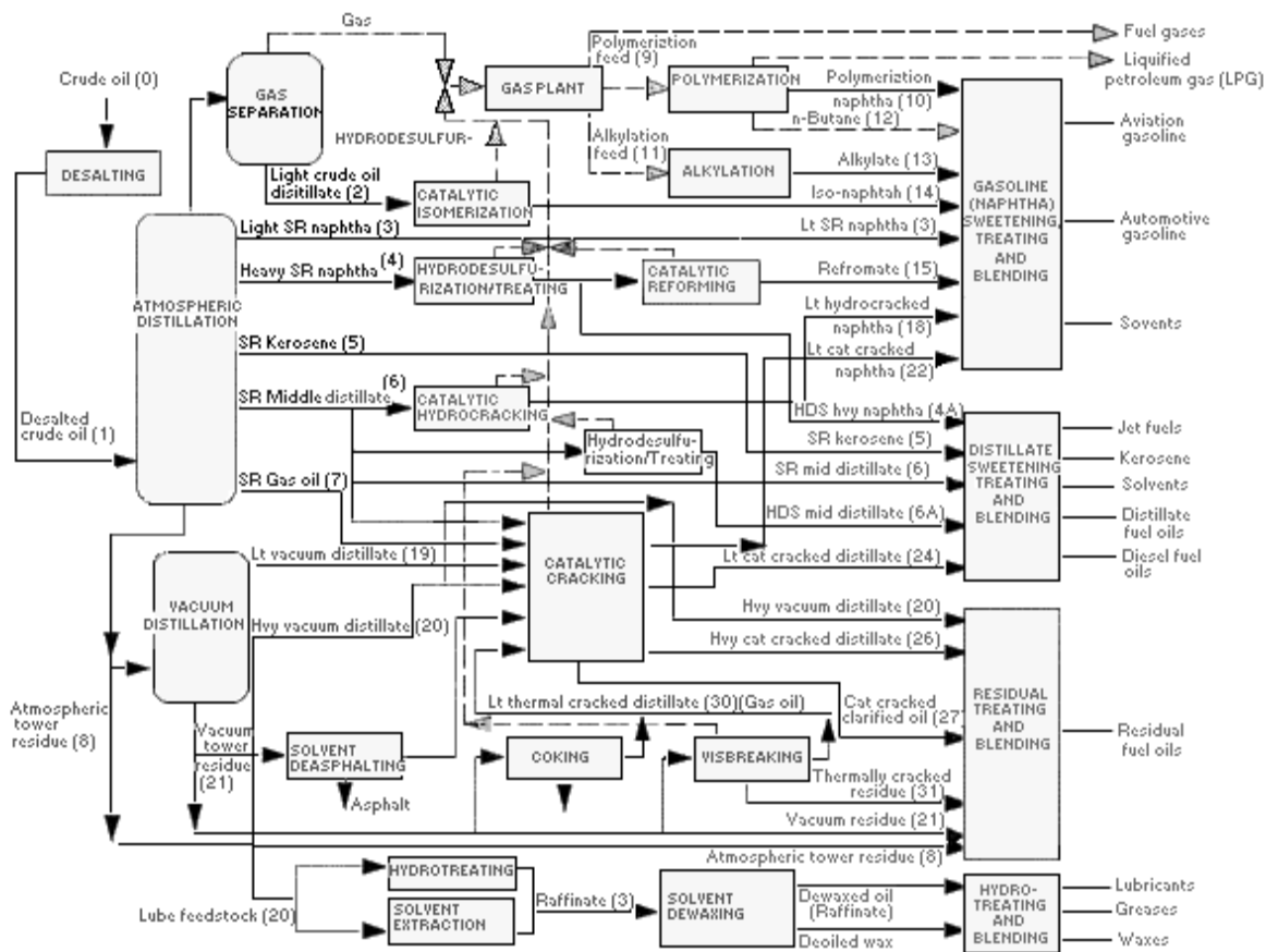
Figure 2-1 Outline of the Refining Process
