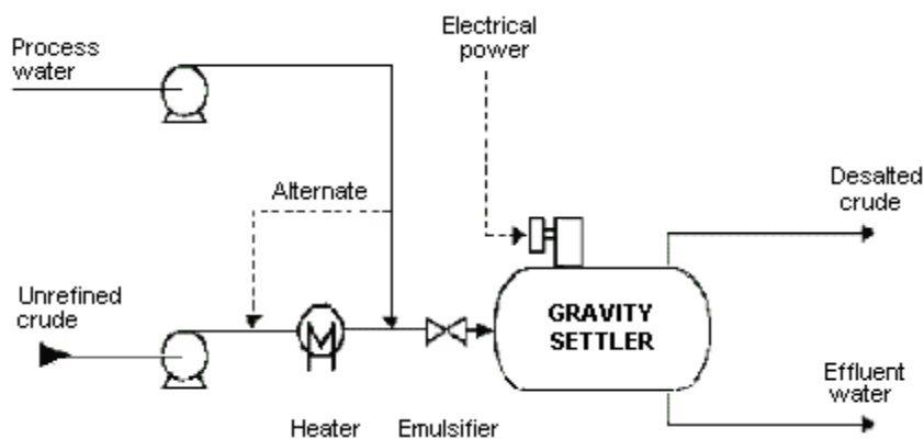
Figure 2-2 Desalting Process
