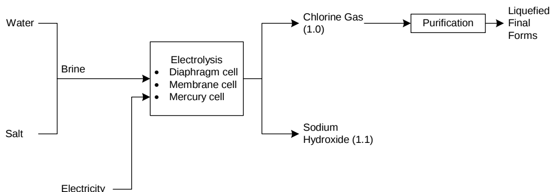
Figure 2-1. Chlor-Alkali Process
