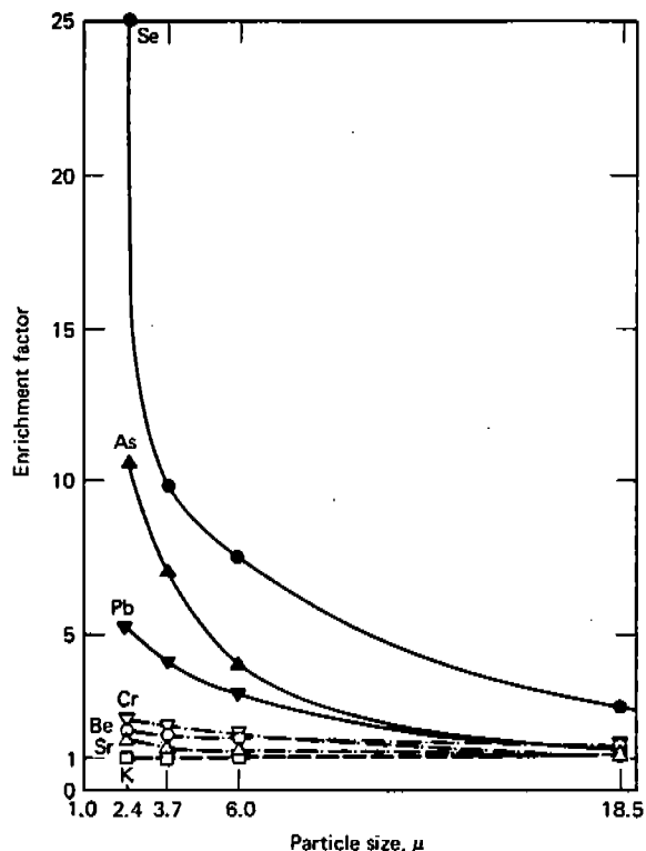
Figure 1. Enrichment factors of selected elements vs. particle size in stack fly ash collected downstream from an electrostatic precipitator (ESP). Errors in data are given in Table III. Group I element (---), Group II elements (—), and Group III elements (- · -)
