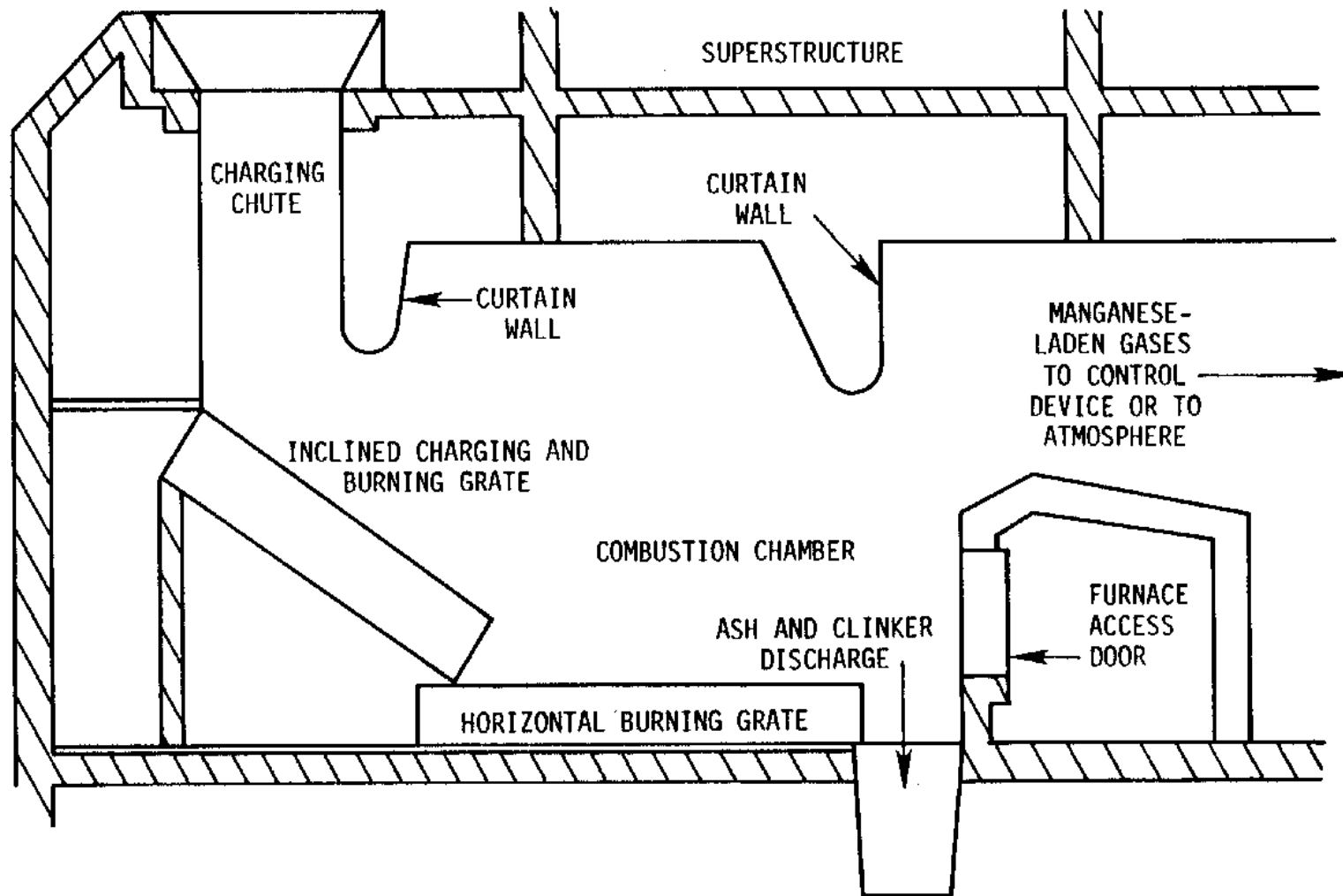
Figure 5-2. Basic configuration of a municipal refuse incinerator. 2
