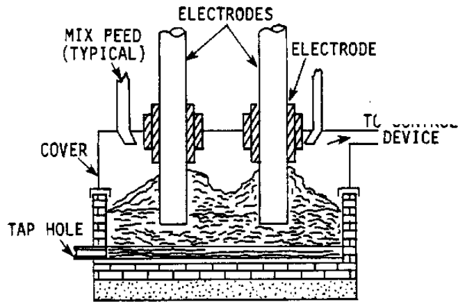
Figure 4-4. Sealed furnace.
