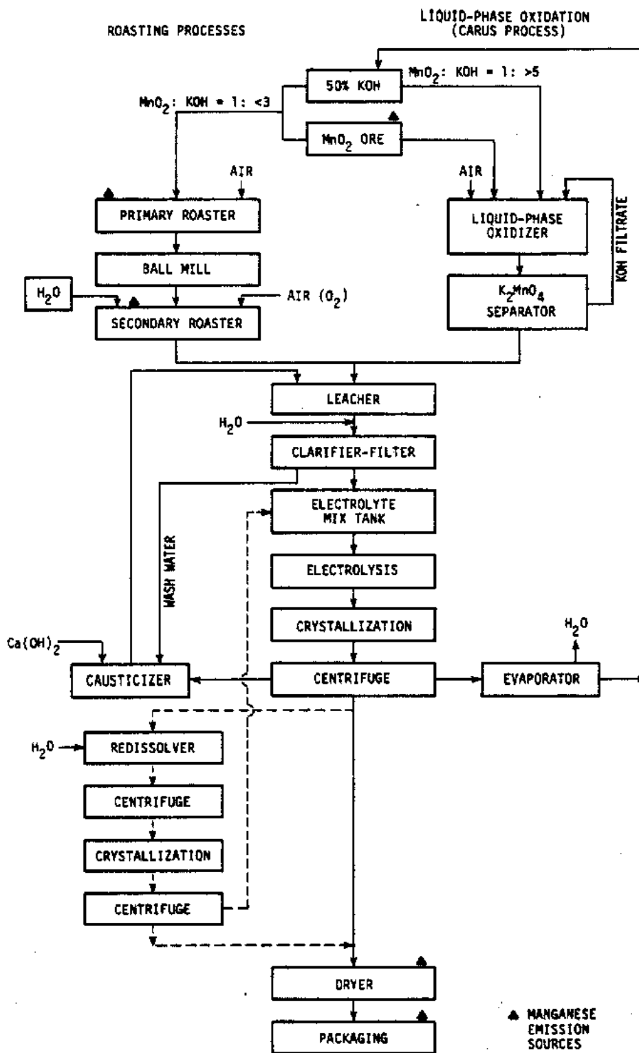
Figure 4-7. Production of KMnO_4 : roasting and liquid phase oxidation processes. 1
