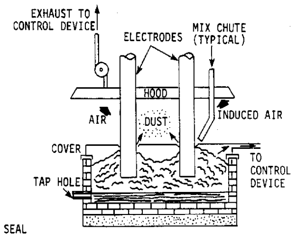
Figure 4-3. Semisealed furnace.
