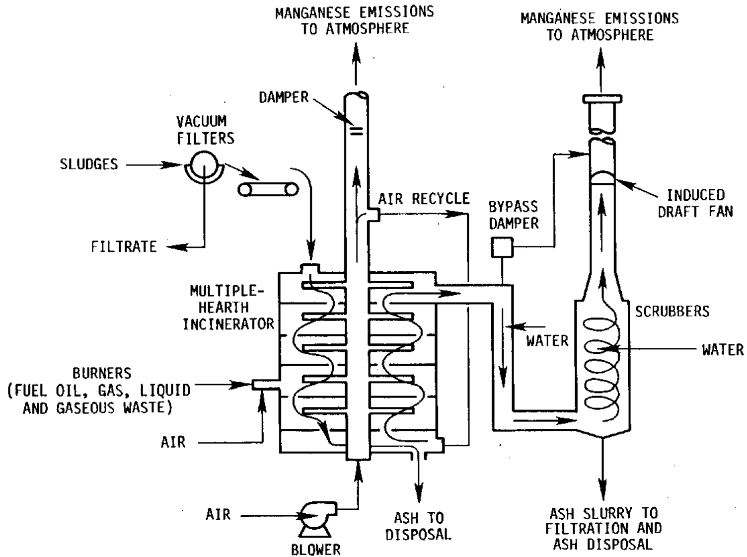
Figure 5-3. Schematic of a typical multiple-hearth incineration system. 4
