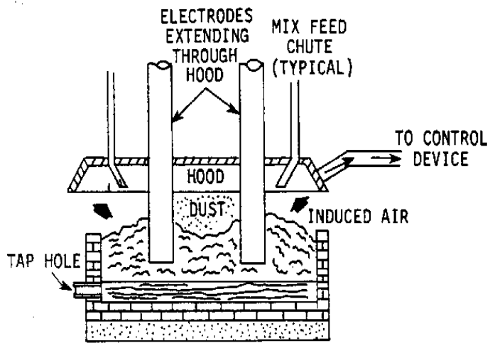
Figure 4-2. Open furnace.
