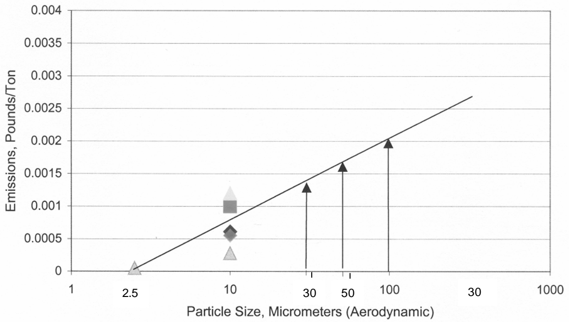
Figure 1. PM Emission Factor Calculation, Screening (Controlled)
