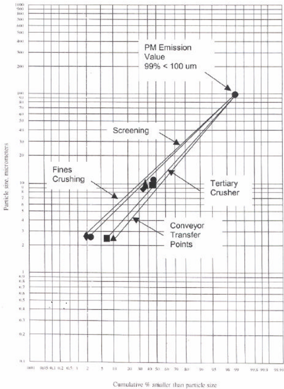
Figure 5. Log Probability Plot Used to Check Estimated PM Emission Factors
