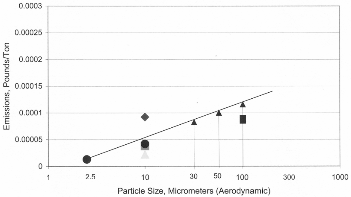
Figure 4. PM Emission Factor Calculation, Conveyor Transfer Points (Controlled)
