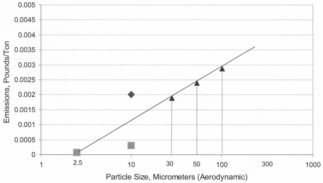
Figure 3. PM Emission Factor Calculation, Fines Crushing (Controlled)
