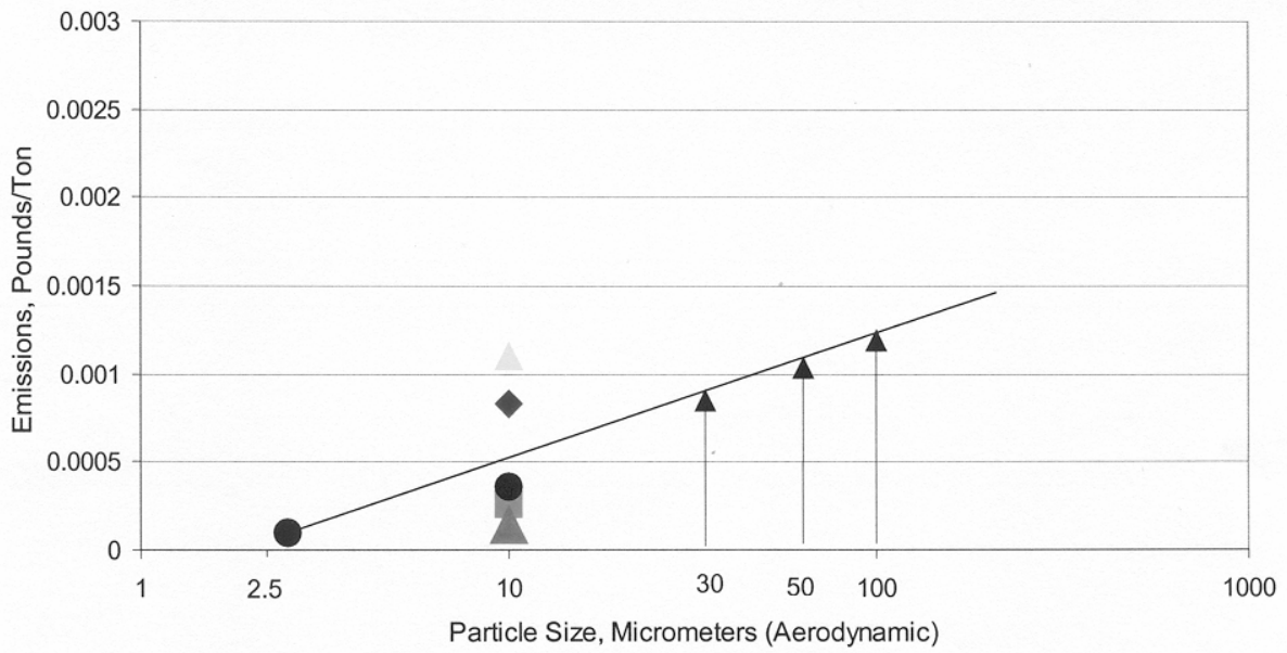
Figure 2. PM Emission Factor Calculation, Tertiary Crushing (Controlled)
