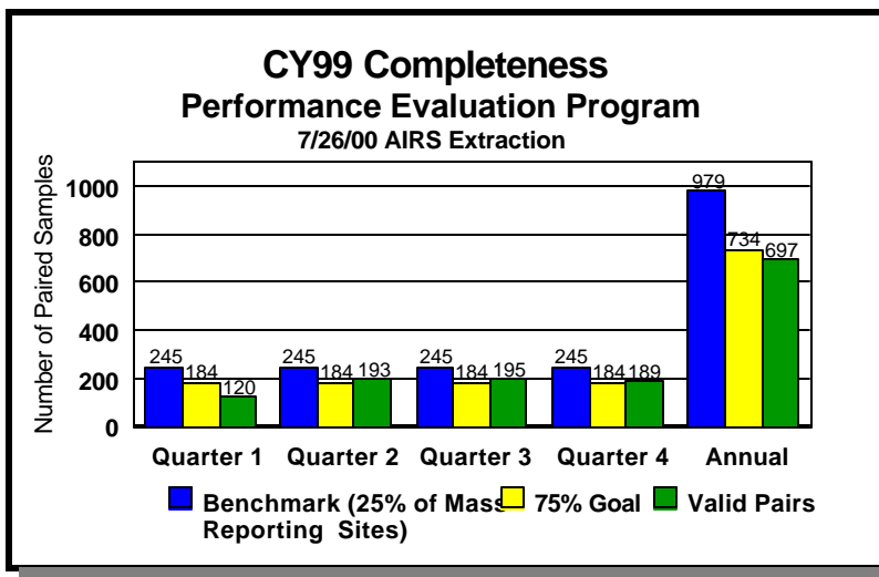
Figure 2.9 Completeness of Performance Evaluation/routine sample pairs
