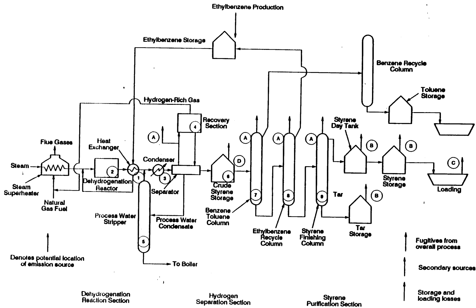
Figure 3. Process Flow Diagram for Styrene Production by Ethylbenzene Dehydrogenation 3
