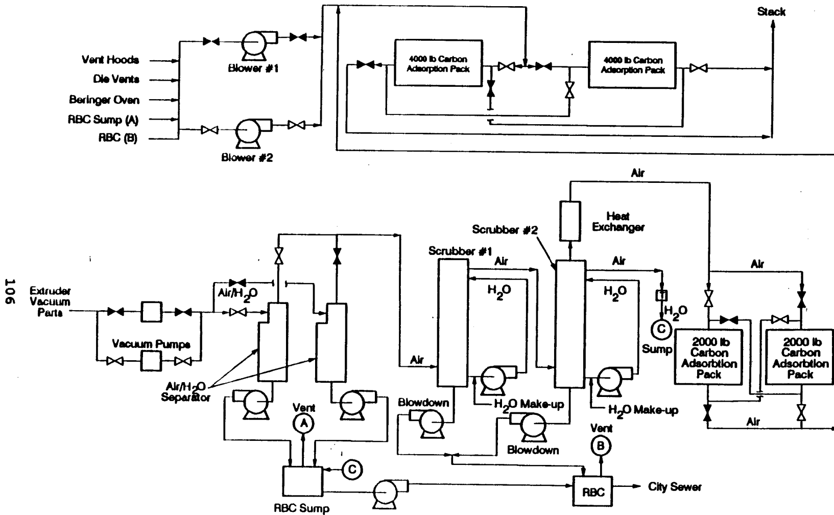
Figure 20. Permanent VOC Controls at an ABS Compounding Facility
