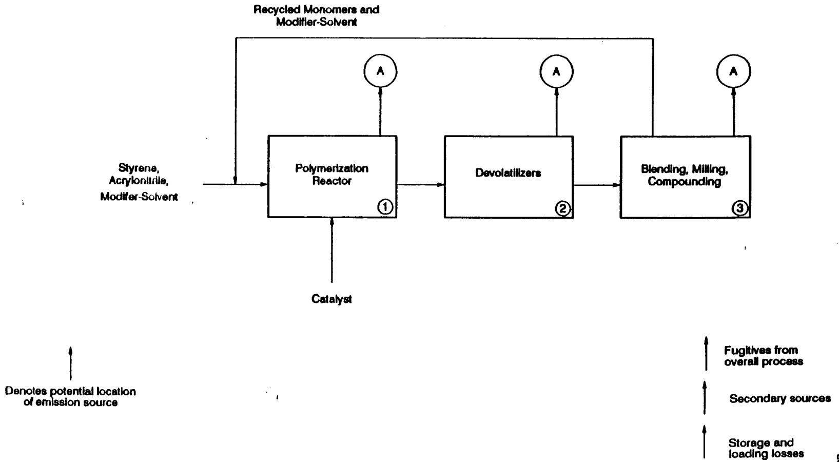
Figure 13. Production of SAN by Continuous Mass Polymerization 21
