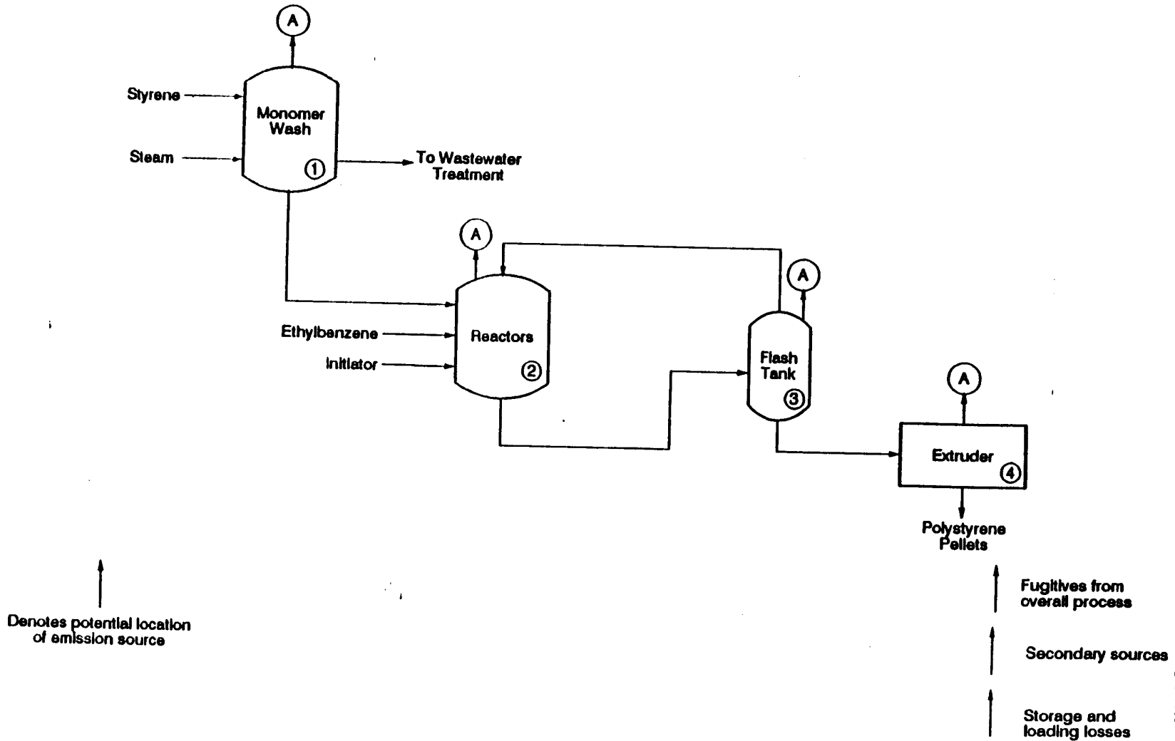
Figure 8. Polystyrene Production by Solution Polymerization 3
