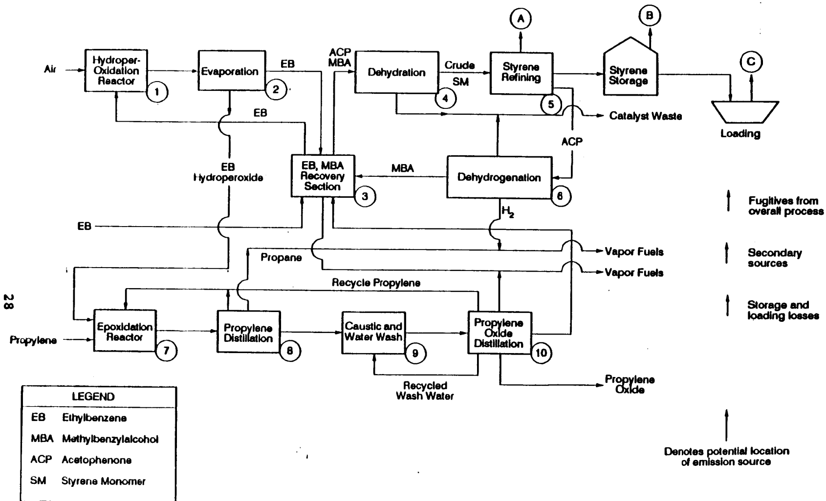
Figure 4. Process Flow Diagram for Styrene Production by Ethylbenzene Hydroperoxidation 4
