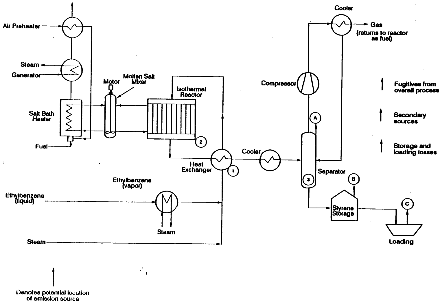
Figure 5. Process Flow Diagram for Styrene Production by Isothermal Processing 5
