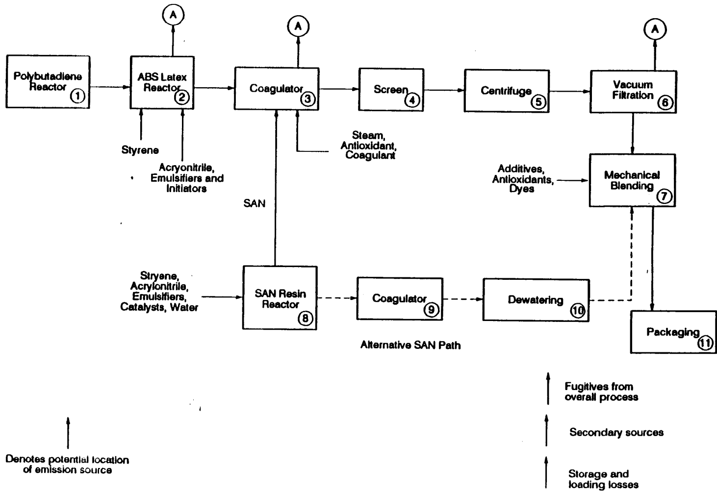
Figure 14. Production of ABS/SAN by Emulsion Polymerization 11
