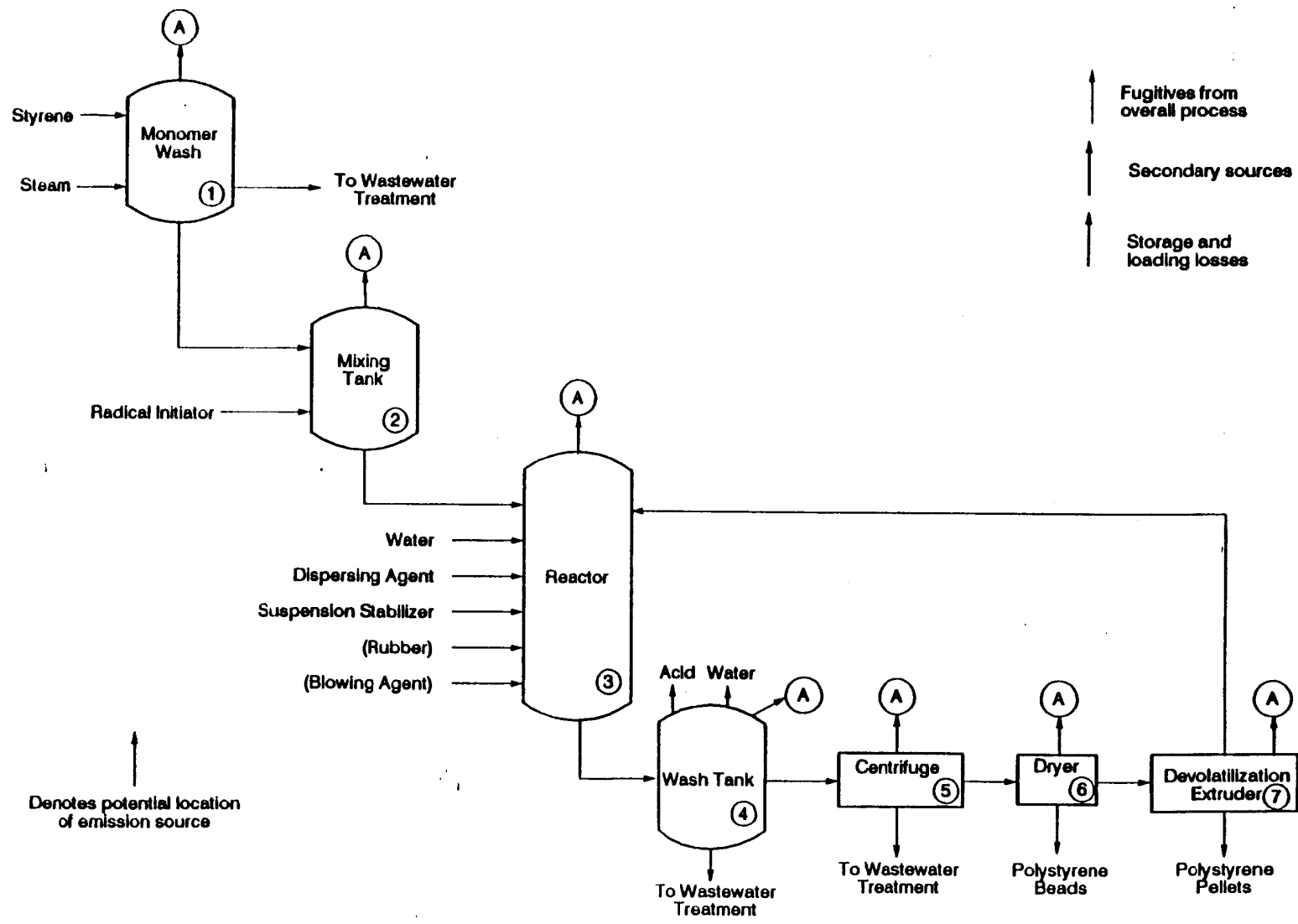
Figure 6. Polystyrene Production by Suspension Polymerization 3
