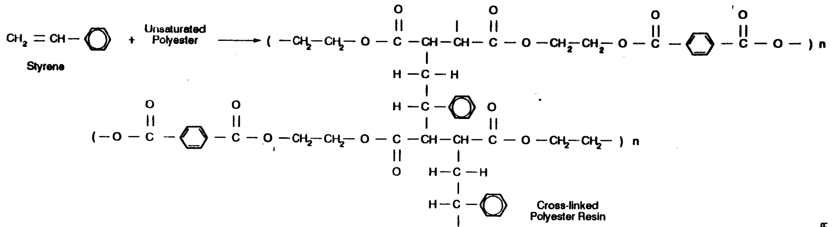
Figure 17. Typical Reaction for Unsaturated Polyester and Polyester Resin Formation 27
