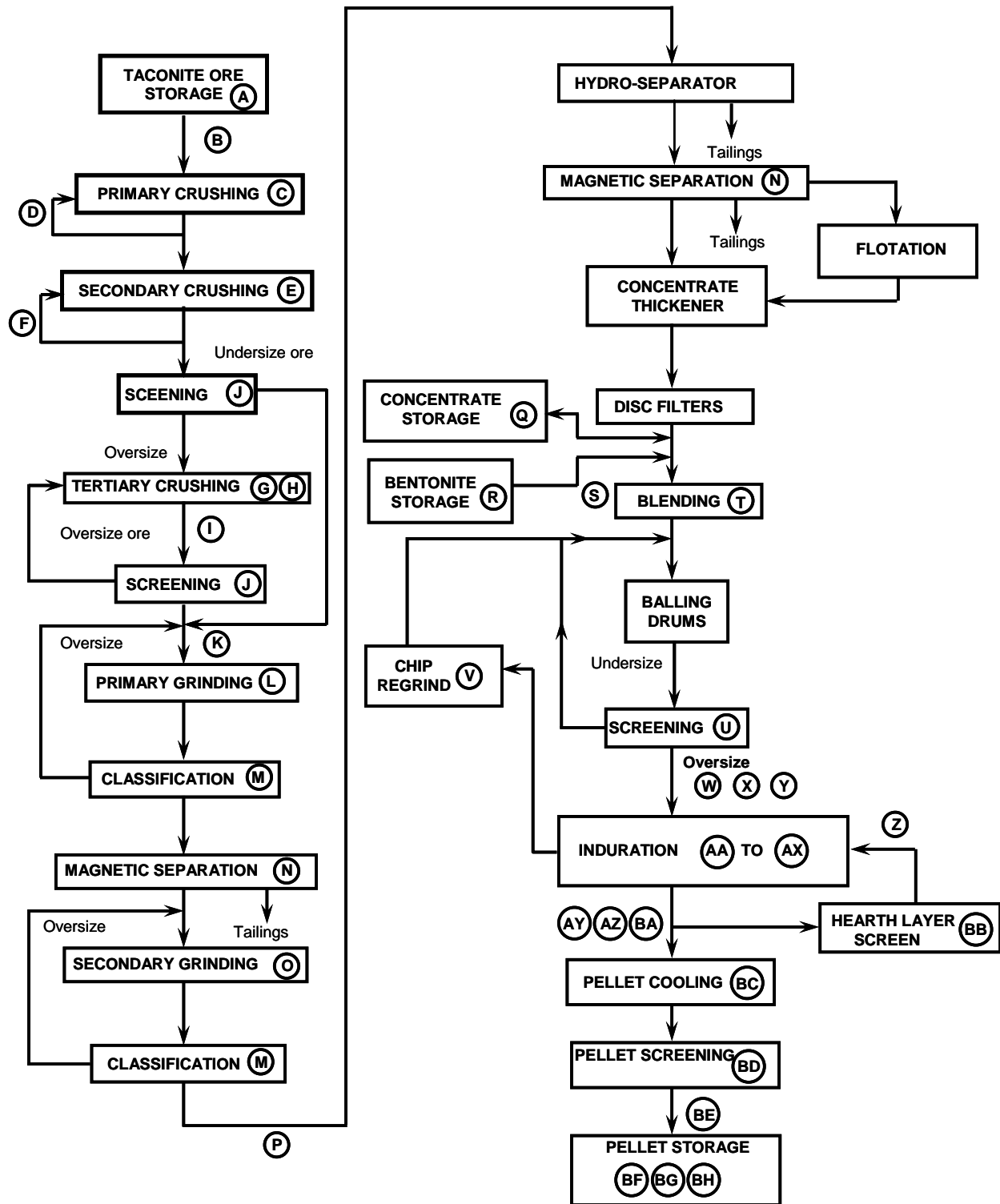
Figure 11.23 - 1. Process flow diagram for taconite ore processing. (Refer to Table 11.23-1 for Source Classification Codes)
