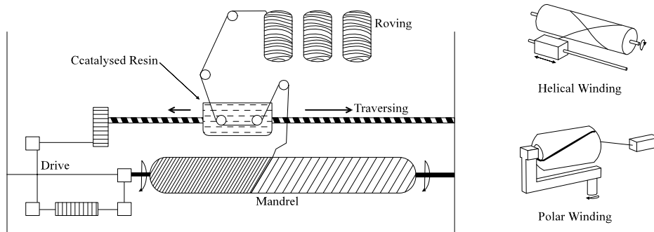
Figure 4.4-3. Typical filament winding process. 3
