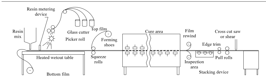
Figure 4.4-2. Typical continuous lamination production process. 2
