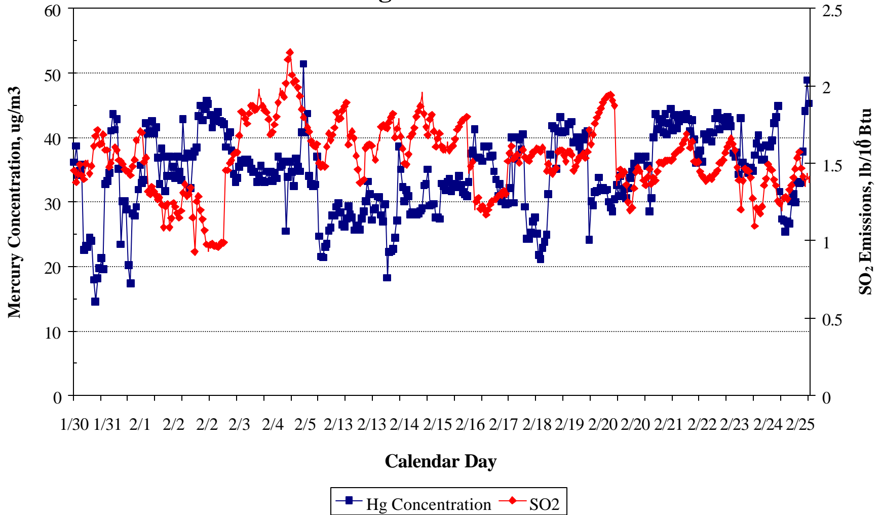
Figure 4. Fabric Filter Outlet Hg versus SO 2
