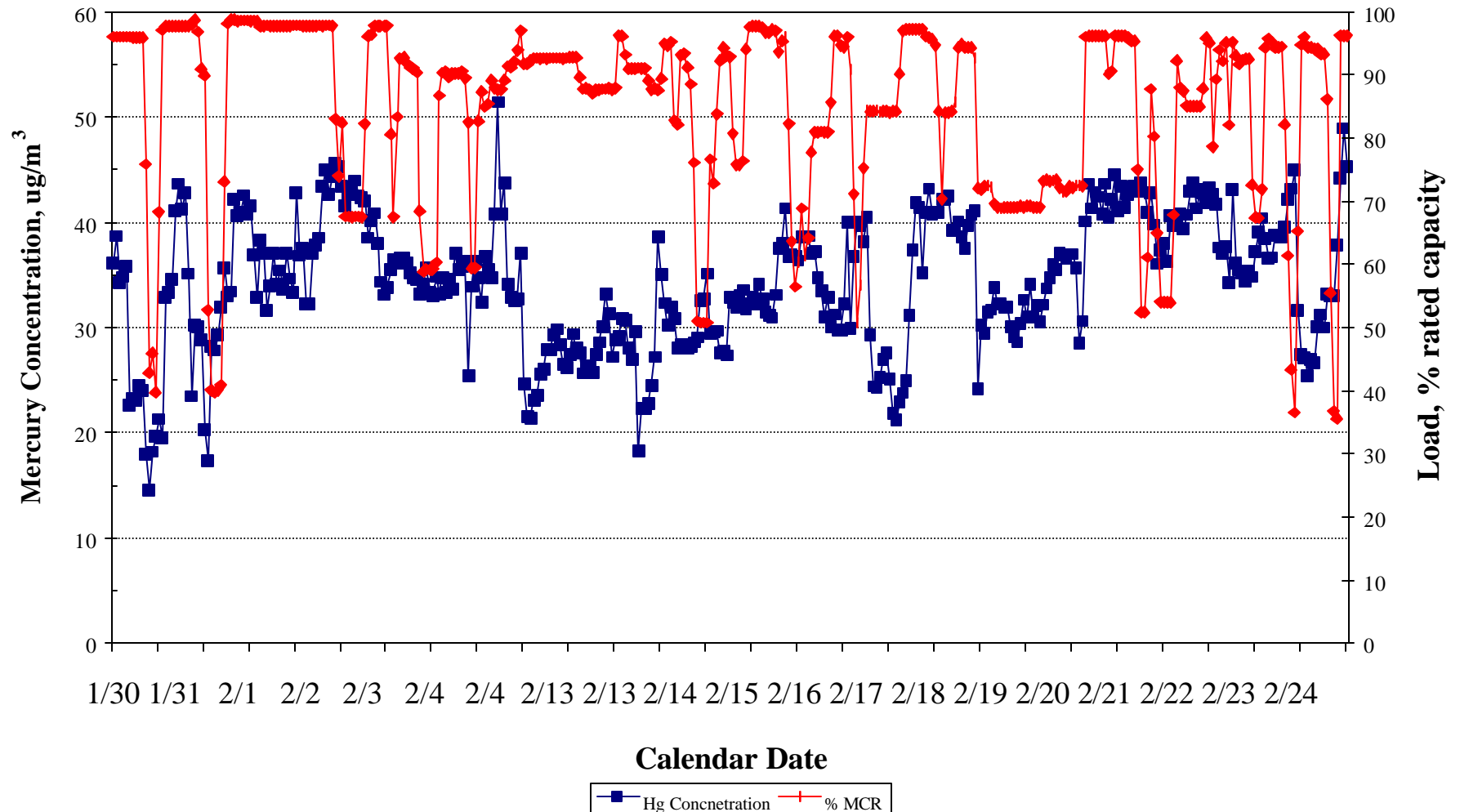
Figure 3. Fabric Filter Outlet Hg versus Load
