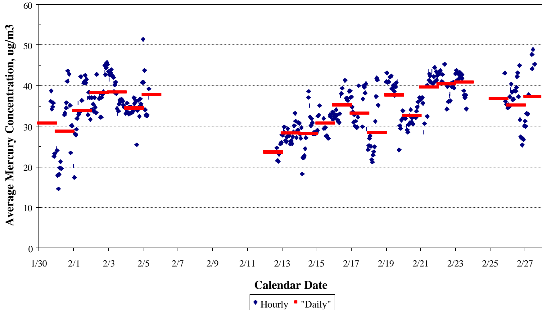
Figure 1. Fabric Filter Outlet Hourly versus Daily Averages
