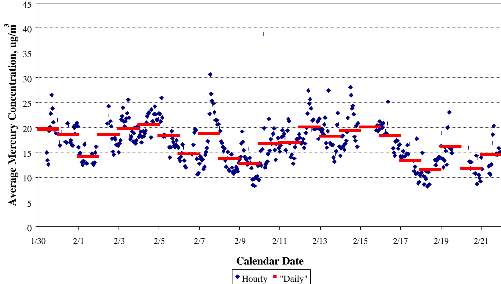
Figure 6. Coal-Fired Boiler: ESP Hourly versus Daily Averages
