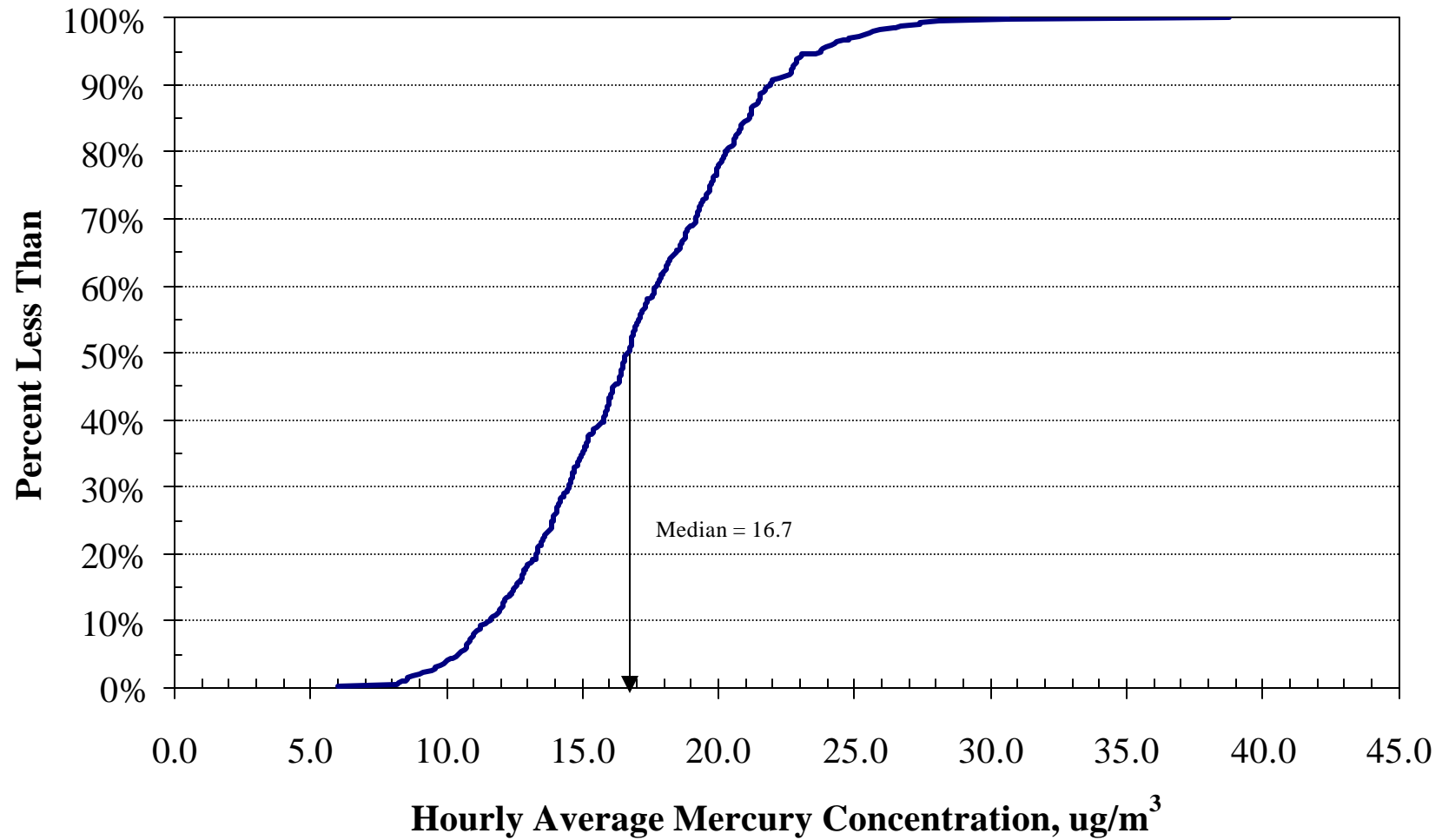
Figure 7. ESP Outlet Cumulative Distribution Frequency
