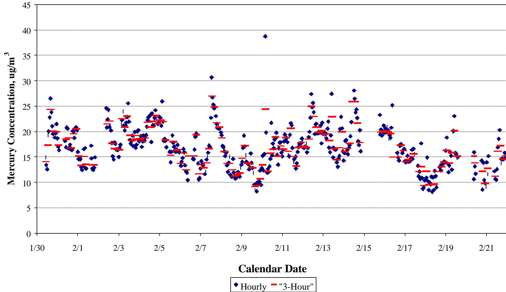
Figure 9. ESP Outlet Hourly versus 3-Hour Averages
