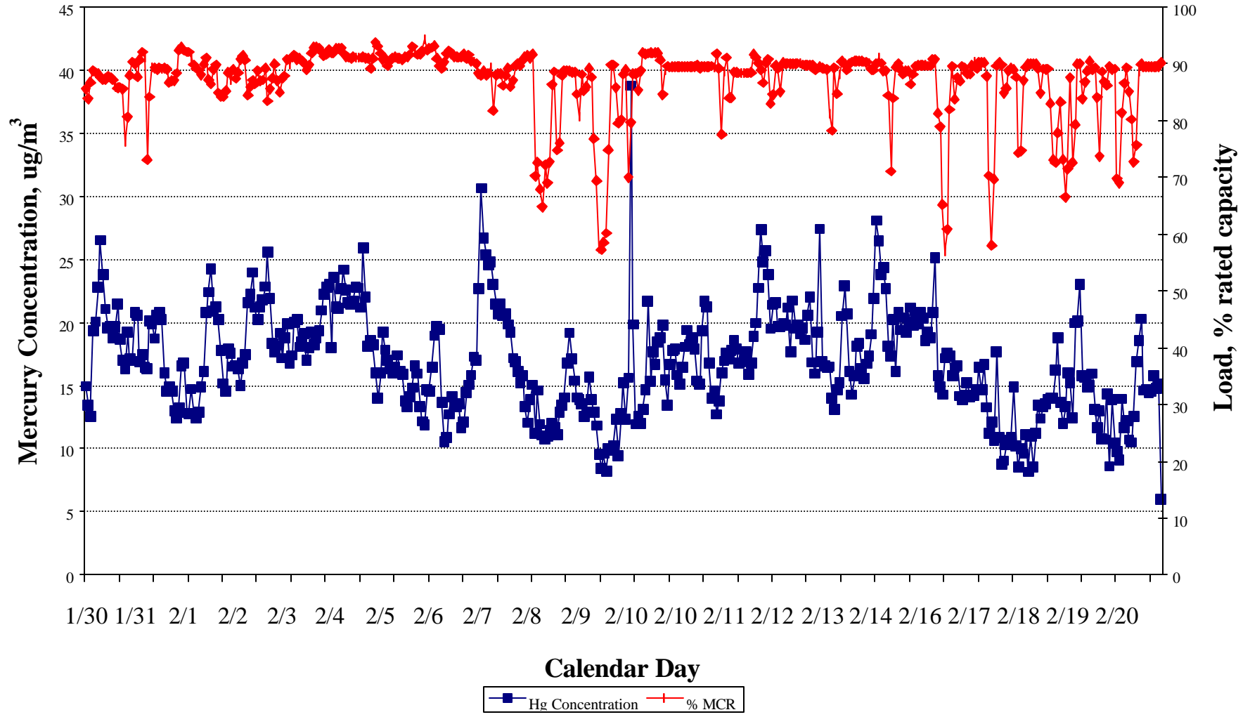
Figure 8. ESP Outlet Hg Versus Load
