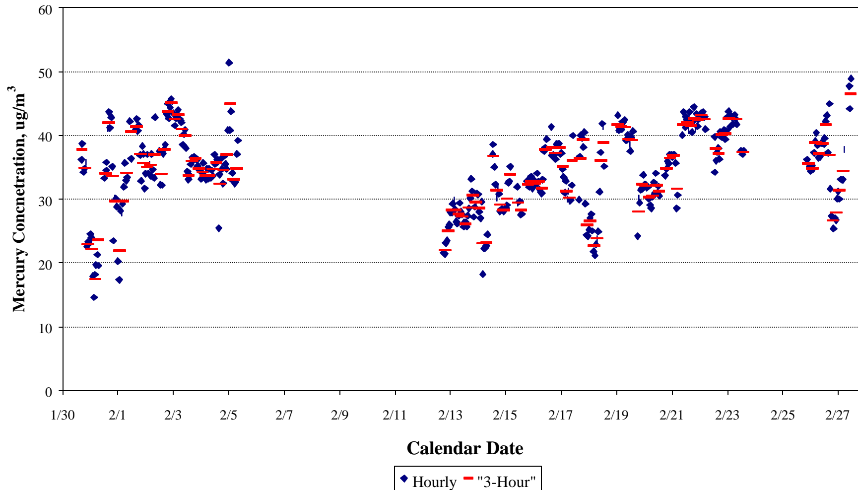
Figure 5. Fabric Filter Outlet Hourly versus 3-Hour Averages
