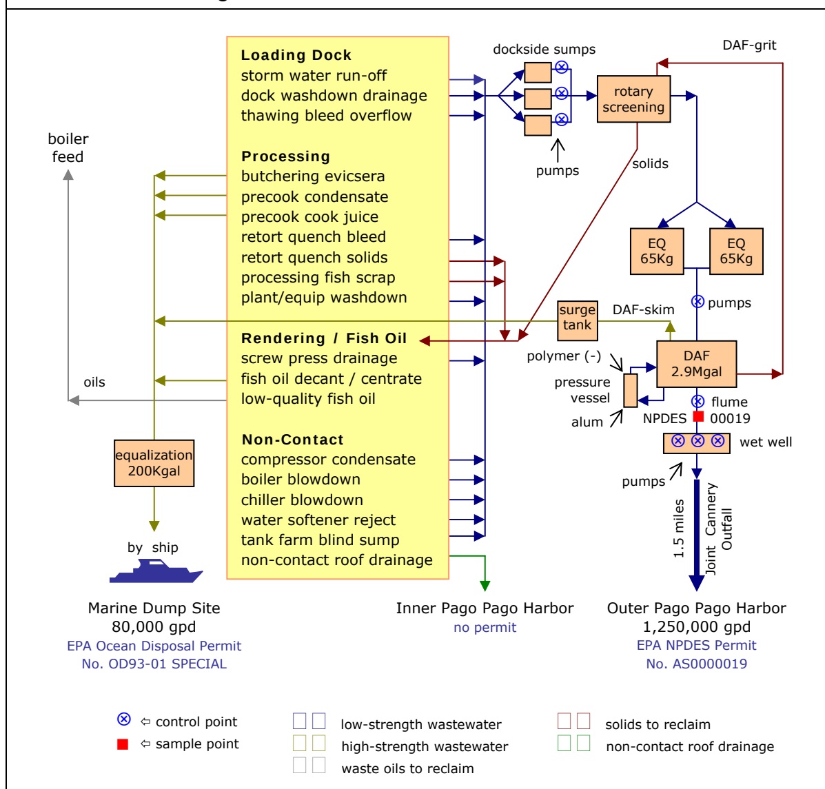
Figure 1.4 Starkist Samoa - Configuration
