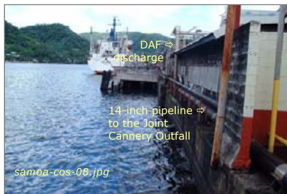
Photo #14: Joint Cannery Outfall Connection Taken By: Greg V. Arthur Date: 04/02/08
