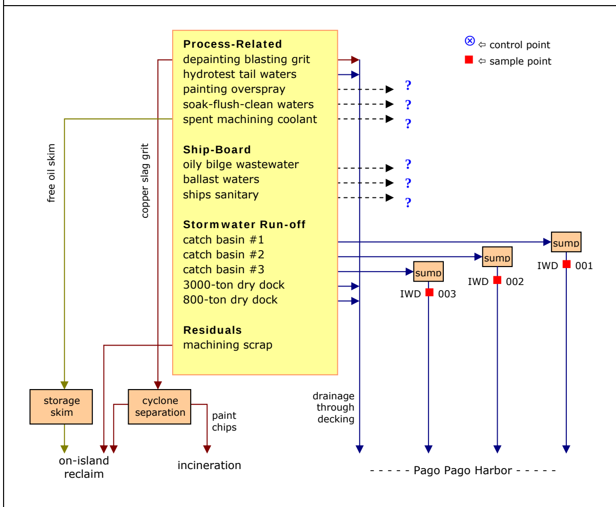
Figure 1.4.1 MYD Samoa Shipyard - Configuration
