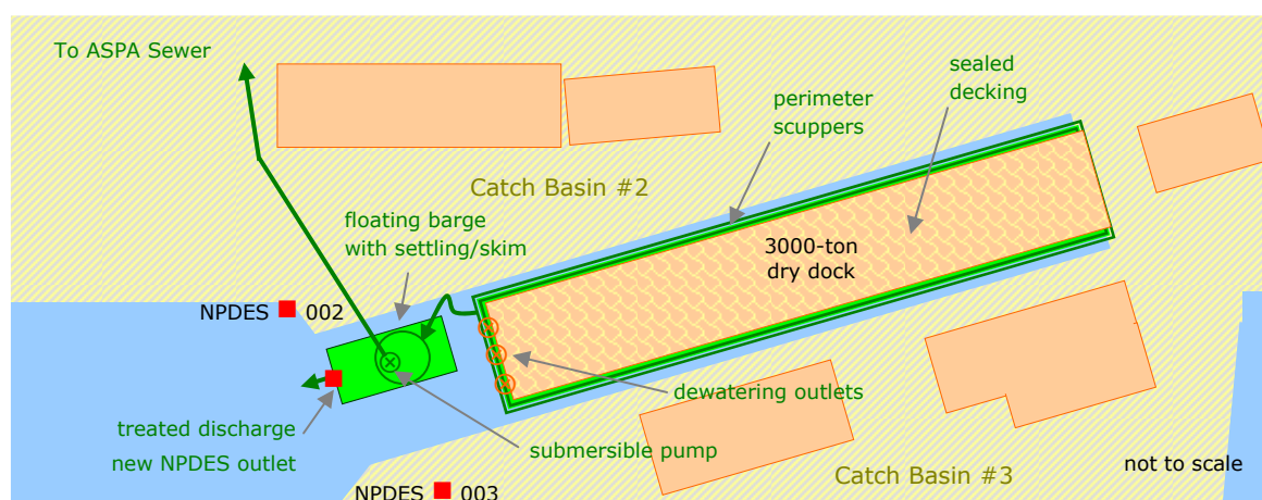
Figure 3.1.3 Schematic of Possible Upgrades - Option 2 Floating Barge Treatment
