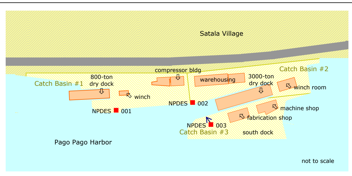
Figure 1.4.2 MYD Samoa Shipyard - Layout
