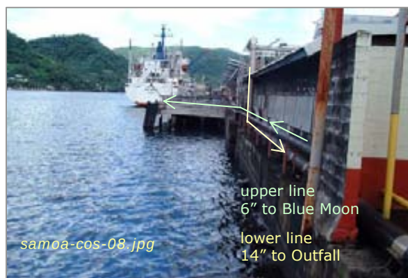
Photo #4: Outfall and High-Strength Lines Taken By: Greg V. Arthur Date: 04/02/08
