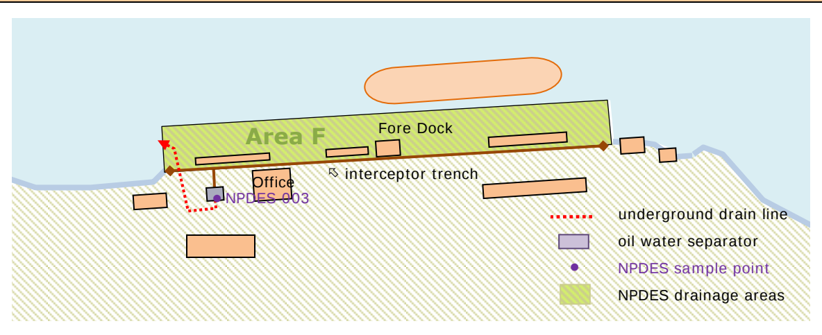
Figure 1.2.2 American Samoa Terminal, Fuel Dock – Layout
