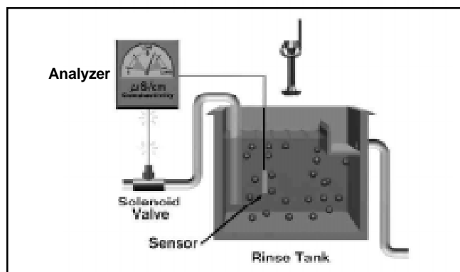
Figure 1. Conductivity Control System Components
