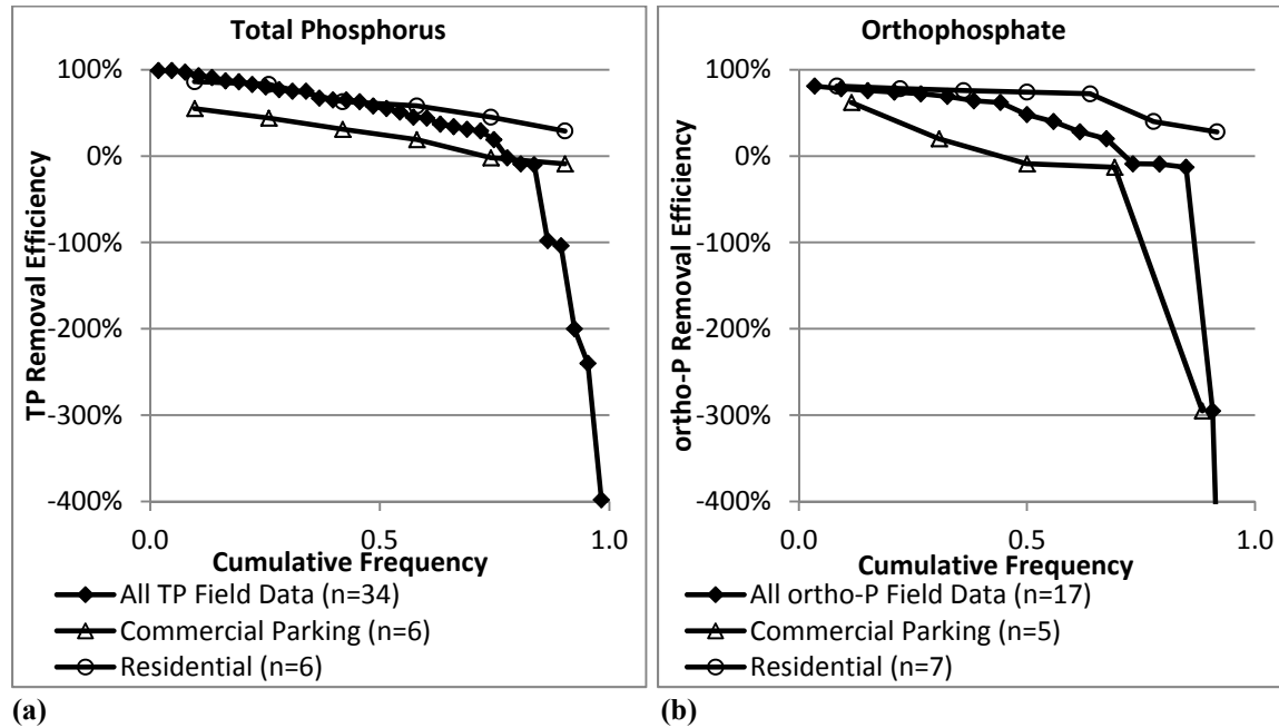
Figure 6. Cumulative Frequency Functions of Total Phosphorus and Orthophosphate Removal Efficiencies in the SPU Bioretention Database.
