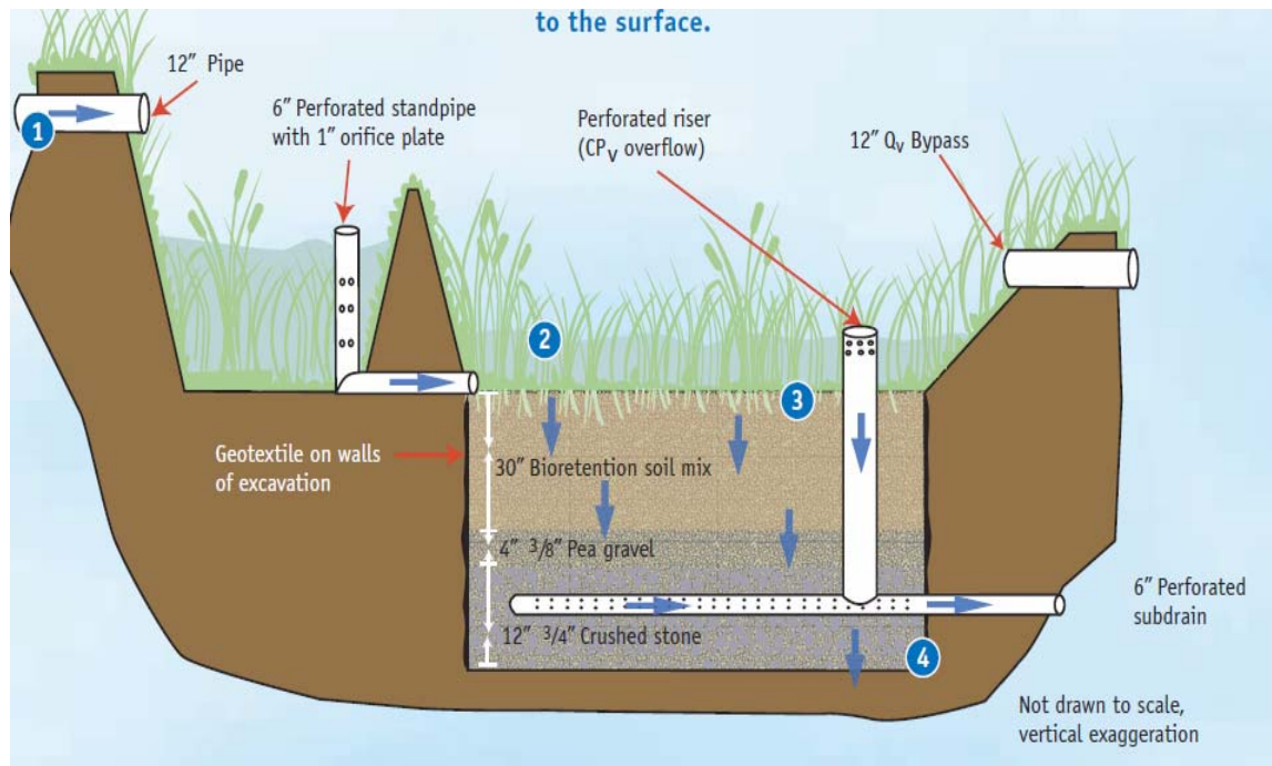
Figure 1. Bioretention Schematic
