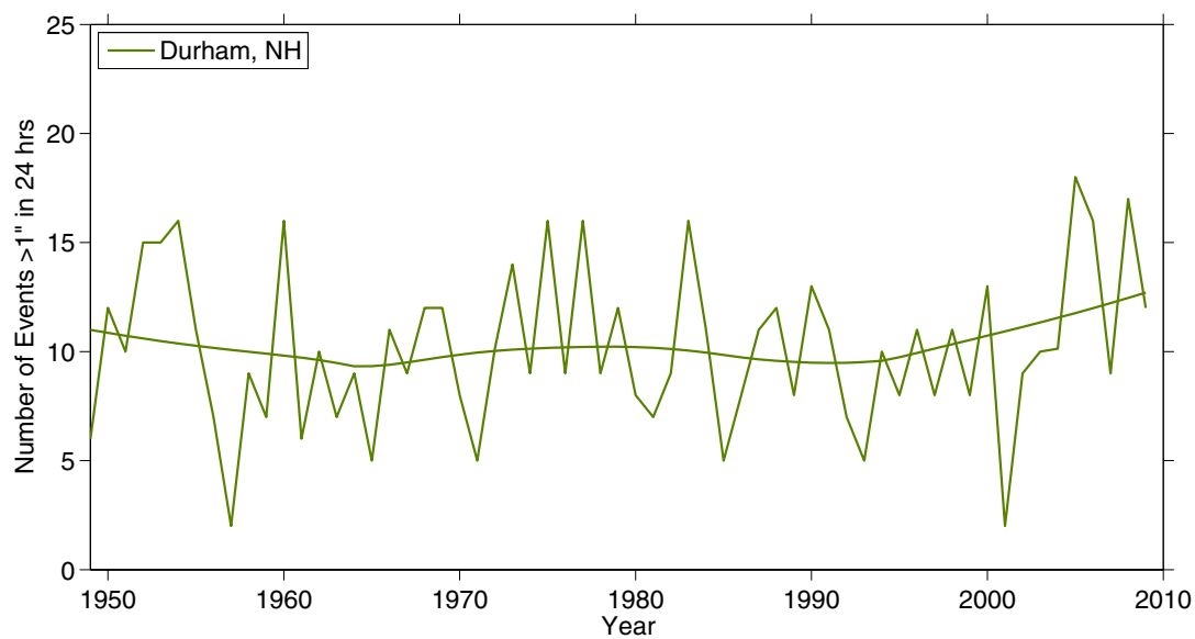
Figure 6. Number of events per year with greater than one inch of precipitation in 24 hours for Portland (top), Lawrence (middle), and Durham (bottom).
