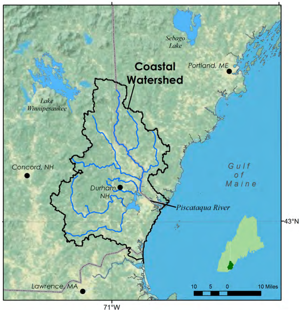
Figure 2. Map of the Piscataqua region and Great Bay watershed showing the location of United States Historical Climate Network stations (Durham, NH, Lawrence, MA, and Portland, ME) and Global Historical Climate Network stations (Concord, NH) (black dots). These stations provide historical climate data within and around the Great Bay watershed over the time period 1895-2009.
