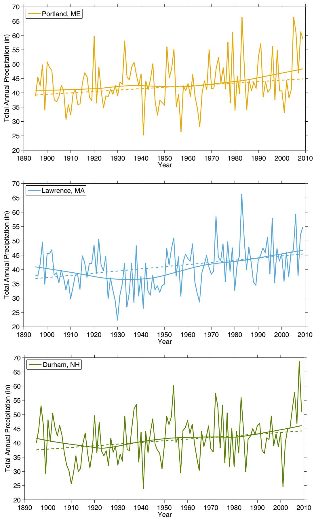
Figure 5. Annual precipitation for Portland (top), Lawrence (middle), and Durham (bottom) showing Sen's slope (dashed) and LOWESS smooths (solid), 1895-2009.
