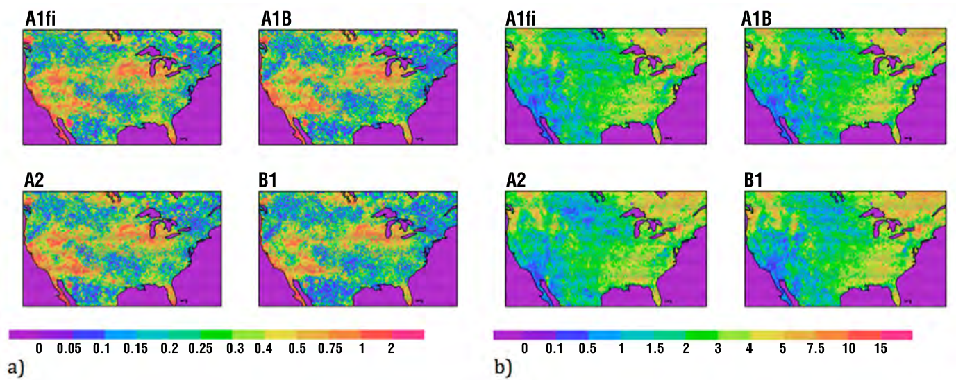
Figure B1. The bias in (a) the 99th quantile of the distribution of maximum temperature as simulated by downscaling GFDL CM2.1, and (b) the number of wet days per year ( pr > 0.1 ) in downscaled simulations compared to observations for the period 1960-2000, as simulated by downscaling HadCM3.
