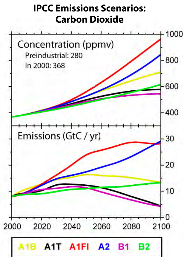
Figure 14. Projected future concentrations (top) and emissions (bottom) of carbon dioxide, 2000-2100. [Image by Robert A. Rohde/Global Warming Art.]
