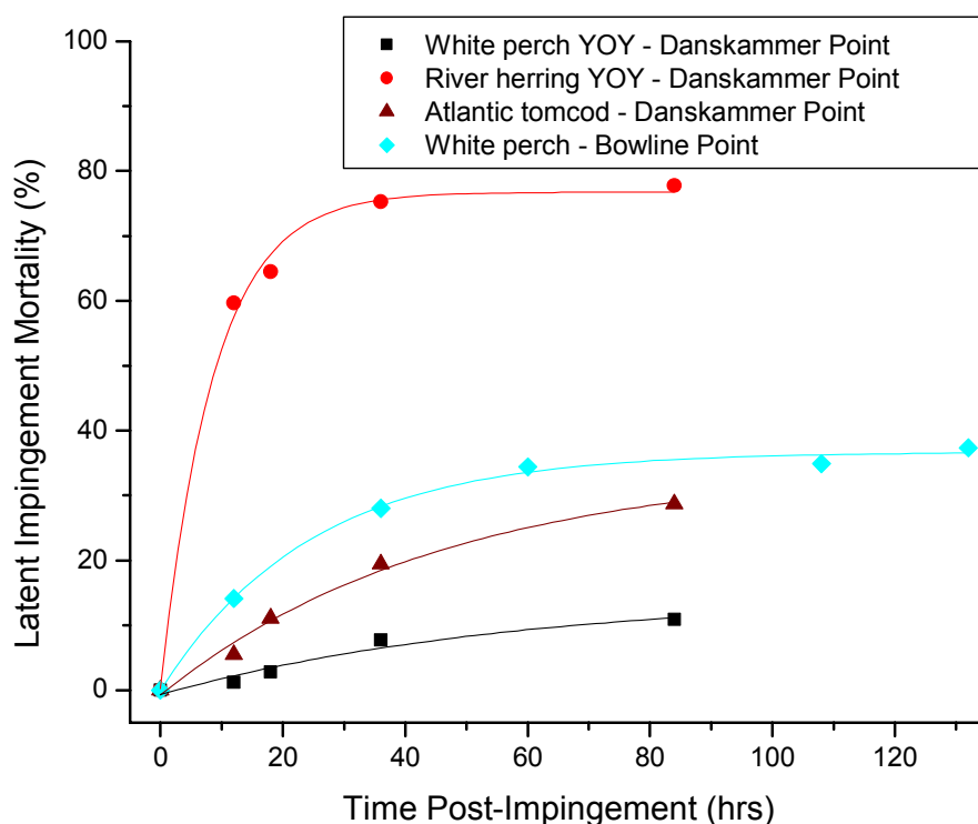
Figure 2-4 Control-adjusted mortality versus holding time for several species impinged at the Danskammer Point and Bowline Point Generating Stations (data from EA 1979a, EA 1982)
