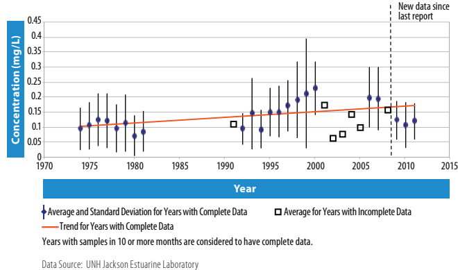
FIGURE 3.2 Dissolved inorganic nitrogen concentration trends at Adams Point in the Great Bay Estuary
