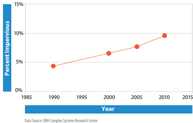
FIGURE 1.1 Percent of land area covered by impervious surfaces in the Piscataqua Region watershed, 1990-2010
