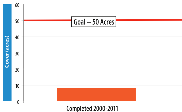
FIGURE 19.1 Cumulative acres of eelgrass restoration 2000-2011
