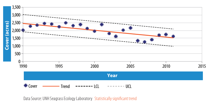
FIGURE 6.2 Eelgrass cover in Great Bay proper
