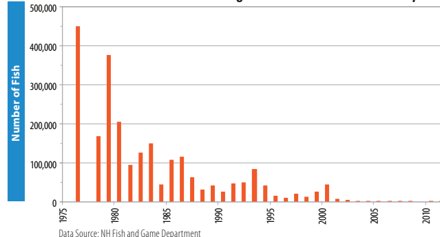
FIGURE 14.2 Returns of river herring to the fish ladder on the Taylor River
