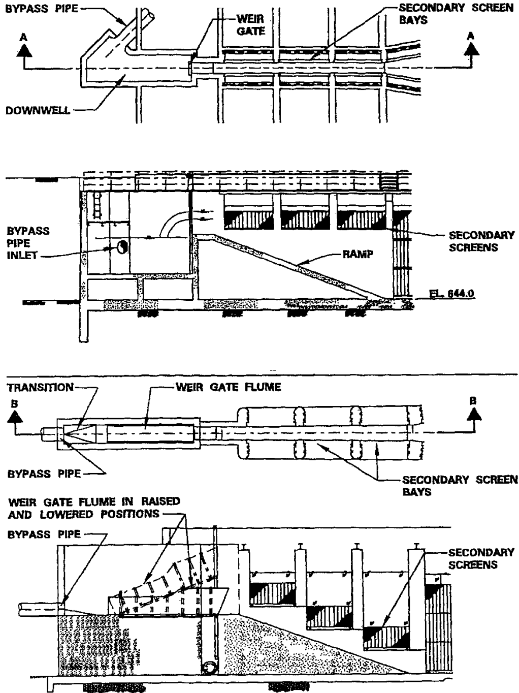
Figure 10-6 White River screen system — section view (Dorratcague et al. 1996)
