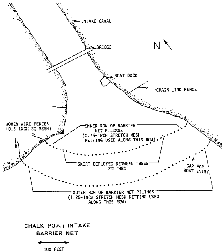
Figure 6-4 Chalk Point barrier net configuration (Loos 1986a, b)
