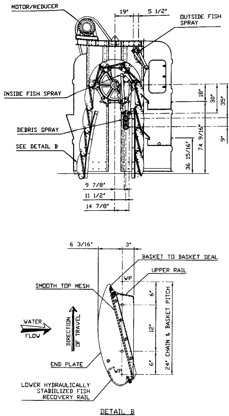
Figure 2-6 Modified dual-flow screen at Dunkirk Station (Beak 1988)
