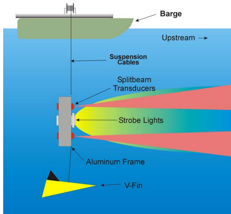
Figure 13-5 Deployment of strobe lights and hydroacoustic transducers from fixed barge (Simmons et al. 2002)
