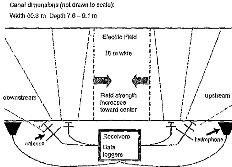
Figure 17-5 Arrangement of antennas and hydrophones at the barrier (Sparks et al. 2010)
