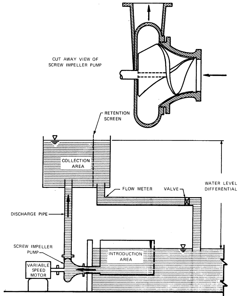
Figure 9-9 Hidrostral pump test facility (ESEERCO 1981b)
