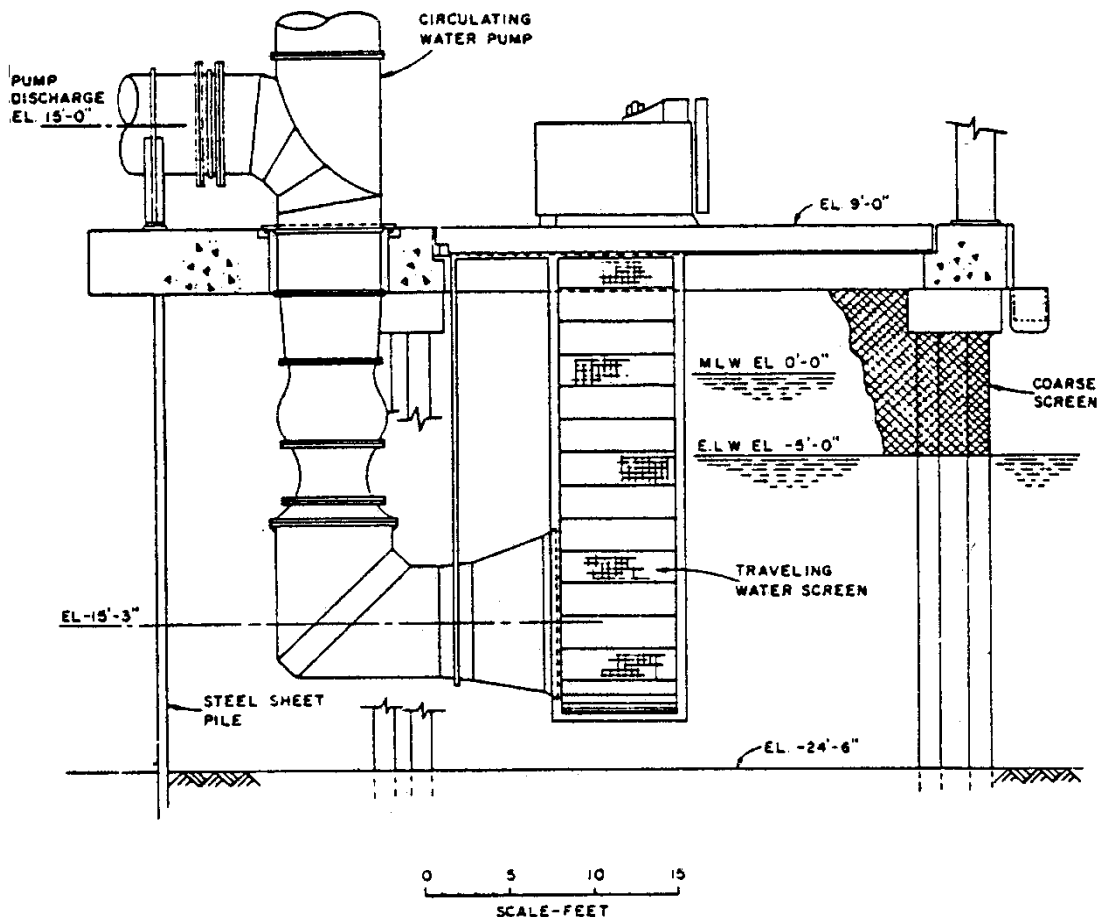
Figure 2-13 No-well screen (SWEC 1980)
