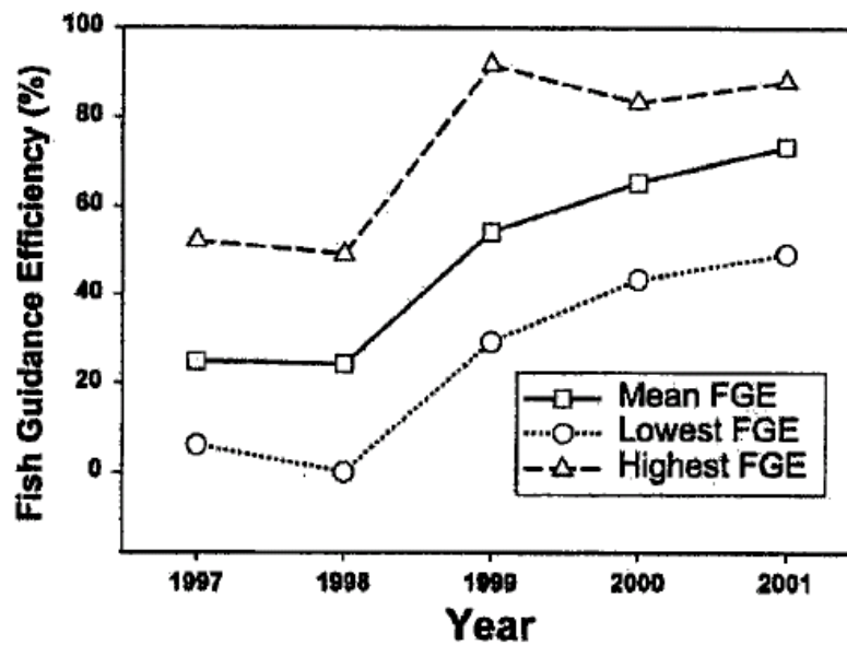
Figure 12-5 Fish guidance efficiencies (unadjusted) for Atlantic salmon smolts for the 5 years of monitoring, 1997 to 2001 (Scruton et al. 2003)
