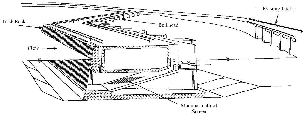
Figure 11-3 Schematic of modular inclined screens (Taft et al 1997)
