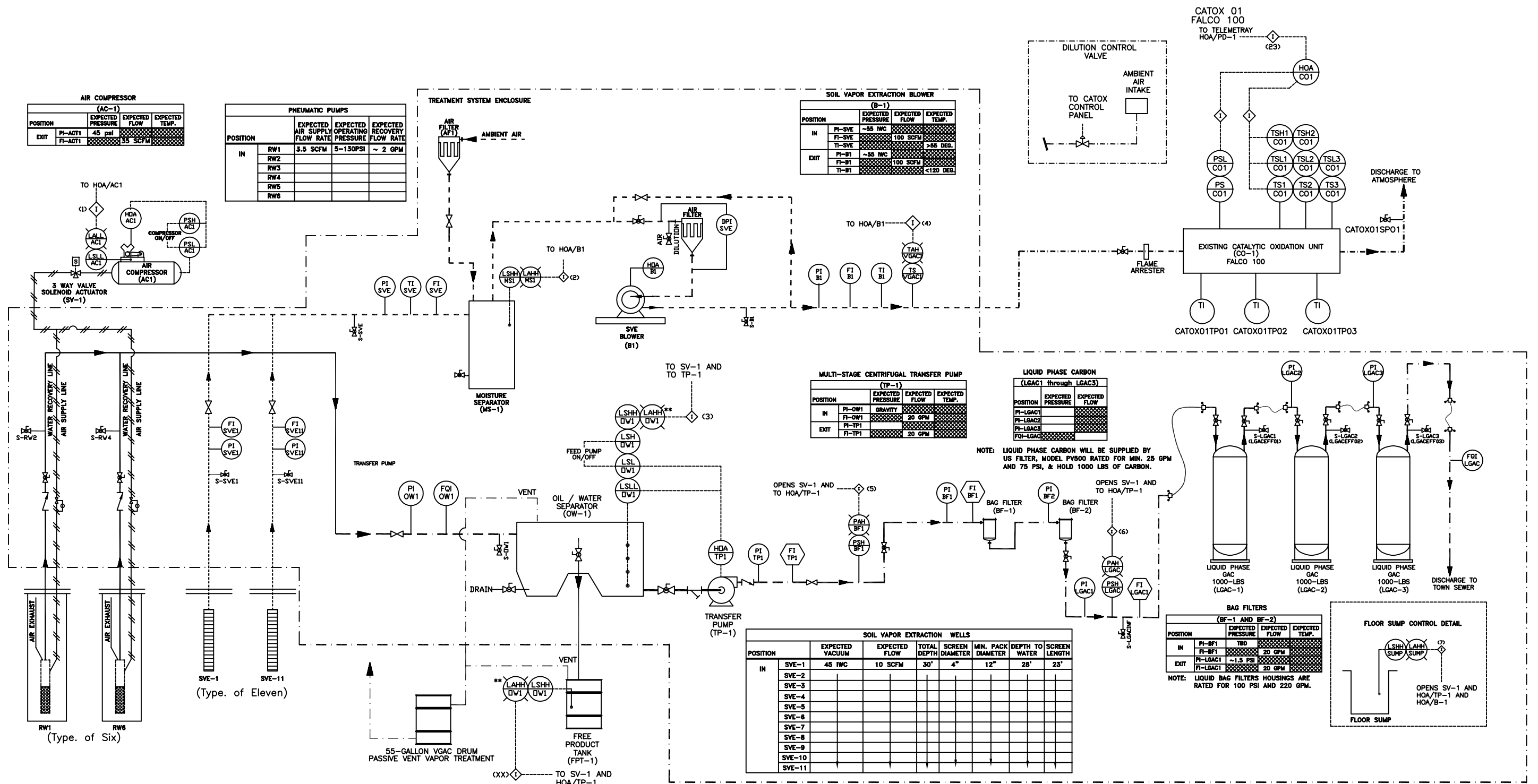
FIGURE 15 SVE/GWE SYSTEM PROCESS & INSTRUMENTATION JEMS NEW ENGLAND 682 MAIN STREET CLINTON, MASSACHUSETTS
