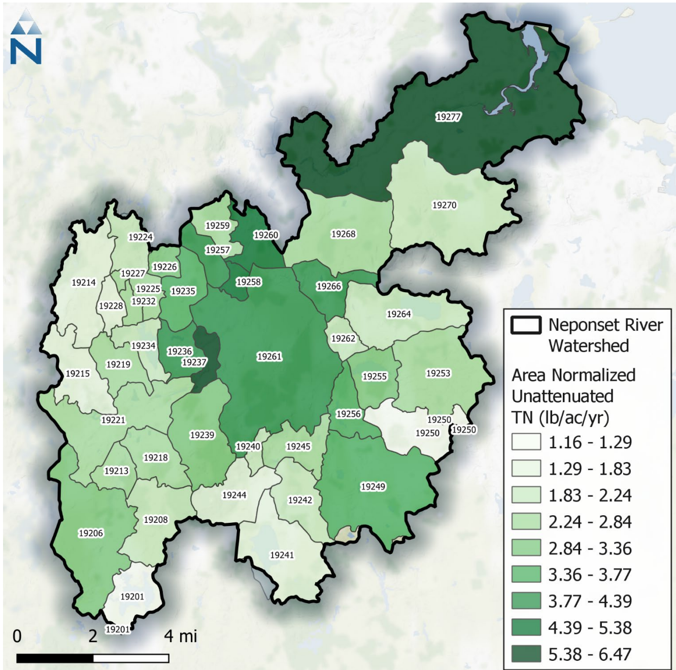
Figure 3-19. Area normalized annual average (1992-2022) total TN load by subbasin.
