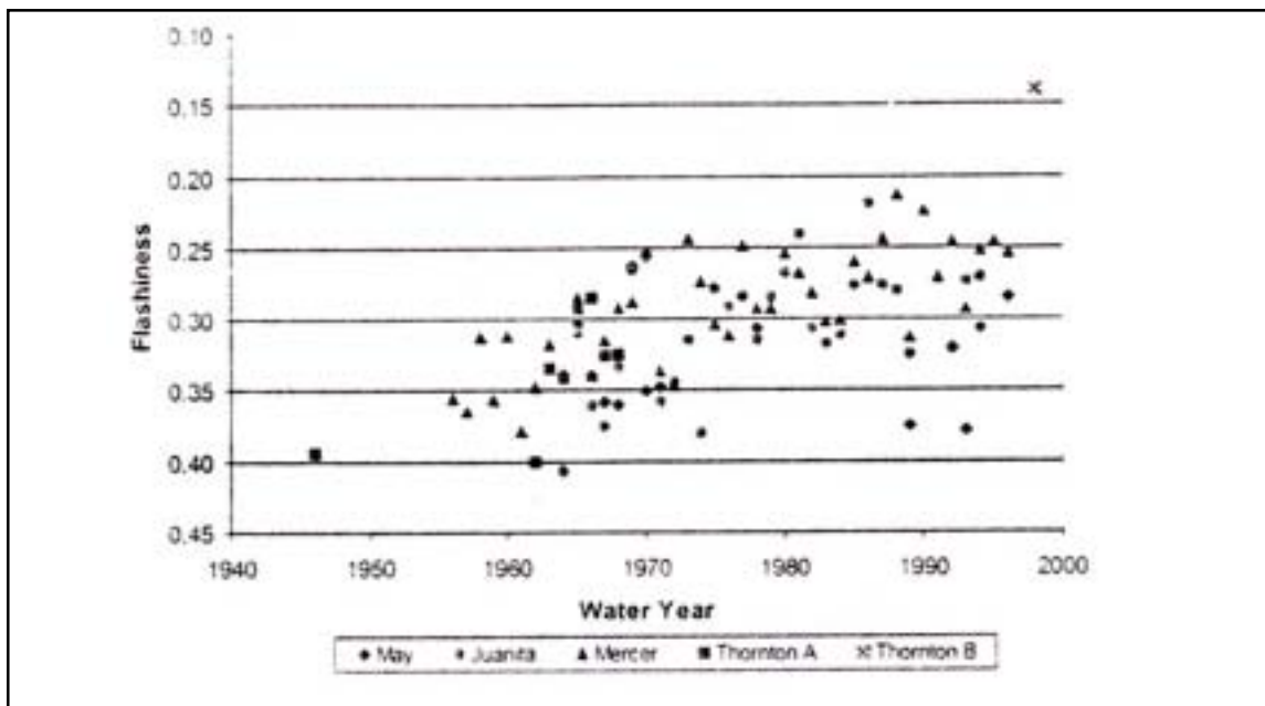
Figure 13: Percent of Gage Reading Above Mean Annual Flow for Puget Sound Lowland Streams (Henshaw and Booth, 2000)
