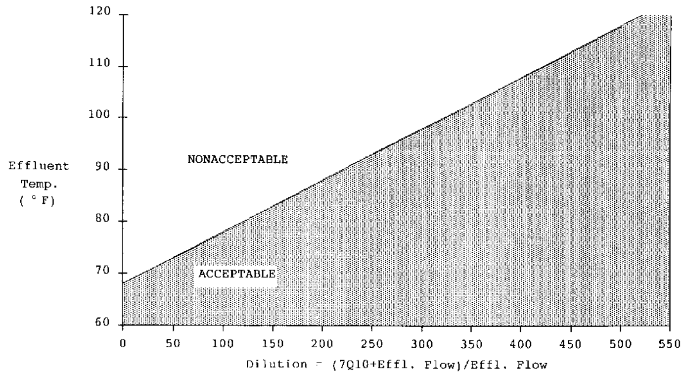
Effluent Temperature Dilution Graph
