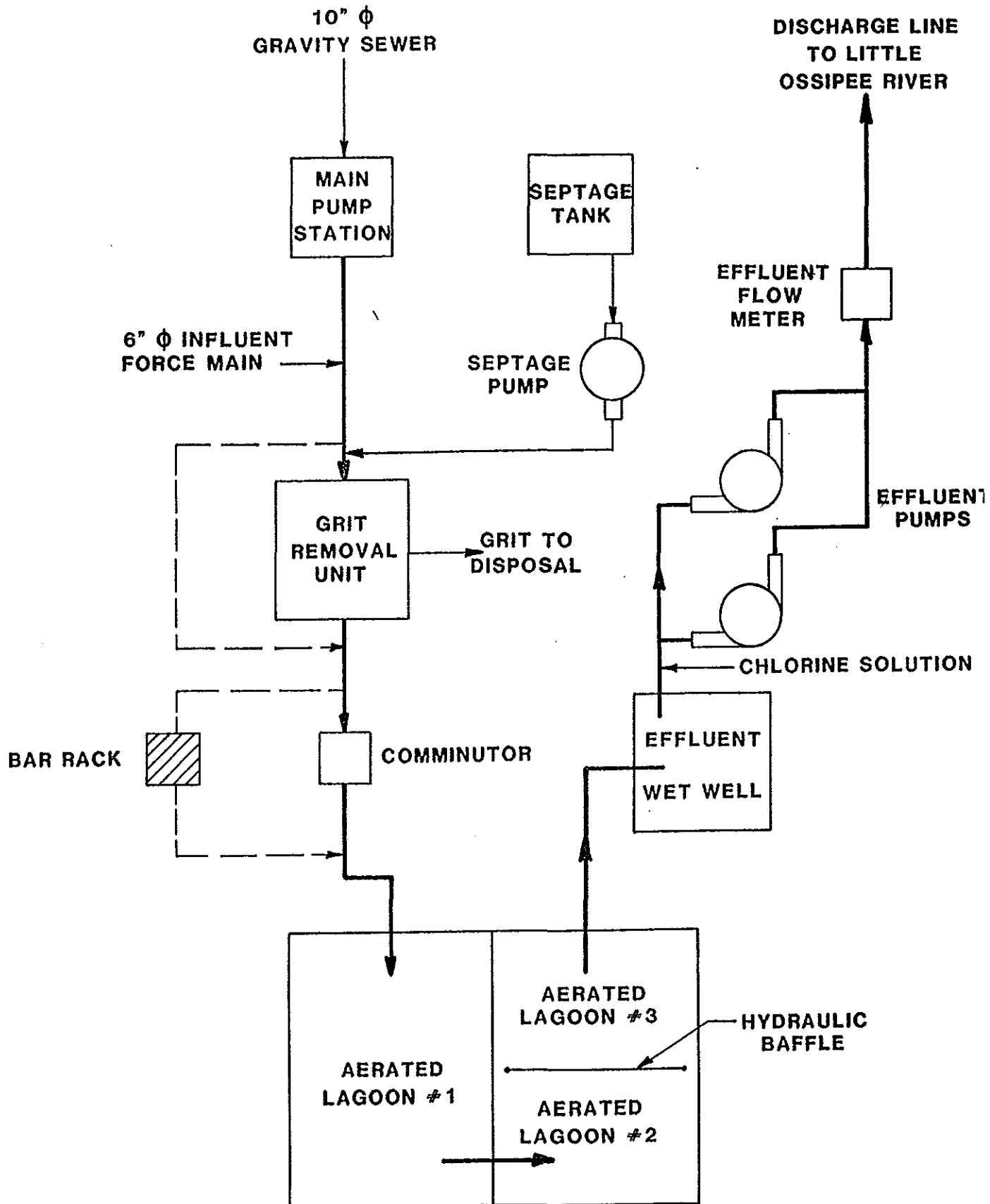
LIMERICK SEWERAGE DISTRICT PLANT FLOW SCHEMATIC
