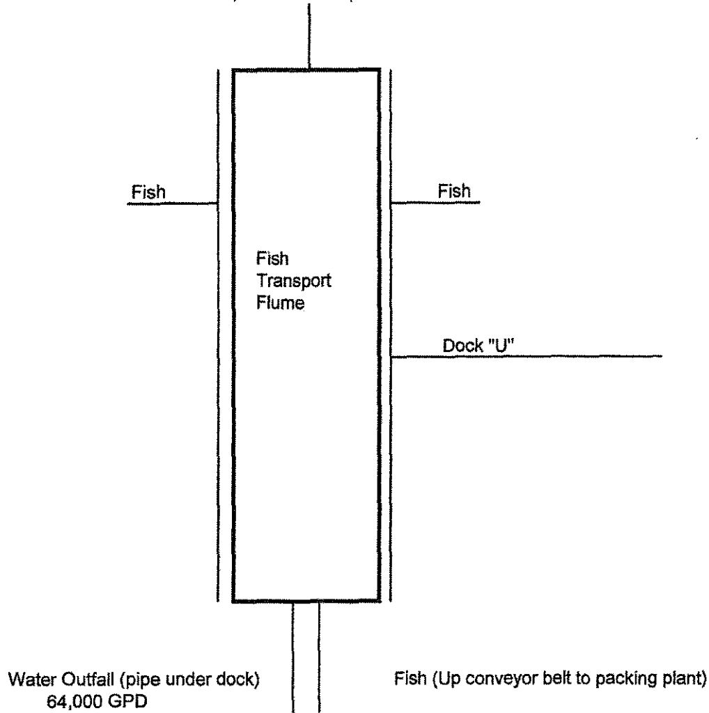
Schematic of Water Flow 001 Seafreeze Shoreside Narragansett, Washington County, RI
