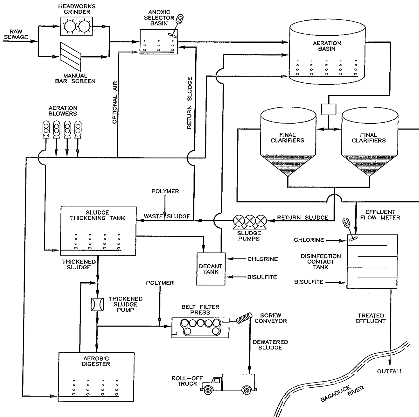
CASTINE POLLUTION CONTROL FACILITY PROCESS FLOW SCHEMATIC
