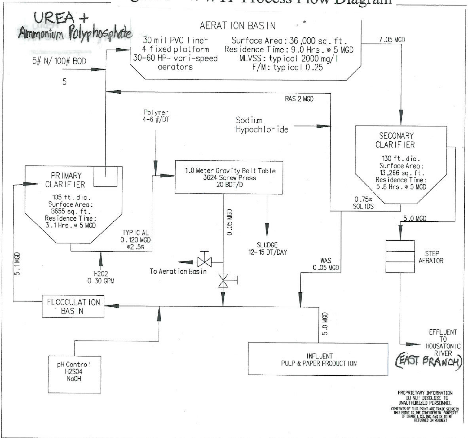
Figure 3 - WWTP Process Flow Diagram
