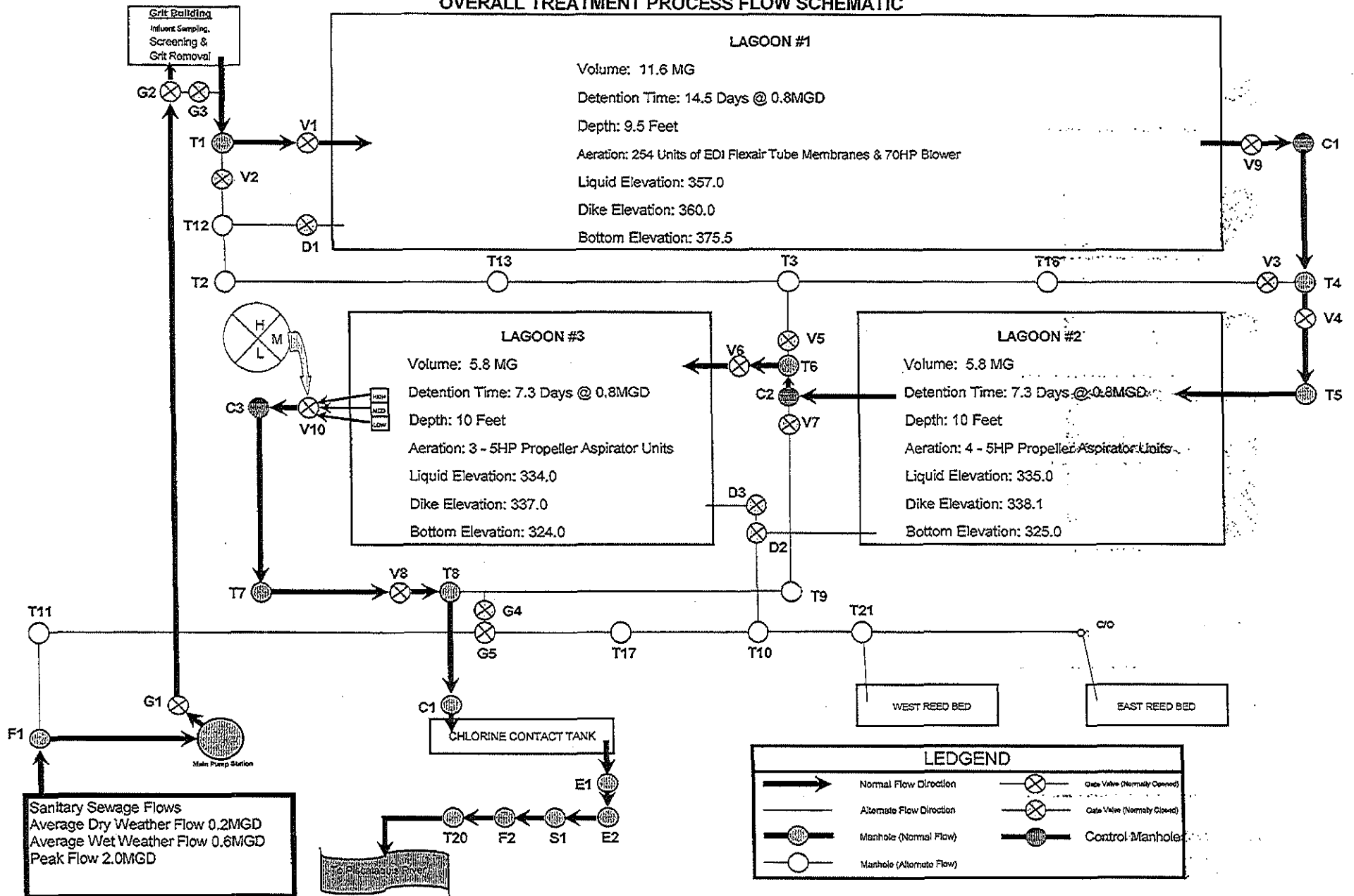
FIGURE 1-1 OVERALL TREATMENT PROCESS FLOW SCHEMATIC
