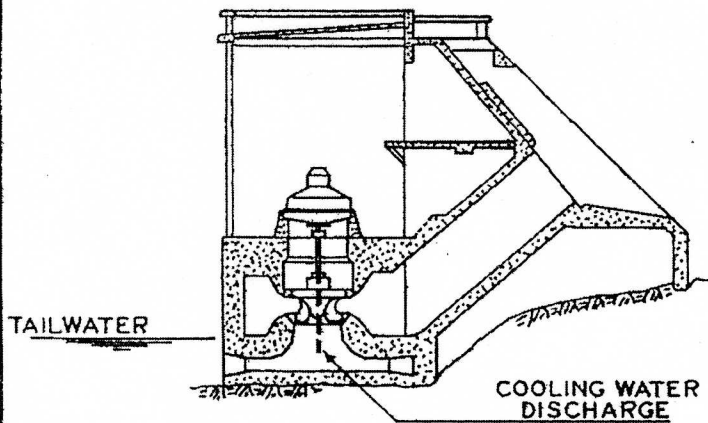
SECTION THRU POWERHOUSE
