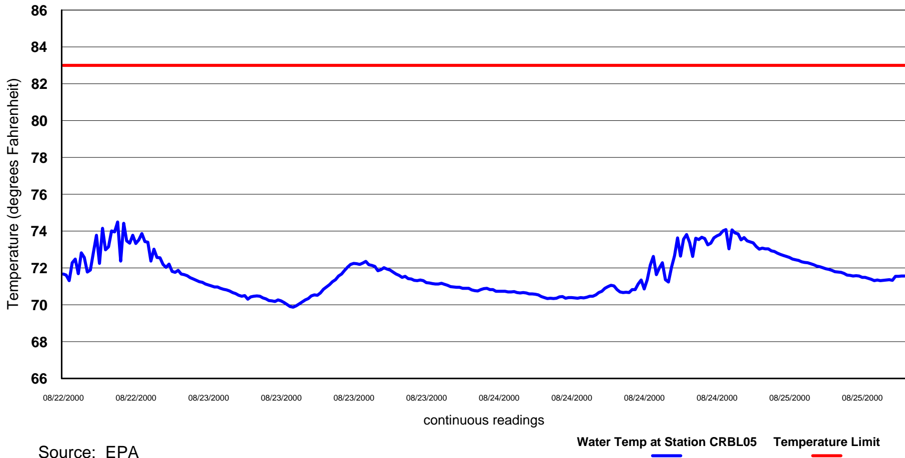
Figure 5.9.2-34 Charles River ambient river temperatures, recorded continuously at a depth of 0.75 meters, in the vicinity of the Boston University Bridge (background monitoring station), compared with the established temperature limit for the Zone of Passage and Habitat (August 22 - 25, 2000).
