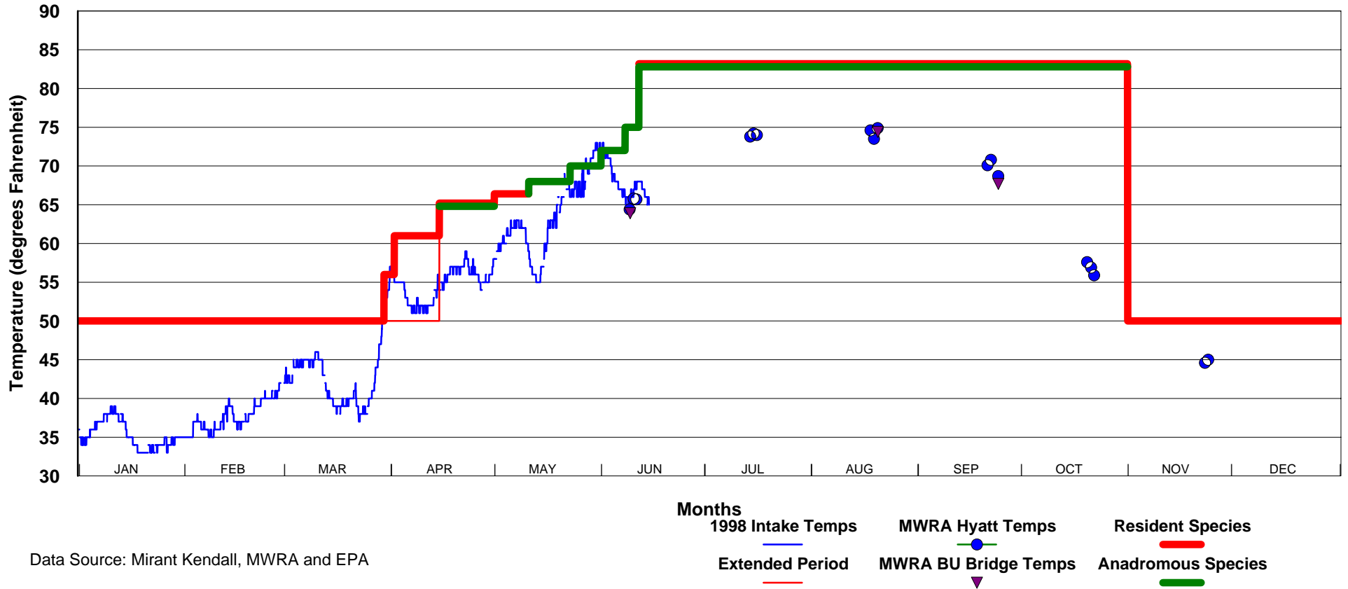
Figure 5.9.2-19 Kendall Station cooling water intake continuous temperatures and discrete MWRA temperature data, judged to approximate ambient lower Charles River Basin conditions, compared with temperature limits established for the Zone of Passage and Habitat (January - December 1998).
