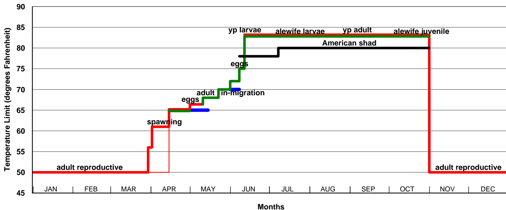
Figure 5.8.1-1 Protective temperature limits and time periods for the most sensitive resident species and the most sensitive anadromous species, organized by month. When two different temperature limits were identified for the same time period, the lowest protective temperature was used as the limit, for as long as it applied. The life stages being protected are also identified. Additional protective temperatures in effect at Station 8 are included. American shad protective temperature values are included for information only at this time.
