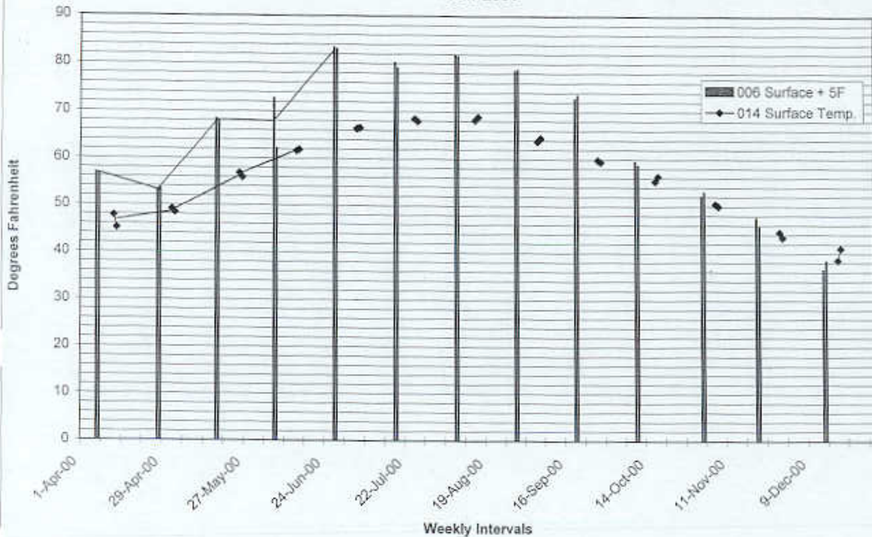
Figure 5.8.2g-7 Charles River, MWRA Station 006 Surface (0.3m) Temperature +5F and MWRA Station 014 (Boston Harbor) Surface (0.3m) Temperature Year 2000
