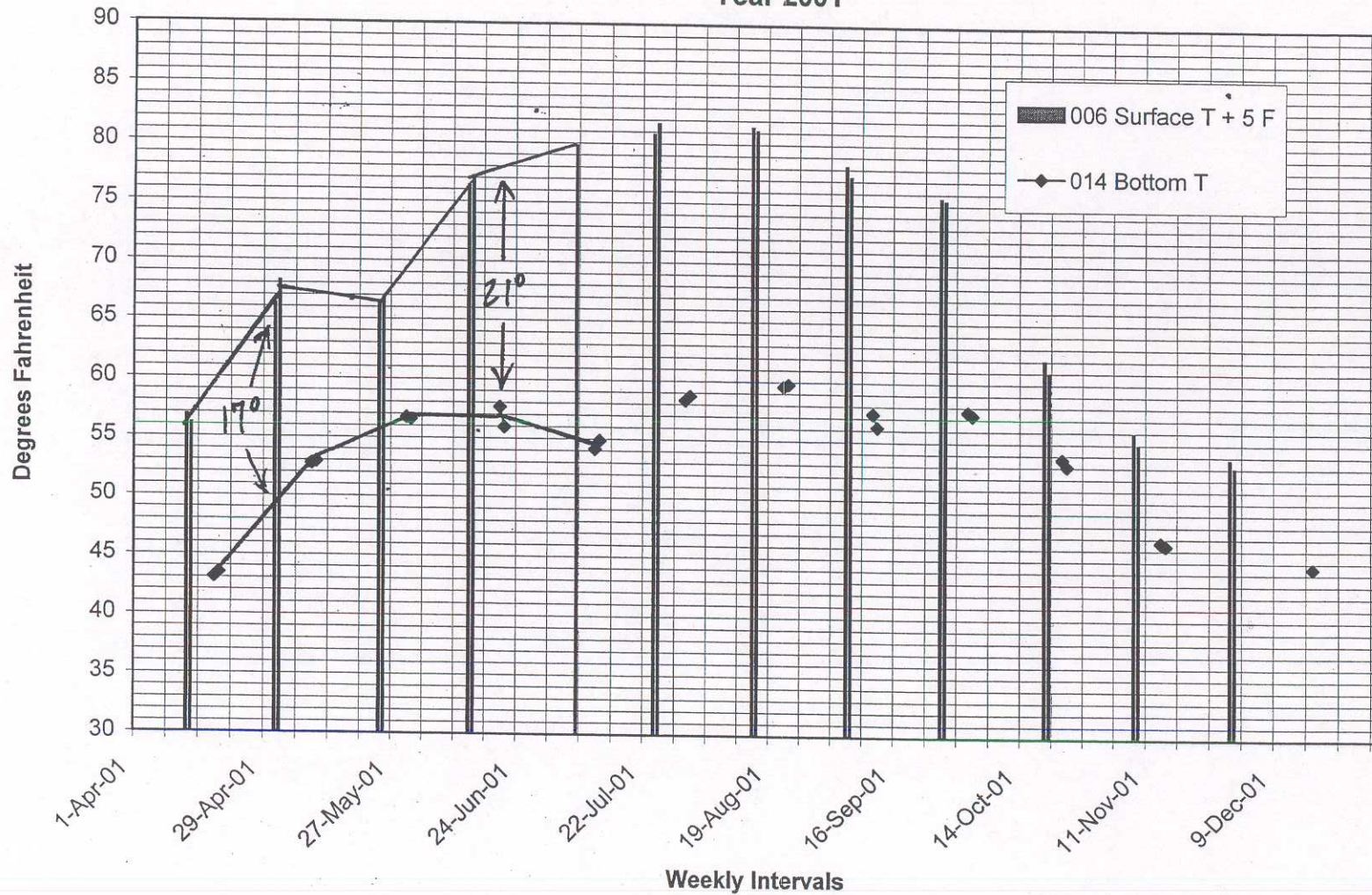
Figure 5.8.2g-5 Charles River, MWRA Station 006 Surface Temperature + 5 F and MWRA Station 014 Bottom Temperature Year 2001
