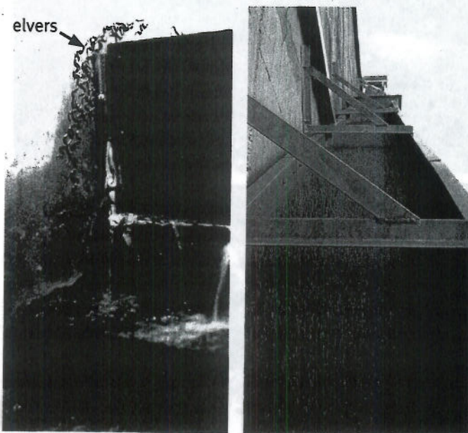
Eels have the ability to ascend damp vertical surfaces (left), but passage is far more successful if we provide ramps with climbing substrate, like this one on Mallemort Dam in France (right). Alex Haro
