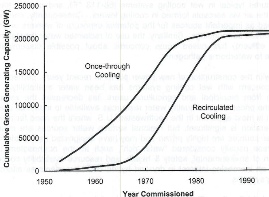
Figure 1 Growth of Once-through and Recirculated Cooling 1
