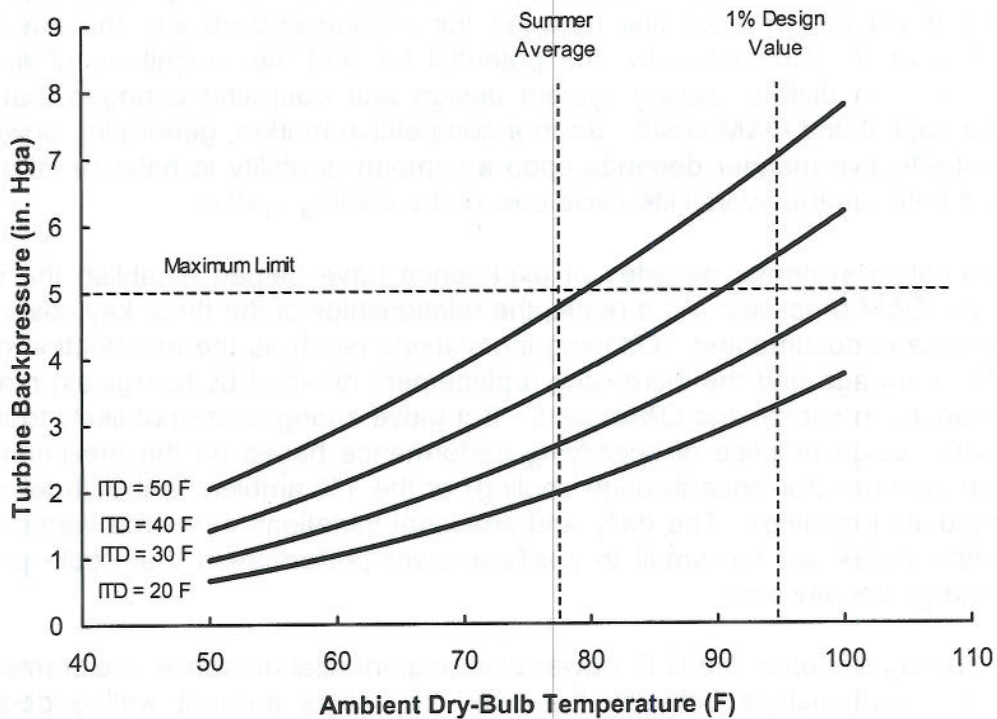
Figure 2 Ambient Dry-Bulb Temperature vs Turbine Backpressure
