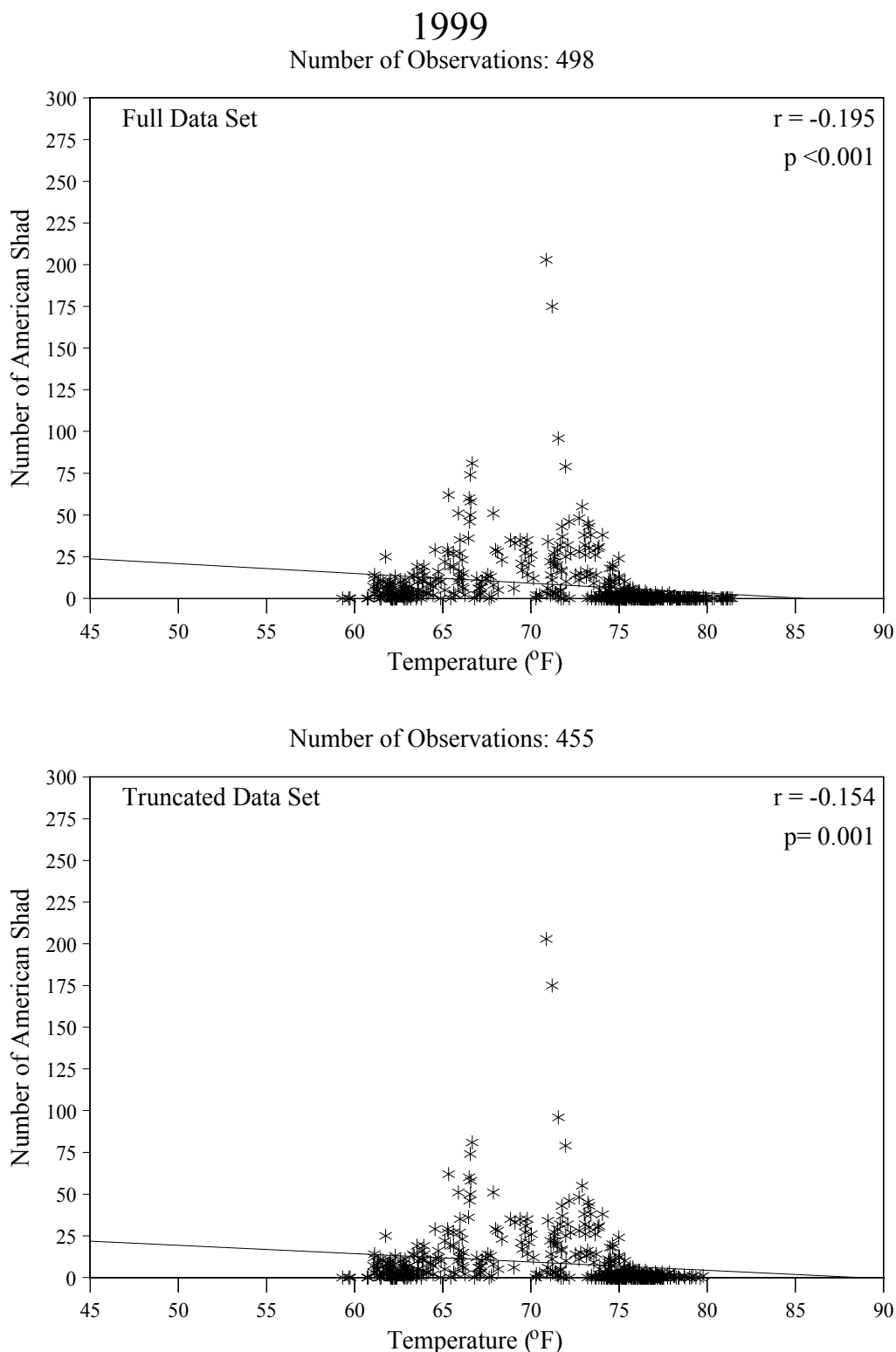
Figure 5-21. Scatter plots, Pearson product-moment correlation coefficient ( r ), and significance probability value ( p ) for the relationship between hourly average temperature ( ^{\circ}\text{F} ) and the corresponding number of adult American shad passing upstream through the Vernon fishway on the Connecticut River, Vernon, Vermont, May-July 1999.
