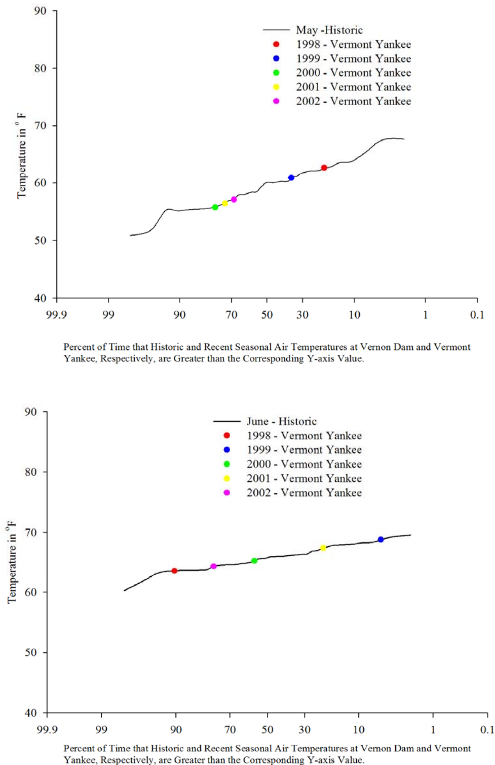
Figure 3-5a. Historic Average (May 16 – 31) and June Air Temperature Duration Curve at Vernon Dam.
