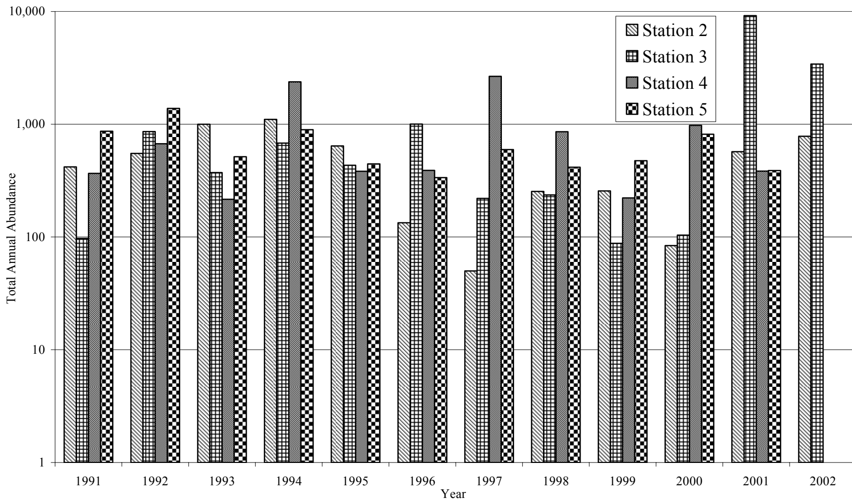
Figure 5-3. Total number of macroinvertebrates collected in rock baskets placed in the Connecticut River upstream and downstream of Vernon Dam, 1991 through 2002. Rock Basket sampling at Stations 4 and 5 was discontinued in 2002. Note the use of a log scale on the Y axis.
