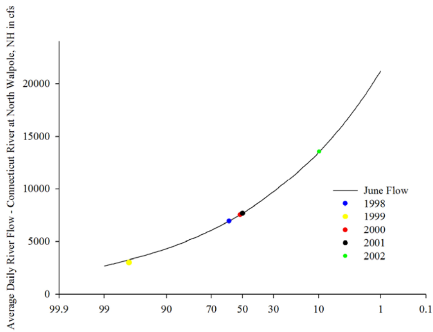
Figure 3-2a. Historic Flow Duration Curve for the Connecticut River at North Walpole, NH – May (16-31) and June.
