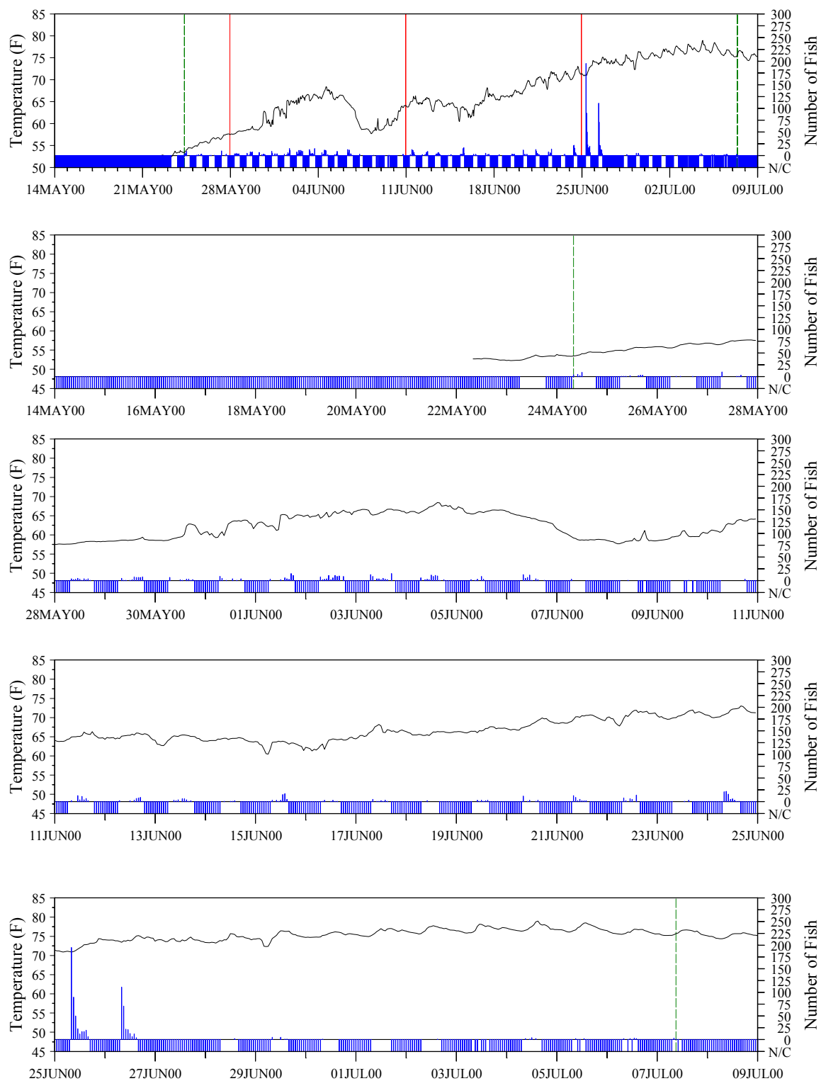
Appendix Figure 6-10. Hourly count of adult American shad passing upstream through the Vernon Dam Fishway on the Connecticut River, Vernon, Vermont and the corresponding hourly average fishway water temperature, 14 May – 9 July, 2000.
