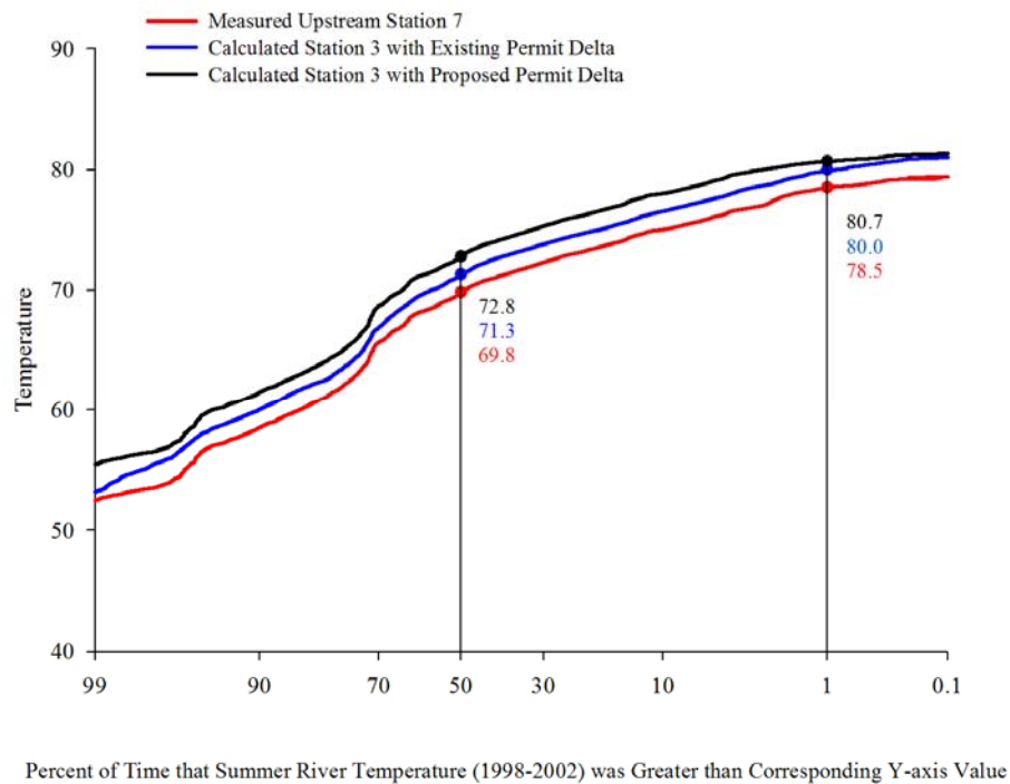
Figure 3-10. Comparison of Projected Temperature Response in the Connecticut River for Background, Existing and Proposed Vermont Yankee Discharge Conditions.
