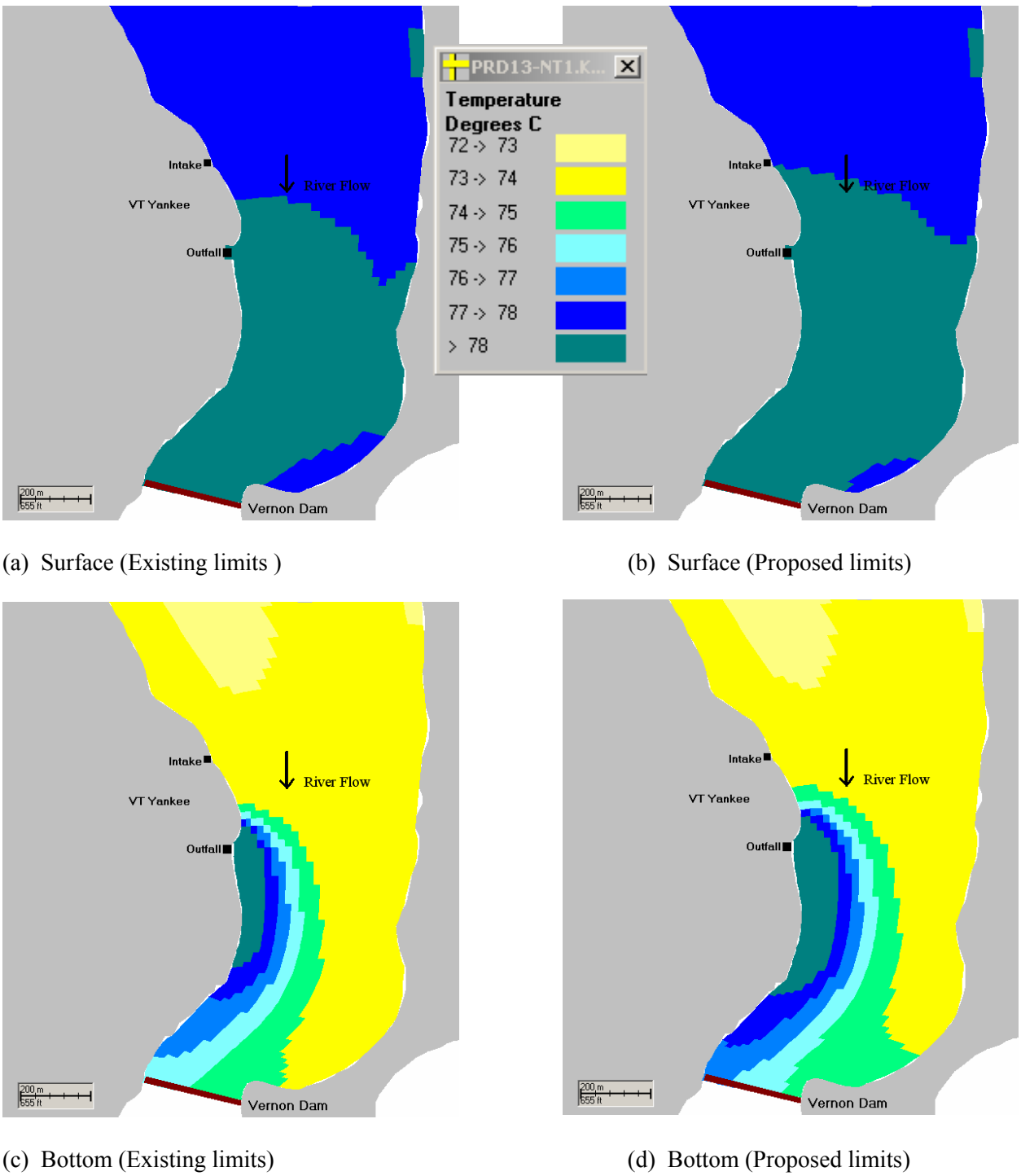
Figure 5-28. Predicted changes in Vermont Yankee's thermal plume surface or bottom area in lower Vernon Pool of the Connecticut River exposed to the average case (50% occurrence) of flow and ambient temperature under existing and proposed new summer thermal discharge limits for the Atlantic salmon (parr and smolts) avoidance temperature of 78°F.
