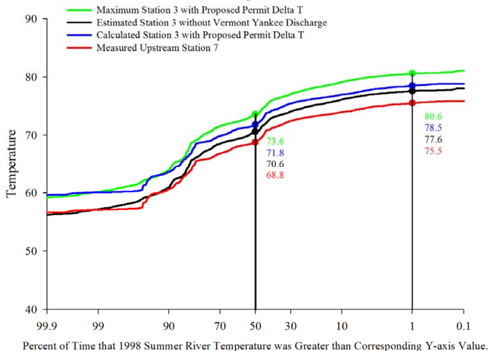
Figure 3-12a. Temperature Duration Curves for the 1998-2002 and 1998 Summer Periods for Selected Connecticut River Monitoring Stations – Proposed Vermont Yankee Discharge Conditions.
