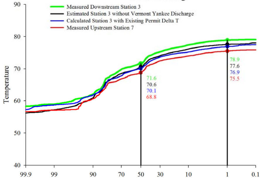
Figure 3-11a. Temperature Duration Curves for the 1998-2002 and 1998 Summer Periods for Selected Connecticut River Monitoring Stations – Existing Vermont Yankee Discharge Conditions.
