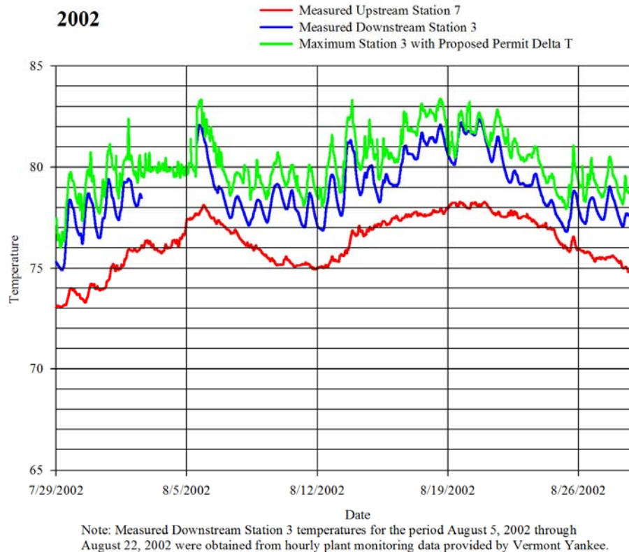
Figure 3-13c. Actual and Predicted Warmest 4-Week Period During the Summer Period (May 16 – October 14) for Selected Connecticut River Monitoring Stations – Existing and Proposed Vermont Yankee Discharge Conditions.
