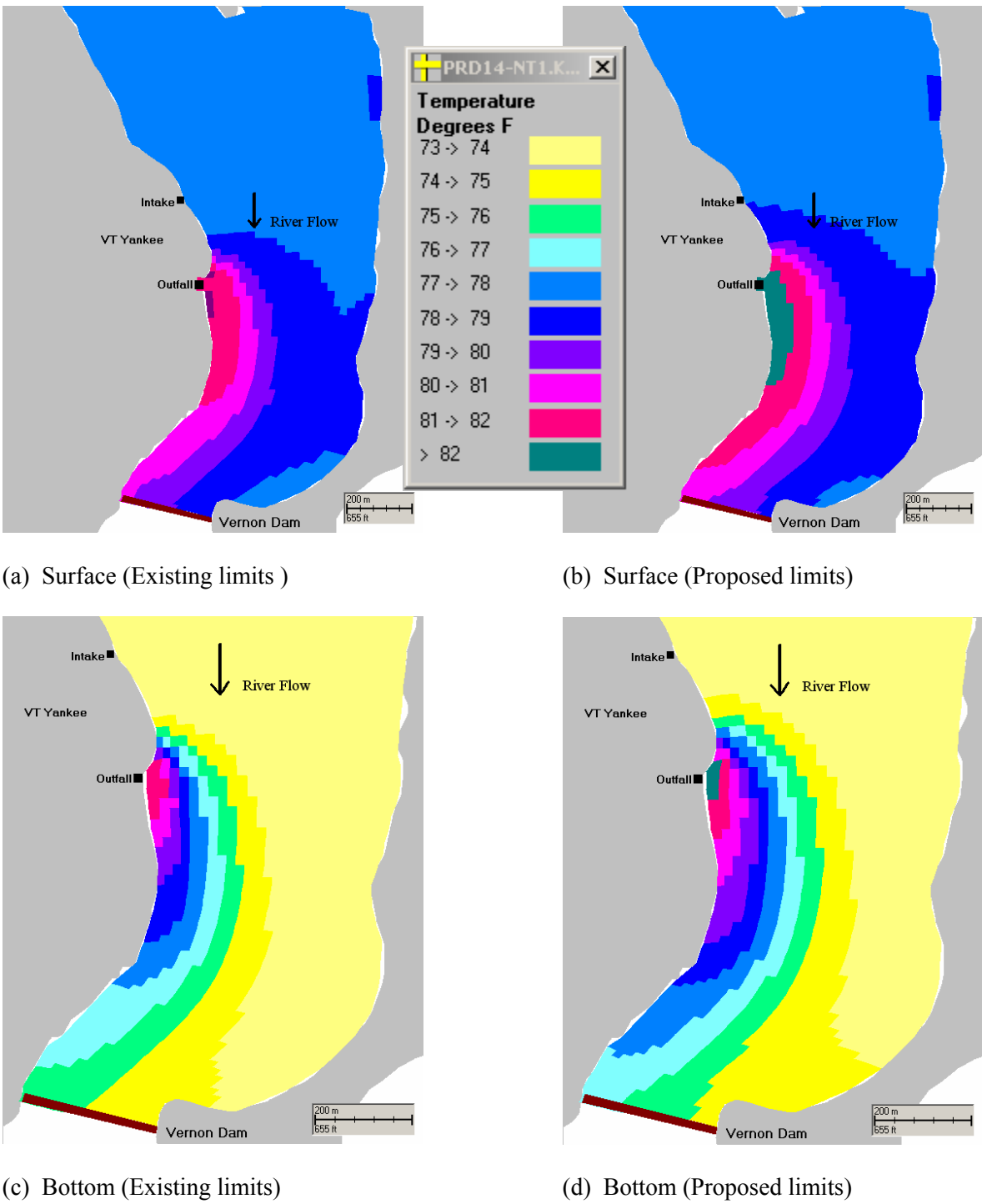
Figure 5-46. Predicted changes in Vermont Yankee's thermal plume surface or bottom area in lower Vernon Pool of the Connecticut River exposed to the average case (50% occurrence) of flow and ambient temperature under existing and proposed new summer thermal discharge limits for the fallfish avoidance temperature of 82°F.
