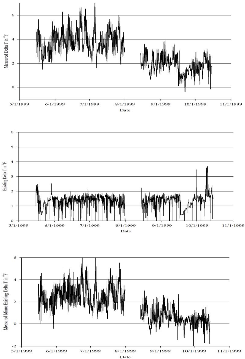
Figure 3-6b. Measured Delta T (Downstream Station 3 Minus Upstream Station 7) Compared to Existing Permit Delta T – 1999 Hourly Data.
