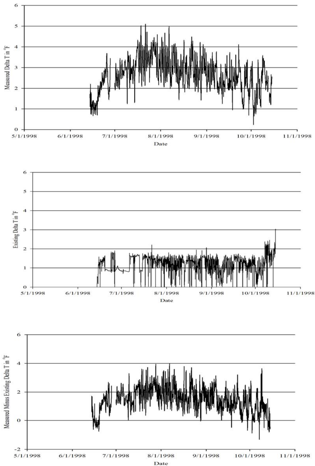
Figure 3-6a. Measured Delta T (Downstream Station 3 Minus Upstream Station 7) Compared to Existing Permit Delta T – 1998 Hourly Data.
