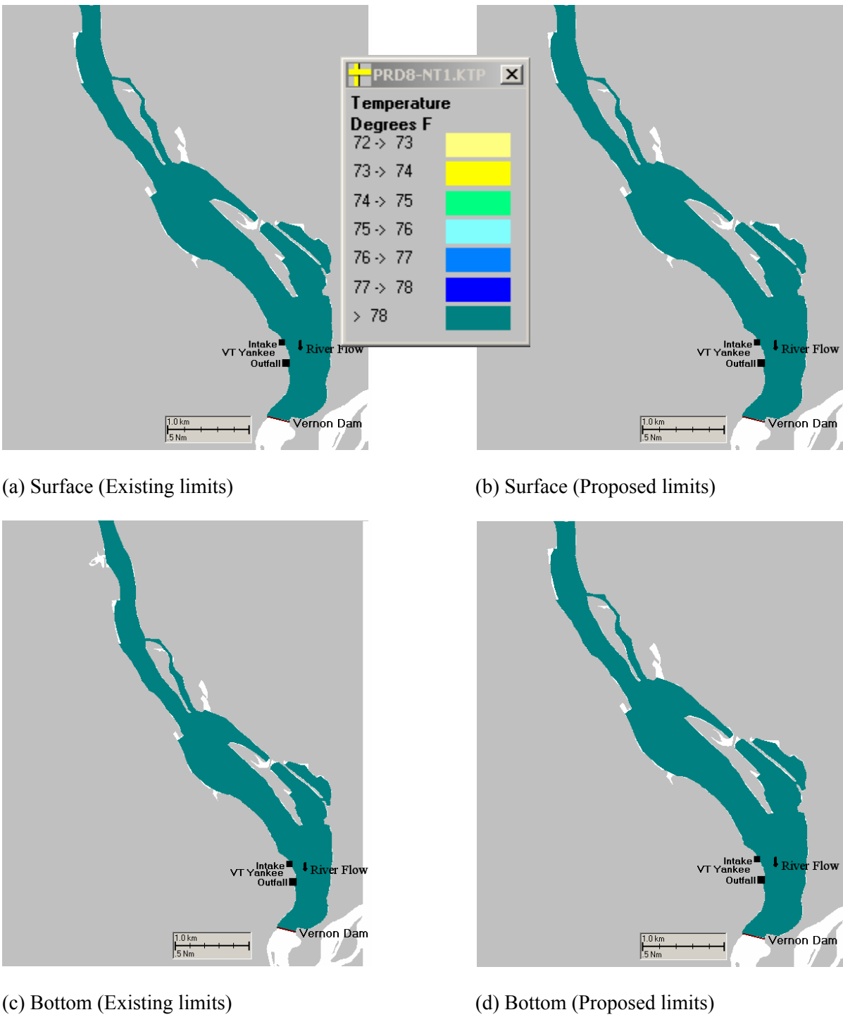
Figure 5-29. Predicted changes in Vermont Yankee's thermal plume surface or bottom area in lower Vernon Pool of the Connecticut River exposed to the extreme case (1% occurrence) of flow and ambient temperature under existing and proposed new summer thermal discharge limits for the Atlantic salmon avoidance temperature of 78°F.
