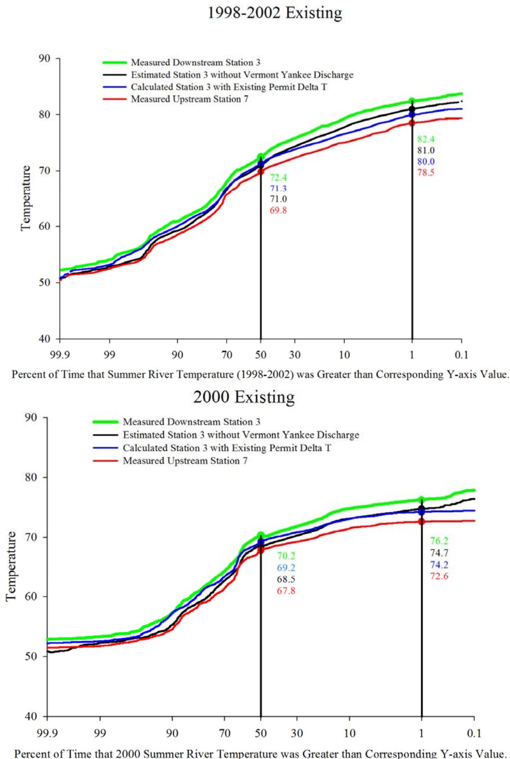
Figure 3-11c. Temperature Duration Curves for the 1998-2002 and 2000 Summer Periods for Selected Connecticut River Monitoring Stations – Existing Vermont Yankee Discharge Conditions.
