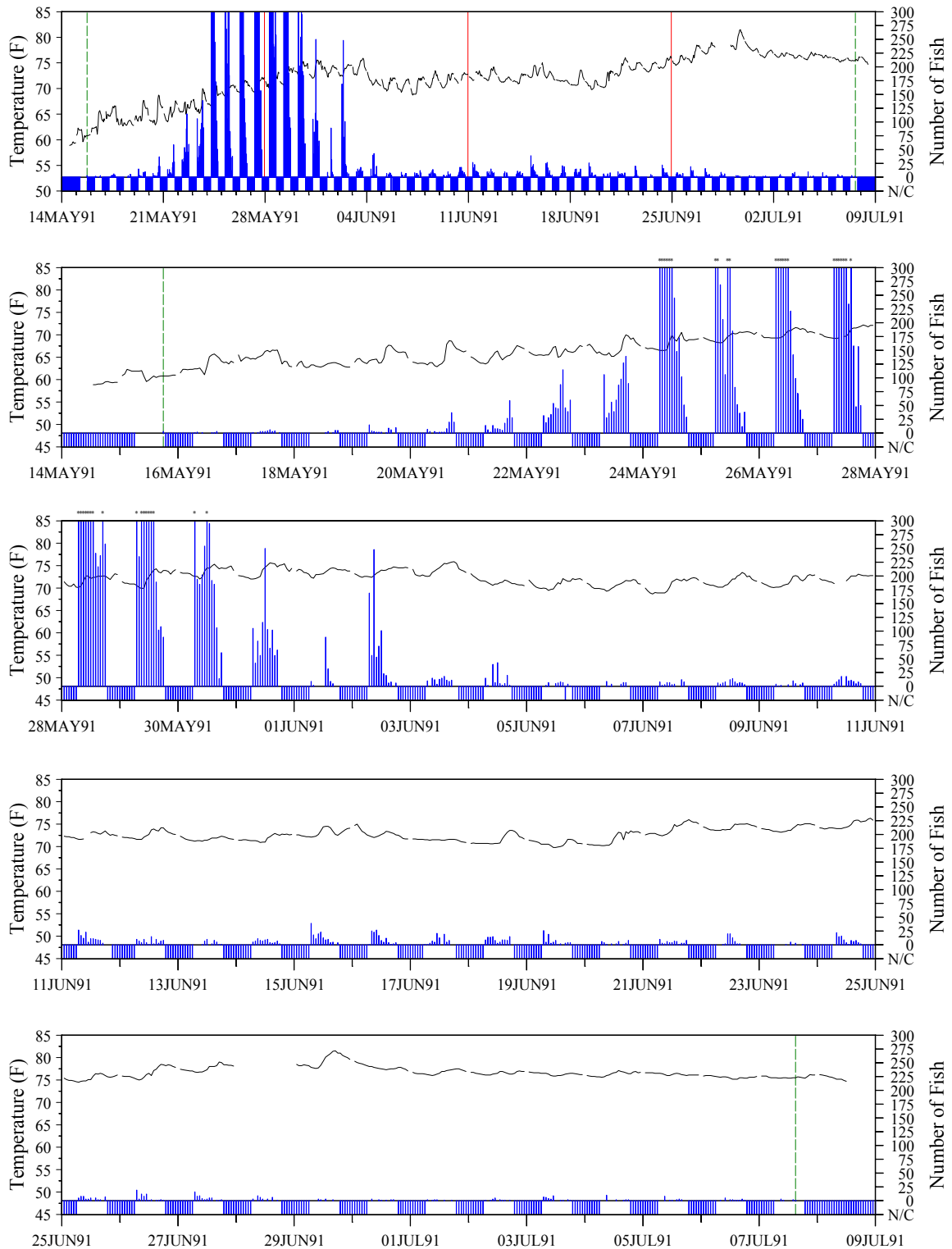
Appendix Figure 6-1. Hourly count of adult American shad passing upstream through the Vernon Dam Fishway on the Connecticut River, Vernon, Vermont and the corresponding hourly average fishway water temperature, 14 May – 9 July, 1991.
