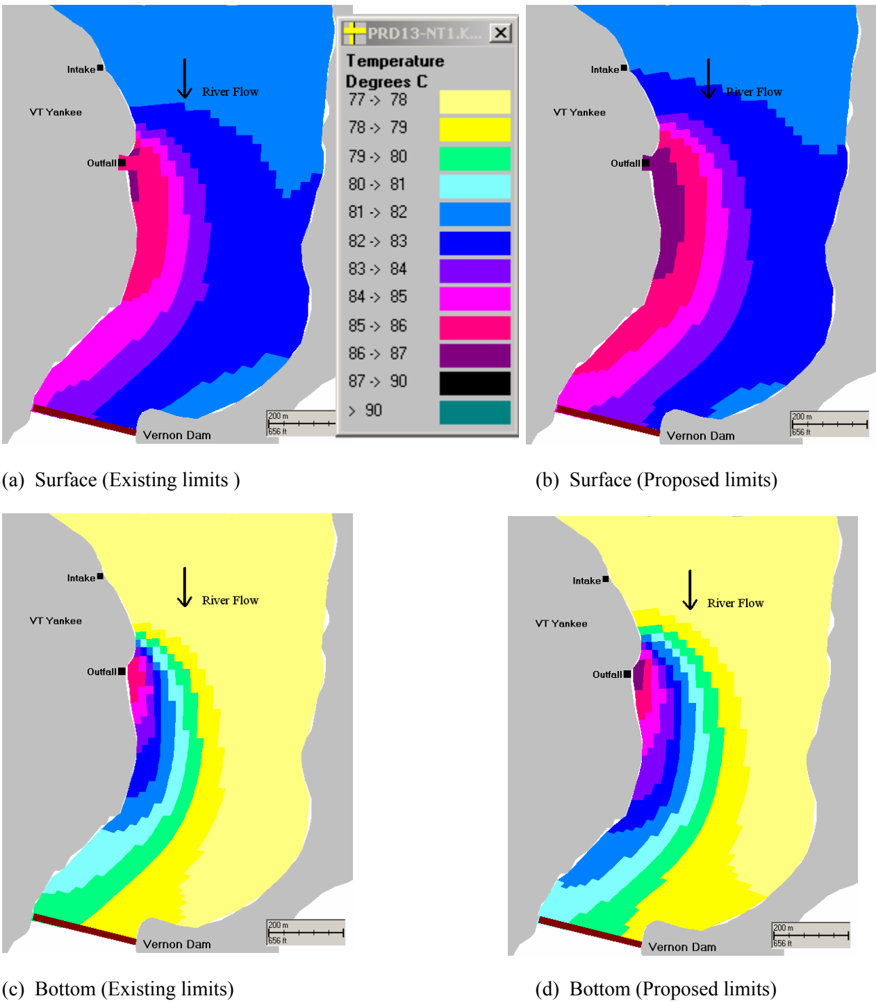
Figure 5-43. Predicted changes in Vermont Yankee's thermal plume surface or bottom area in lower Vernon Pool of the Connecticut River exposed to the average case (50% occurrence) of flow and ambient temperature under existing and proposed new summer thermal discharge limits for the largemouth bass avoidance temperature of 90°F.
