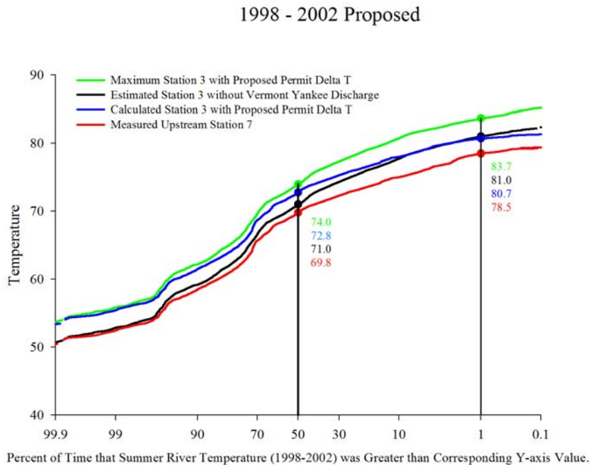
Figure 3-9. Temperature Duration Curves for the Summer Period (1998-2002) for Selected Connecticut River Monitoring Stations – Proposed Vermont Yankee Discharge Conditions.
