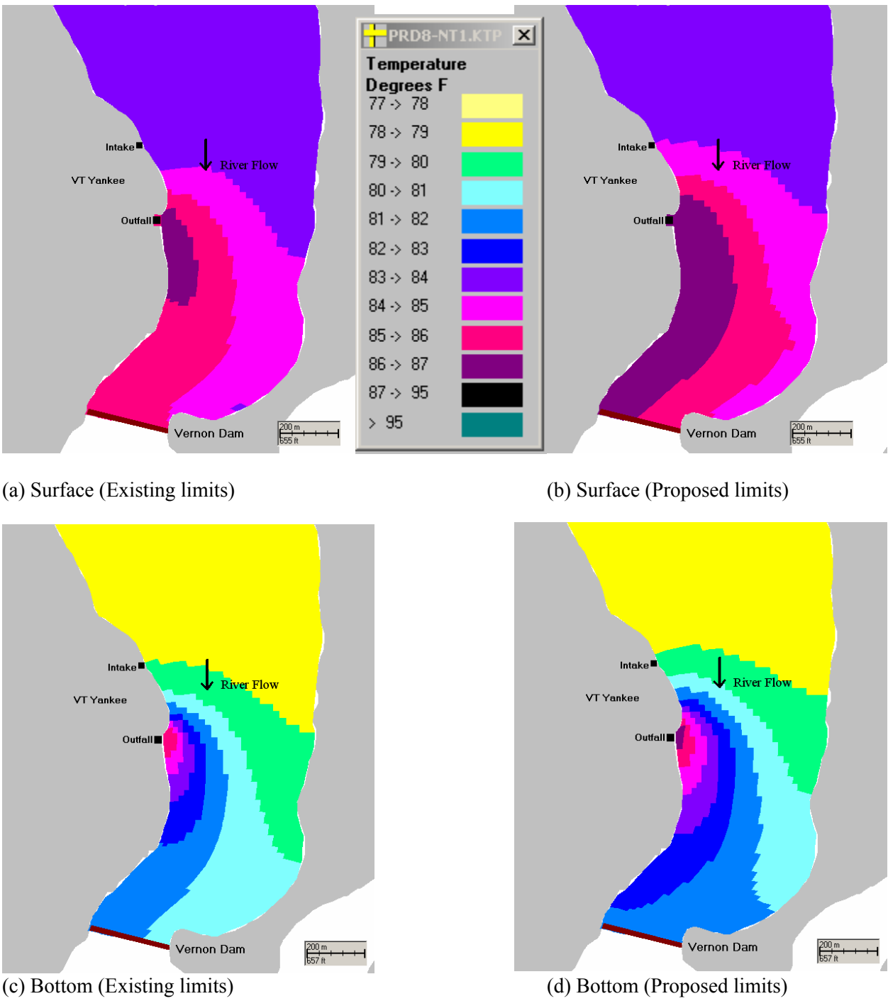
Figure 5-32. Predicted changes in Vermont Yankee's thermal plume surface or bottom area in lower Vernon Pool of the Connecticut River exposed to the extreme case (1% occurrence) of flow and ambient temperature under existing and proposed new summer thermal discharge limits for the spottail shiner avoidance temperature of 95°F.
