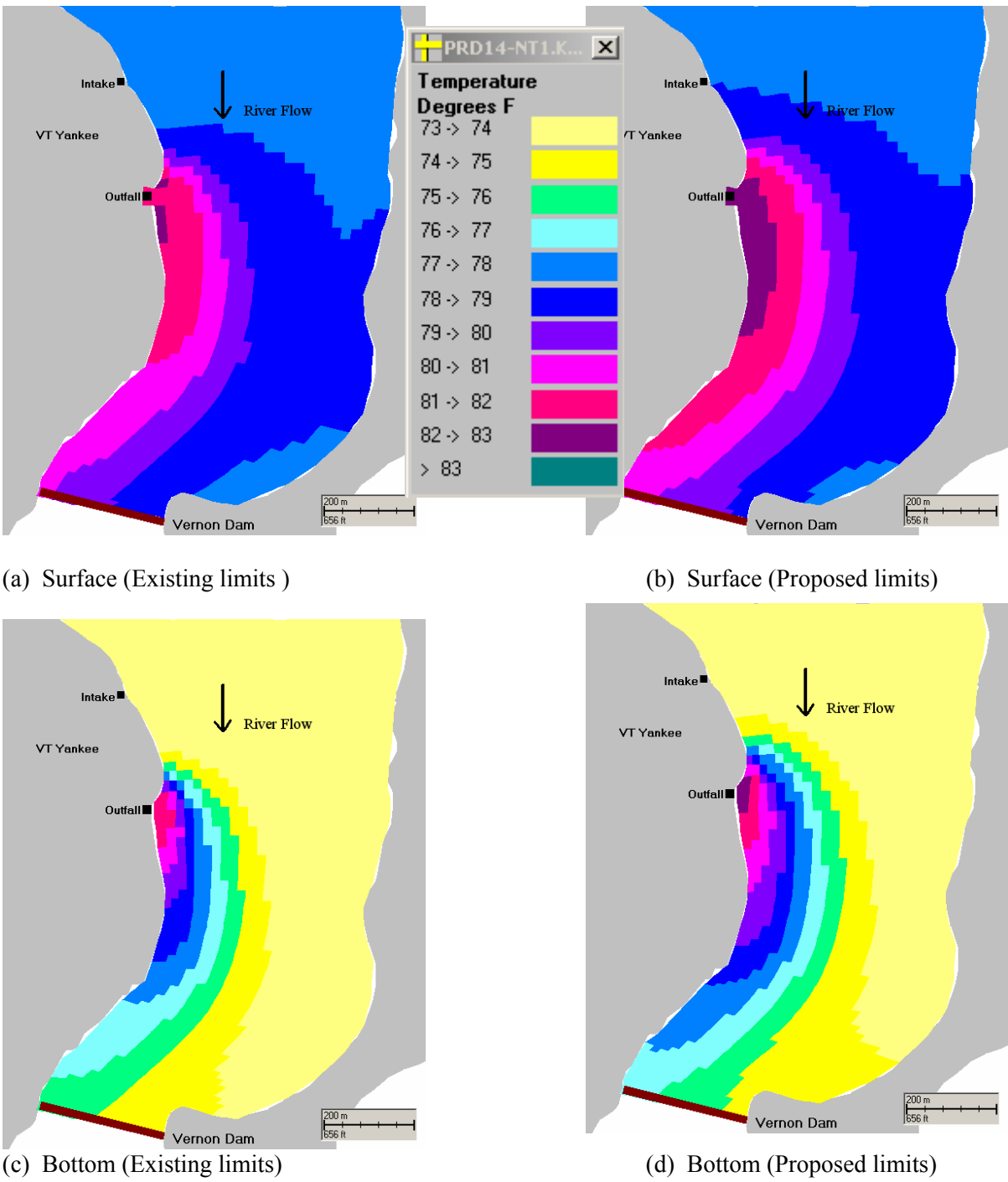
Figure 5-37. Predicted changes in Vermont Yankee's thermal plume surface or bottom area in lower Vernon Pool of the Connecticut River exposed to the average case (50% occurrence) of flow and ambient temperature under existing and proposed new summer thermal discharge limits for the yellow perch avoidance temperature of 83°F.
