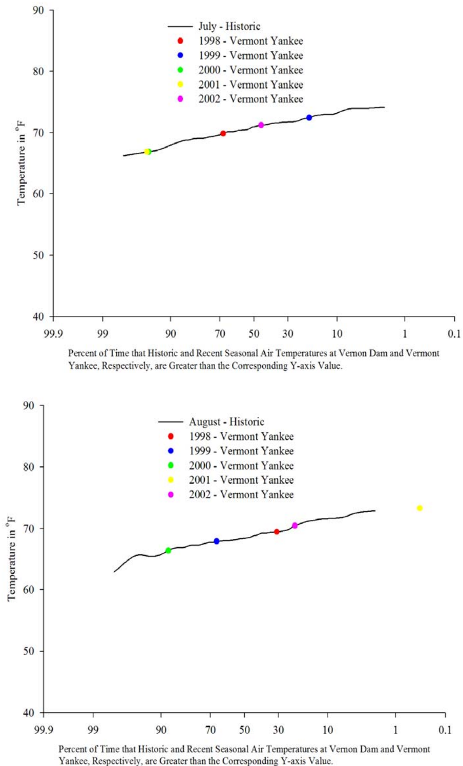
Figure 3-5b. Historic Average July and August Air Temperature Duration Curve at Vernon Dam.
