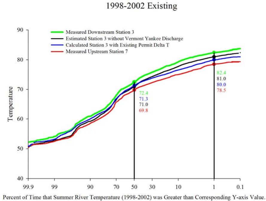
Figure 3-8. Temperature Duration Curves for the Summer Period (1998-2002) for Selected Connecticut River Monitoring Stations – Existing Vermont Yankee Discharge Conditions.
