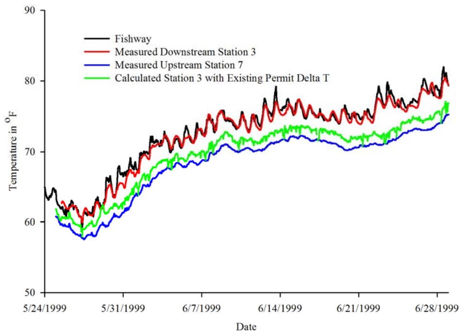
Figure 3-7b. Hourly Temperature at Selected Monitoring Stations in the Vicinity of Vernon Dam during Period of Fishway Operation – 1999.
