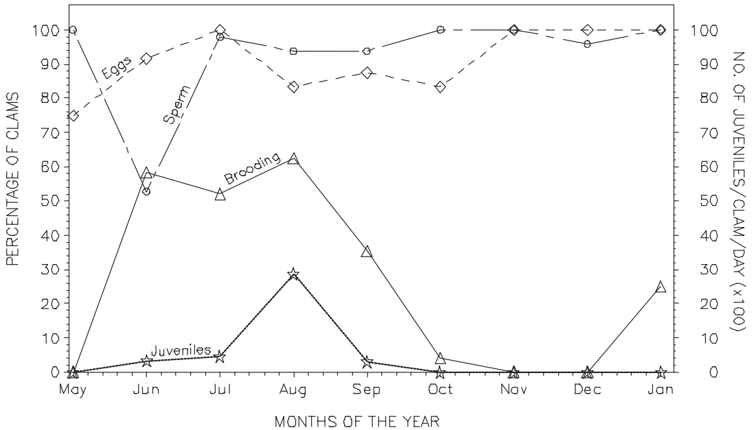
Figure 5. Average seasonal reproductive status of Corbicula fluminea (1991-1994) at ambient river temperatures. The percentage of adult clams (e"8 mm) with mature gametes or brooding young is plotted using the left axis. Active spawning is plotted using the right axis and is defined as the average number juveniles released over a 24-hour period by 12 randomly selected adult clams.
