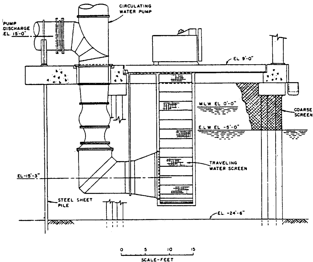
Figure 2-13 No-well screen (SWEC 1980)
