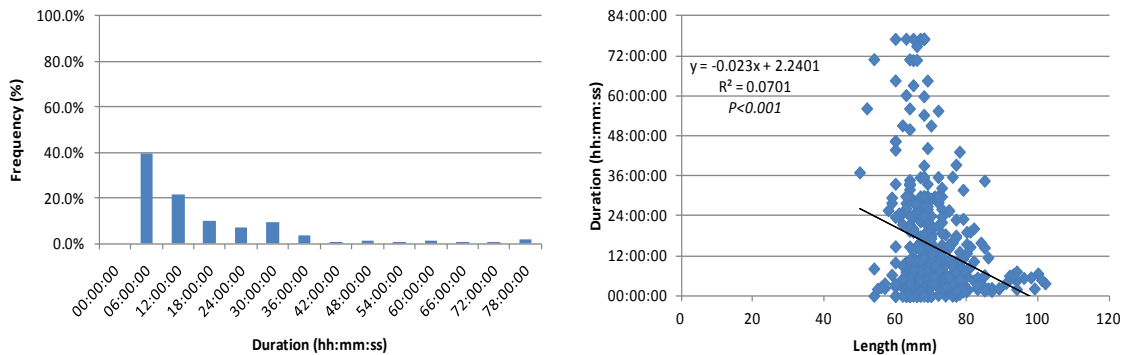
Figure 2-31 Time-to-impingement frequency (left) and length relationship (right) for bluegill during Week 1 testing.
