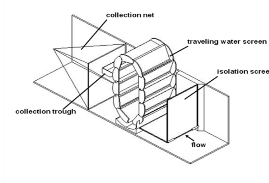
Figure 2-24 Test flume including isolation screen, traveling water screen, collection trough, and collection net
