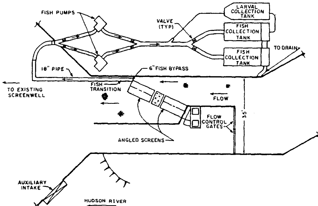
Figure 10-4 Danskammer angled screen system layout (LMS 1985)
