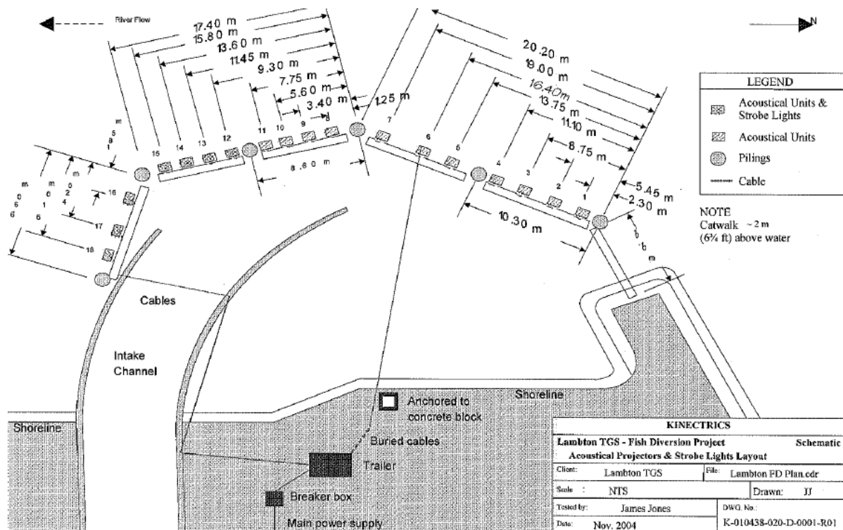
Figure 16-3 Layout of the strobe light-acoustic hybrid system installed at Lambton (Cord et al 2007)
