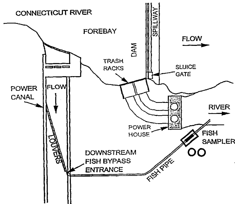
Figure 12-6 Holyoke louver system (Stira and Robinson 1997)
