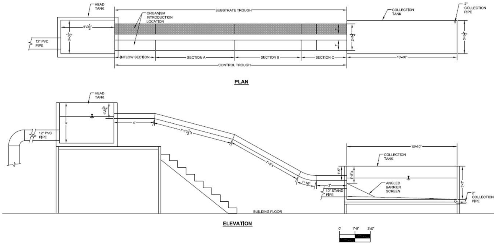
Figure 2-41 Plan and elevation views of the Phase III fish return testing facility
