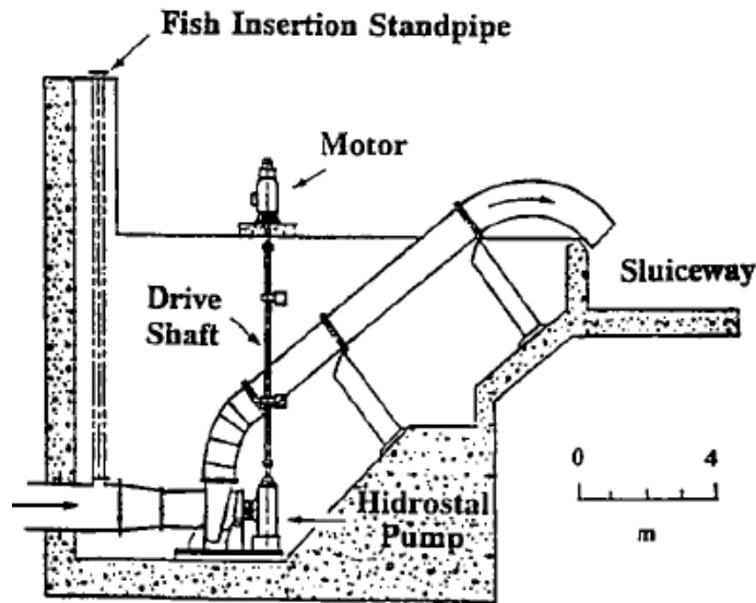
Figure 9-4 Cut-away perspective of the Hidrostal pump in bay 3 of the Red Bluff Research Pumping Plant, Sacramento River, California. During operations entrained fish were carried upward and discharged into a sluiceway that led downstream to the vertical screens shown in Figure 9-2 (McNabb et al. 2003).
