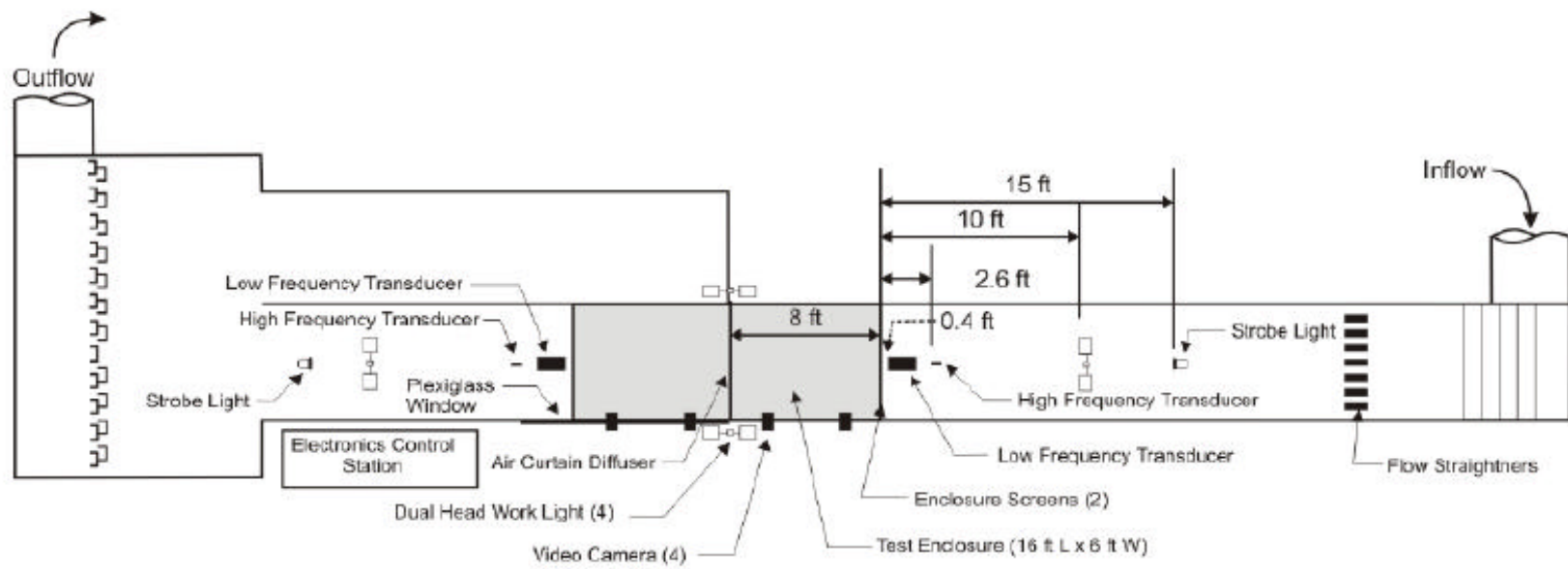
Figure 16-6 Overhead schematic of the test facility (PSEG 2003)
