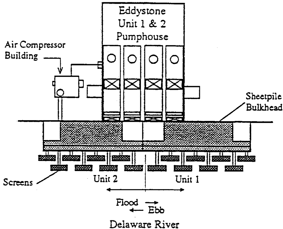
Figure 5-4 Wedge wire intake system at Eddystone Station (Veneziale 1991)
