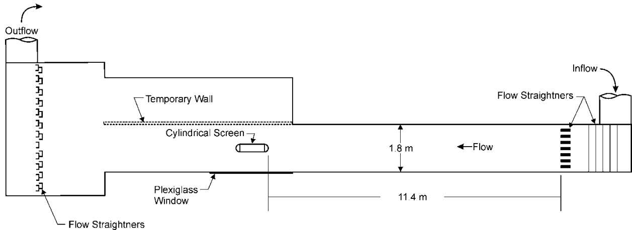
Figure 5-7 Fish testing facility and approximate location of cylindrical wedgewire screens (EPRI 2003)
