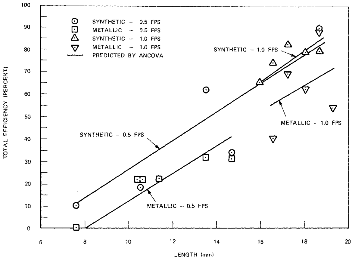
Figure 10-11 Total efficiency versus length for 2.5 mm mesh 1978 striped bass diversion study (Taft et al. 1981b)
