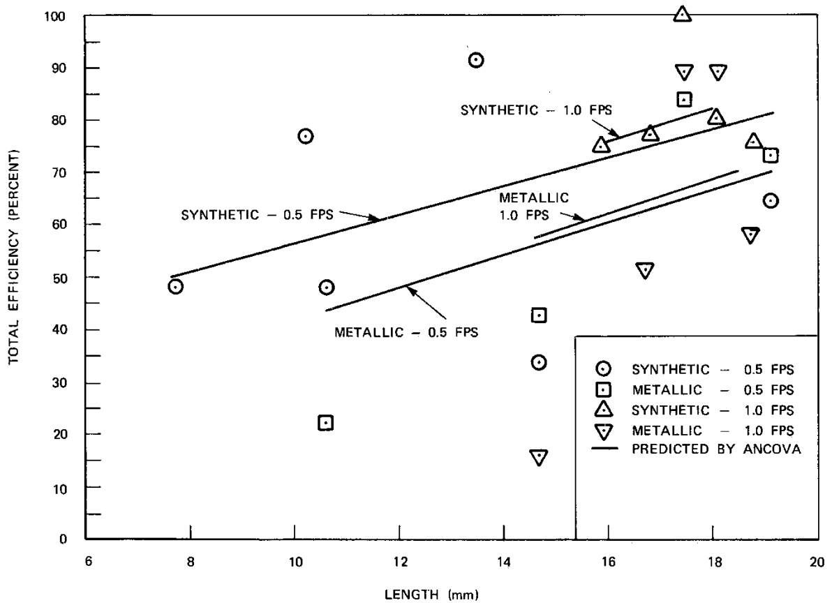
Figure 10-10 Total efficiency versus length for 1.5 mm mesh 1978 striped bass diversion study (Taft et al. 1981b)
