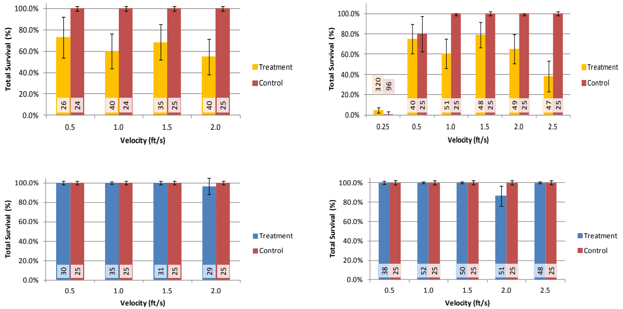
Figure 2-29 Common carp total survival on the OVIVO screen (left) and WIP screen (right). The total number of fish held for LM evaluation is presented at the base of each bar. 95% confidence intervals (shown as error bars) were calculated using the normal approximation of the binomial distribution.
