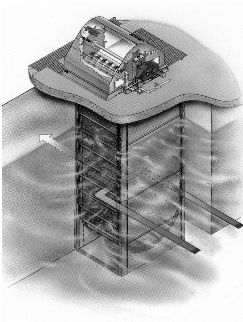
Figure 2-10 Schematic of a dual-flow traveling intake screen (courtesy of U.S. Filter)
