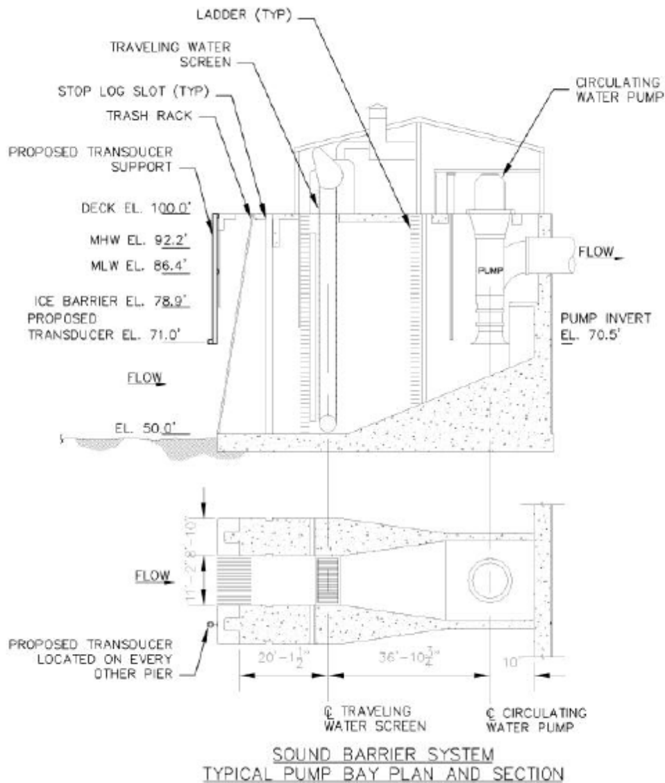
Figure 16-7 Section and overhead view of the proposed sound system at Salem (PSEG 2003)
