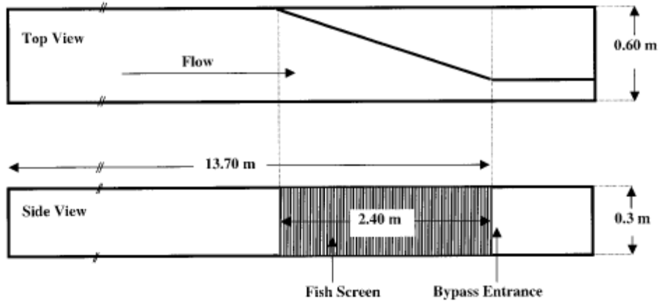
Figure 10-12 Diagram of the open-topped, glass water flume swimming chamber and bypass channel
