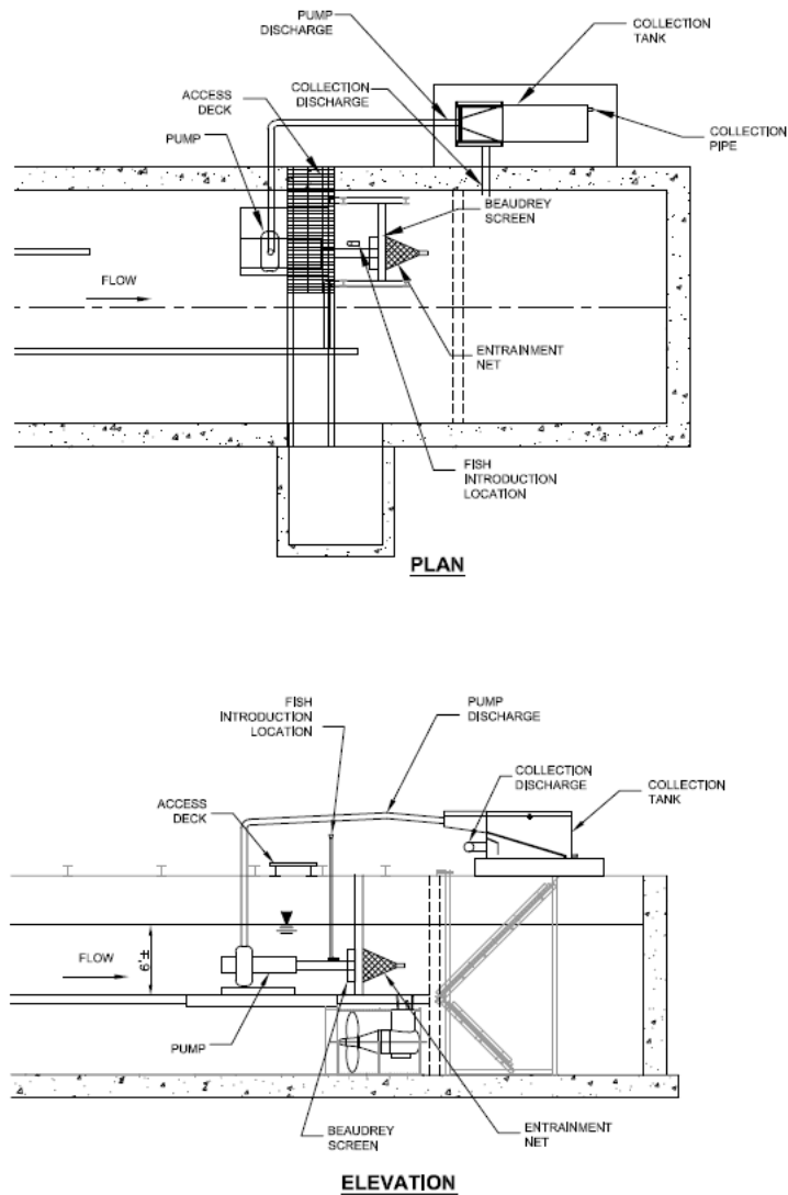
Figure 2-36 Taft Fisheries Research and Test Facility configured for the Phase II biological evaluation of the Beaudrey WIP screen.
