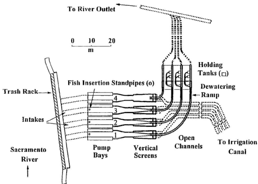
Figure 9-2 Schematic of the Red Bluff Research Pumping Plant, Sacramento River, CA. Archimedes lifts were in pump bays 1 and 2. The Hidrostal pump was in bay 3, and bay 4 was empty. Dotted lines indicate underground portions of water intakes, the conveyance system for irrigation water, and the fish bypasses (McNabb et al. 2003).
