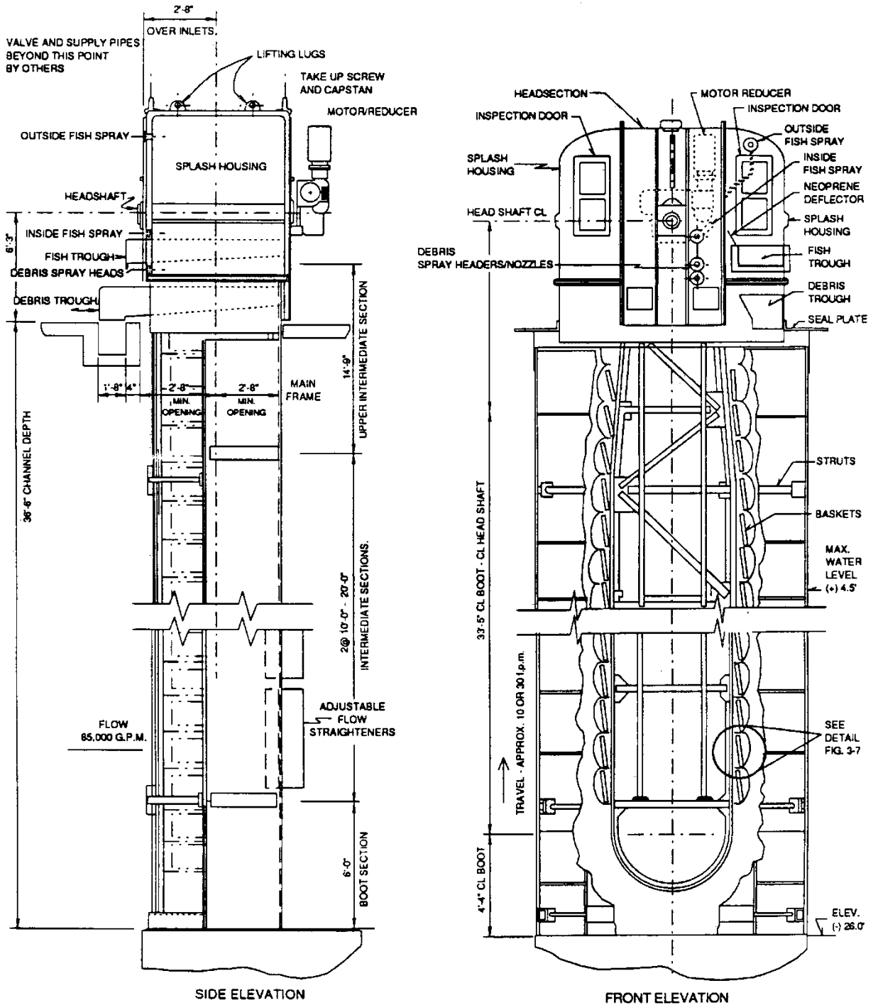
Figure 2-11 Section view of Roseton dual-flow traveling screen (LMS 1991)
