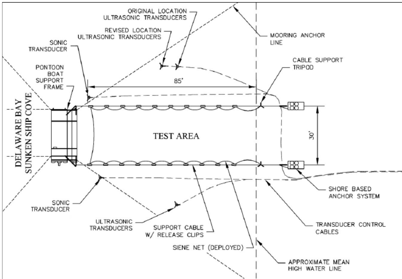
Figure 16-1 Plan view of the sampling equipment and test area (PSEG 2005)
