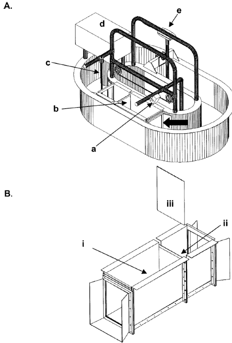
Figure 10-9 Test tank (A) showing (a) video camera, (b) test chamber, (c) velocity meter), (d) cooling unit, and (e) propeller system. The thick black arrow shows the direction of flow. (B) Test chamber, showing (i) release area, (ii) capture area, and (iii) position of removable test screen (Zytlewski and Johnson 2002).
