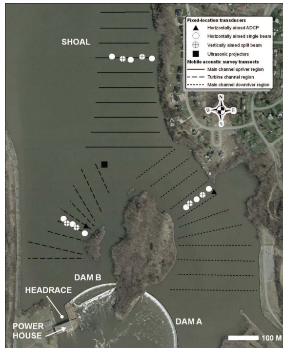
Figure 14-1 Locations of eight ultrasonic (122–128 kHz) projectors, a horizontally aimed, 500-kHz acoustic Doppler current profilers (ADCPs), 420-kHz, horizontally-aimed single-beam transducers and vertically-aimed split-beam transducers (mounted from the river bottom), and mobile hydroacoustic survey transects used for the 2008 evaluation of high-frequency sound at the Crescent Project (Dunning and Gurshin 2012).
