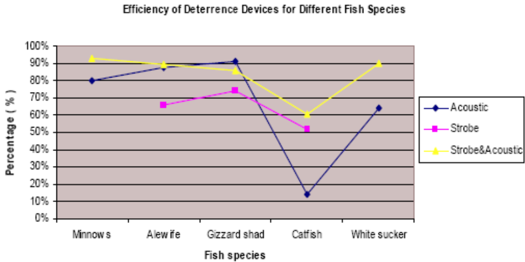
Figure 16-10 Efficiency comparisons for deterrence devices for five species (Patrick et al. 2006b)
