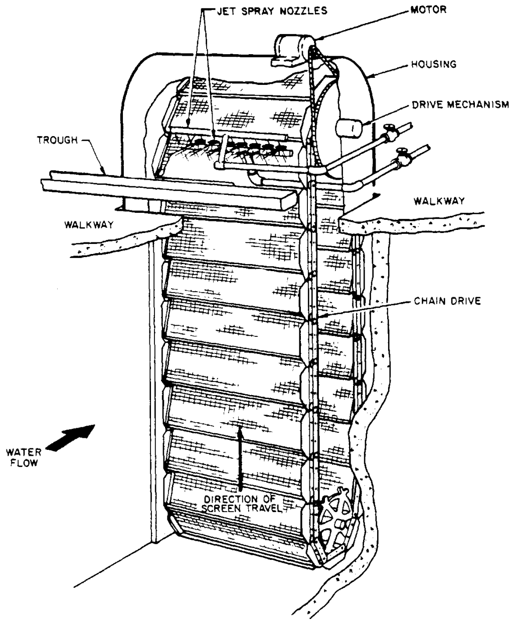
Figure 2-2 Schematic of a conventional traveling water screen
