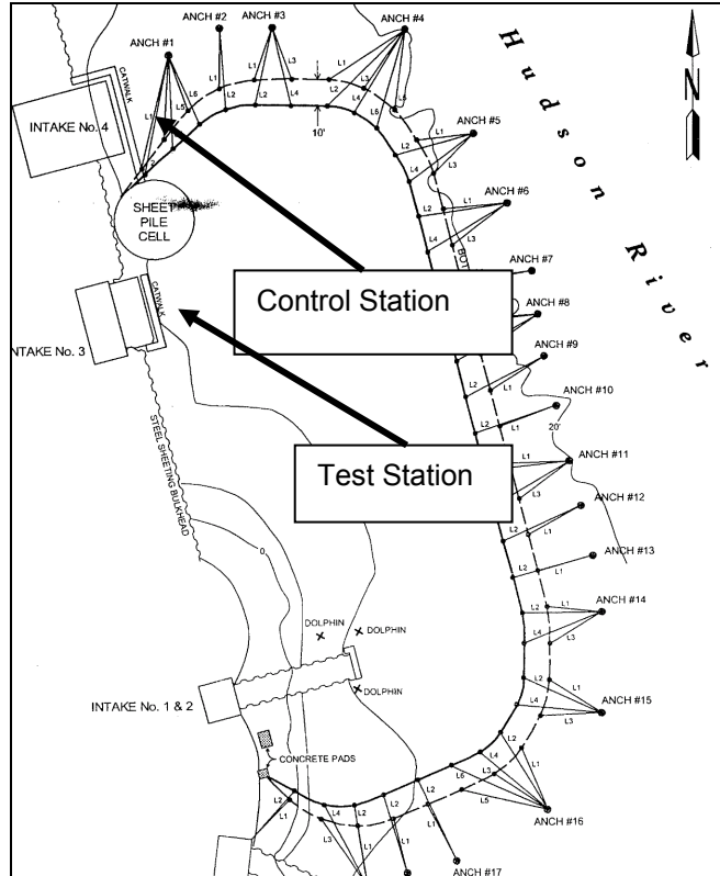
Figure 7-3 Site plan of the AFB deployment at the Lovett Generating Station showing sampling locations for entrainment sampling conducted between 1995 and 1999 (LMS 1998a,b).
