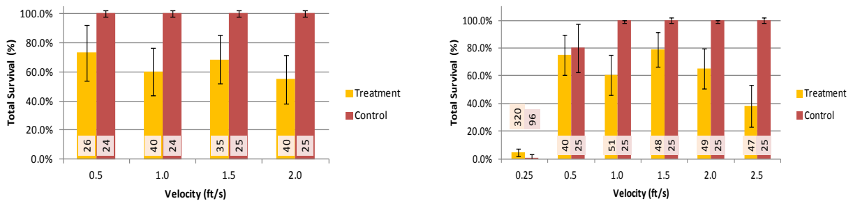
Figure 2-30 Golden shiner total survival on the OVIVO screen (left) and WIP screen (right). The total number of fish held for LM evaluation is presented at the base of each bar. 95% confidence intervals (shown as error bars) were calculated using the normal approximation of the binomial distribution.
