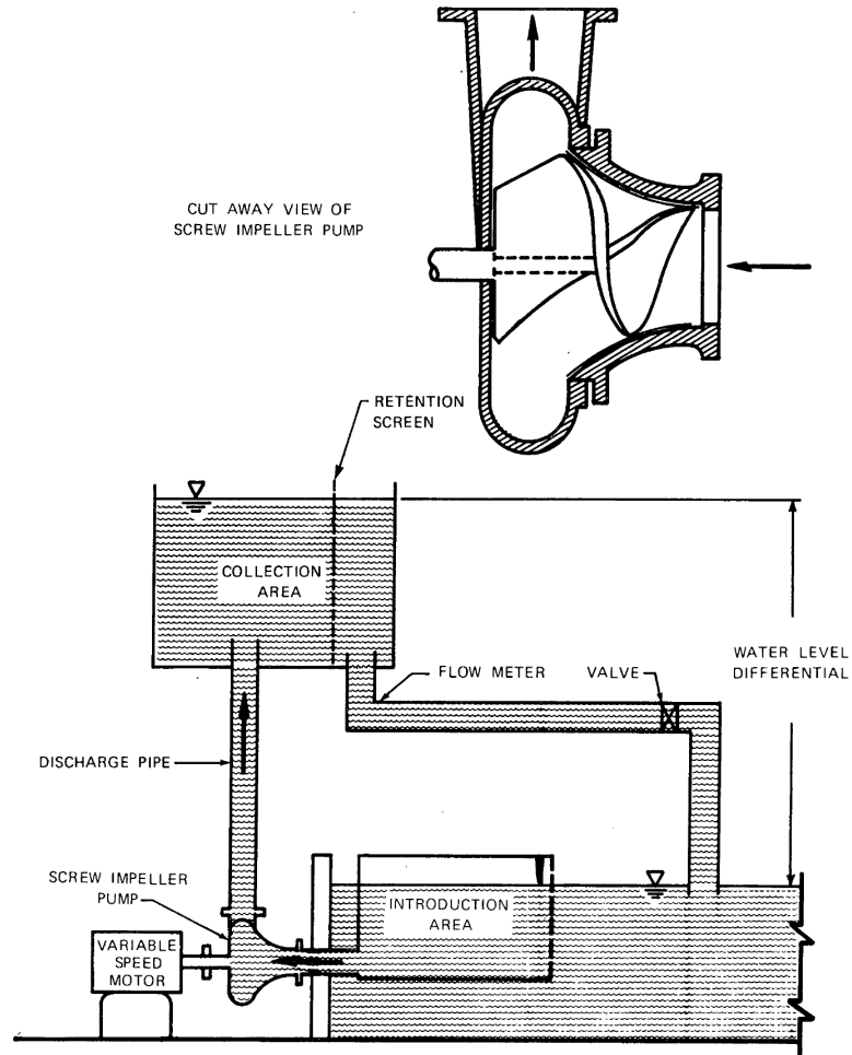
Figure 9-9 Hidrostal pump test facility (ESEERCO 1981b)
