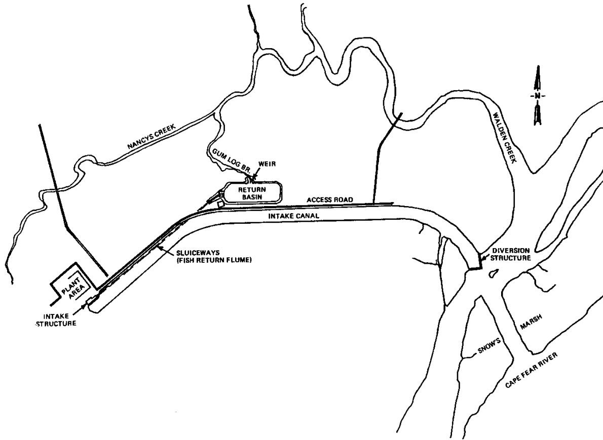
Figure 3-1 Brunswick Plant layout and fish diversion barrier screen (Carolina Power and Light 1985b)
