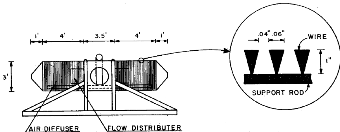
Figure 5-18 Test module with wire design (University of Iowa, Institute of Hydraulic Research)
