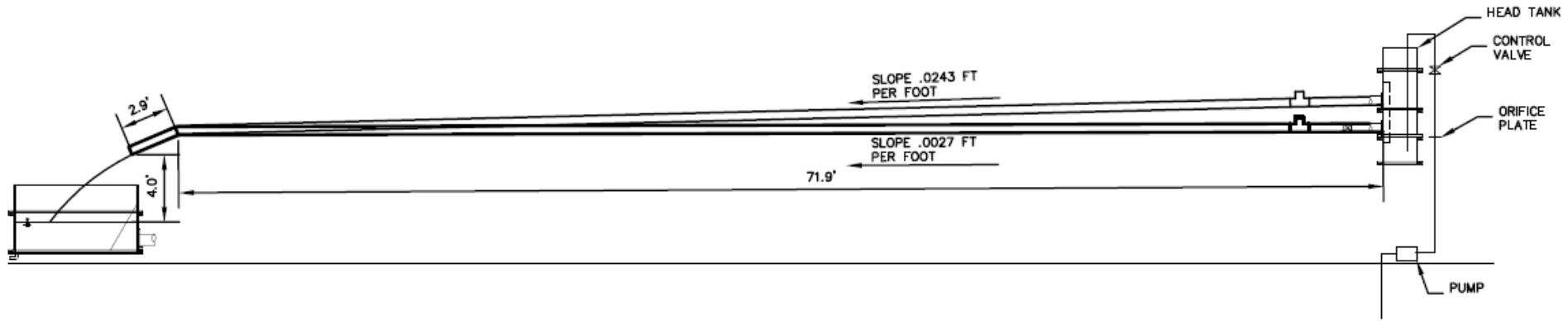
Figure 2-37 Section view of fish return system testing loop with collection box at the 4 ft discharge height.
