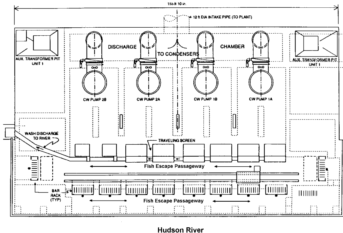
Figure 2-9 Plan view of Roseton cooling water intake structure (modified from LMS 1991)
