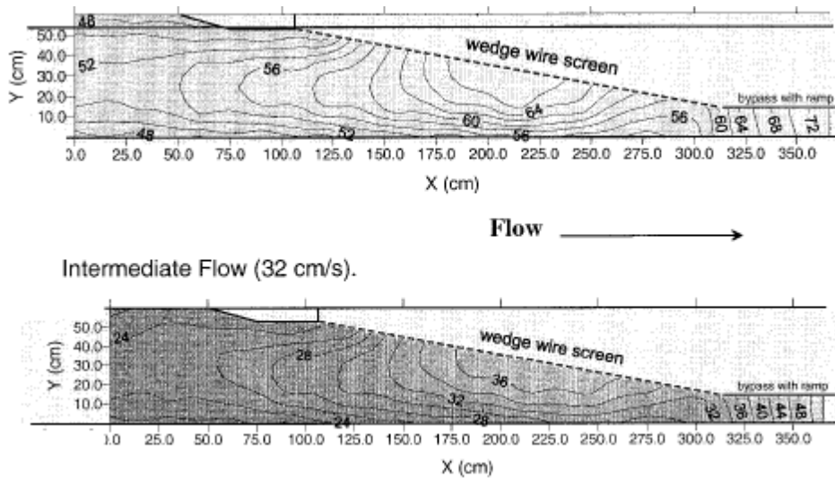
Figure 10-13 Flow maps of water velocities at middepth (8 cm) in the high-velocity, high-bypass (60 cm/s with a 72 cm/s bypass) and intermediate-velocity (32 cm/sec) treatments near the fish screen. The x-axis indicates distance along the length of the flume, the y-axis indicates width, and the contour lines indicate water velocities (cm/sec).
