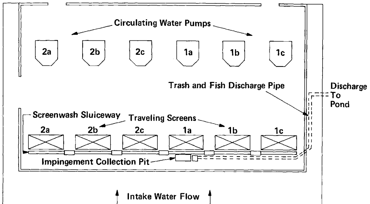
Figure 2-16 Bowline Point Station intake structure (King et al. 1978)
