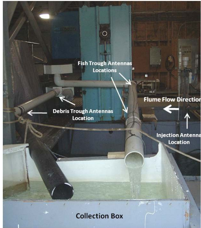
Figure 2-28 Ovivo screen collection system and PIT tag antenna locations.
