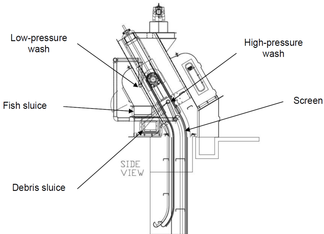
Figure 2-20 Hydrolox™ screen installed at the Barrett Generating Station, 2007
