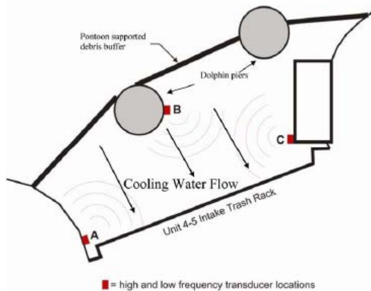
Figure 16-5 Locations of the 3 sonic and 5 ultrasonic sound frequency transducers inside the intake forebay of the Units 4-5 CWIS. One sonic and two ultrasonic transducers are located on each side of the intake structure (A and C). Location B is equipped with only one sonic and one ultrasonic transducer.
