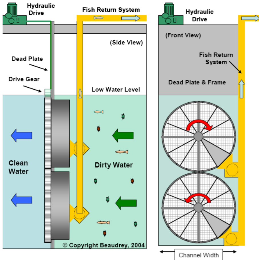
Figure 2-5 Schematic of a Beaudrey WIP screen (Source: Beaudrey)
