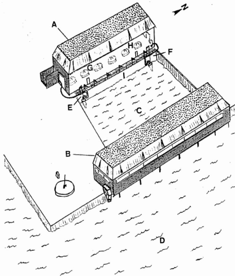
Figure 2. Schemata of the Belle River Power Plant showing sampling stations and other pertinent information. A = Pump house B = Screen house C = Forebay D = St. Clair River E = Unit #1 (south) F = Unit #2 (north) G = Unit #1 Circulation Pumps (3) H = Unit #2 Circulation Pumps (3) I = Catwalk with POC sampling stations
