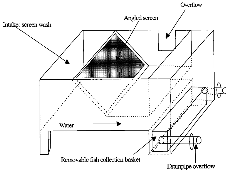
Figure 2-7 Somerset Station fish collection table (McLaren and Tuttle 2000)
