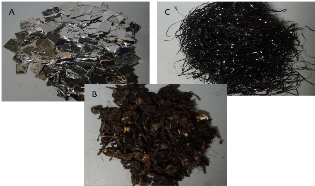
Figure 2-42 The surrogate debris group included mylar (A), wood chips (B), and tinsel (C) debris
