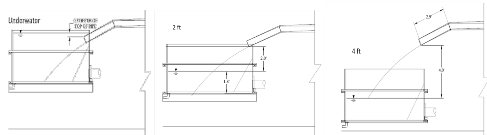
Figure 2-38 Configuration of collection box at each discharge height; underwater, 2 ft, and 4 ft.
