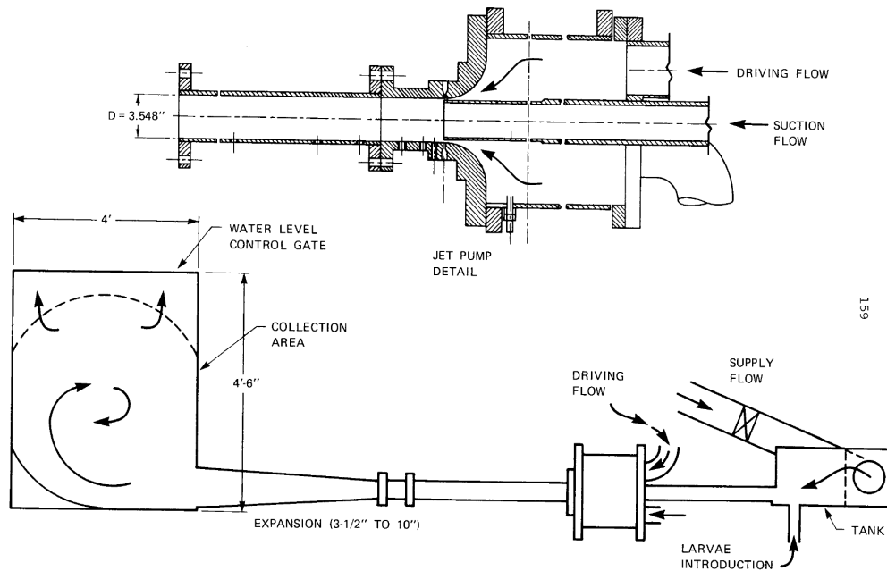
Figure 9-8 Jet pump test facility (ESEERCO 1981b)
