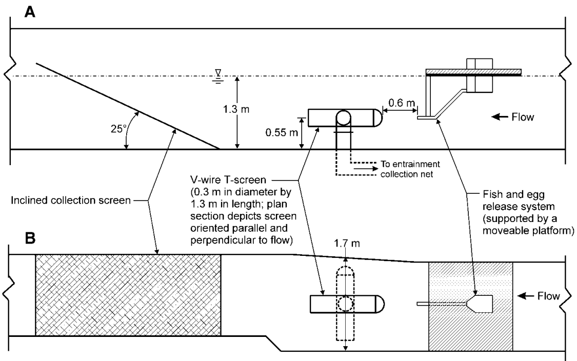
Figure 5-8 2001 wedgewire screen test facility (EPRI 2003)
