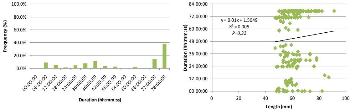
Figure 2-32 Time-to-impingement frequency (left) and length relationship (right) for common carp during Week 1 testing.
