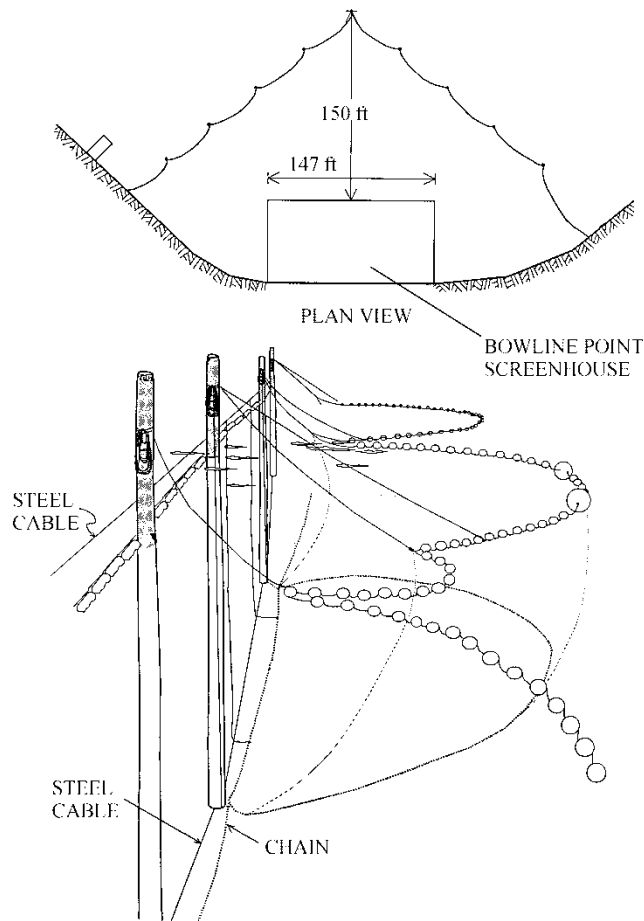
Figure 6-3 Bowline Point fine-mesh barrier net configuration (LMS 1994)
