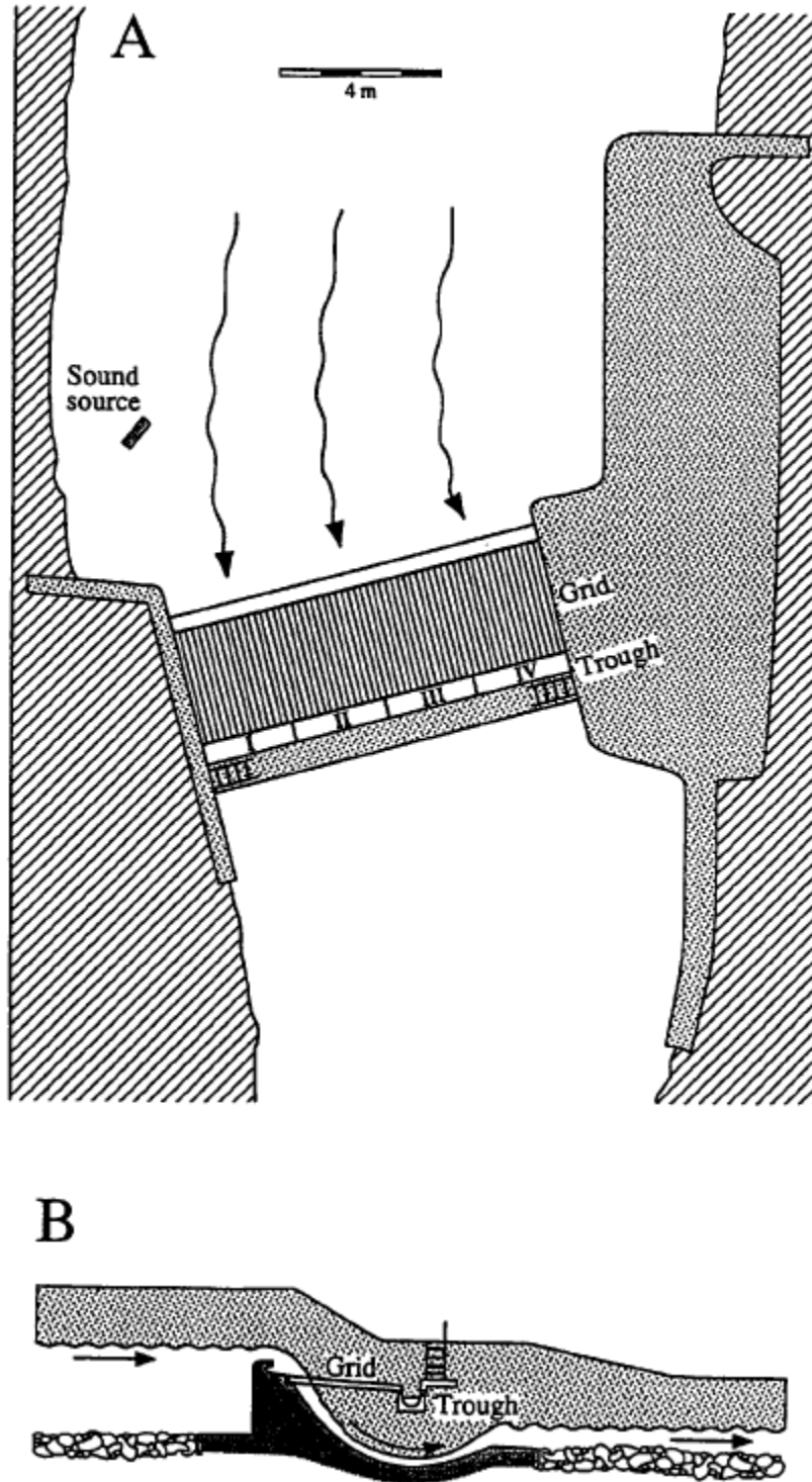
Figure 14-3 Sketch of the River Imsa at the site of the fish trap. (A) Horizontal view showing the position of the infrasound source relative to the trap. The collecting trough of trap was separated into four equal sections (I–IV). (B) Longitudinal section of the trap, which catches all of the descending fish (Sand et al. 2000).
