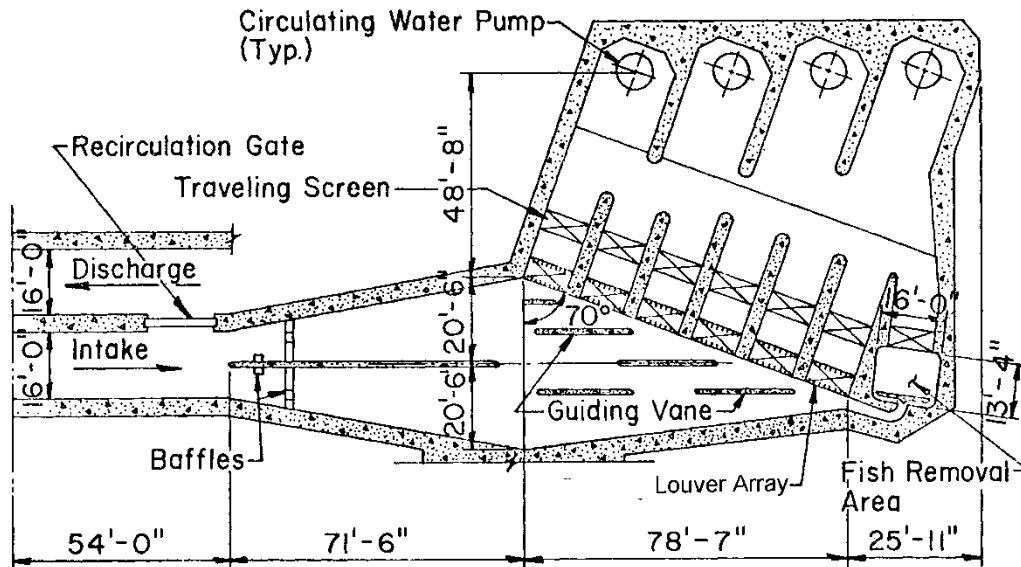
Figure 12-12 Louver system at SONGS (EPRI 1987)
