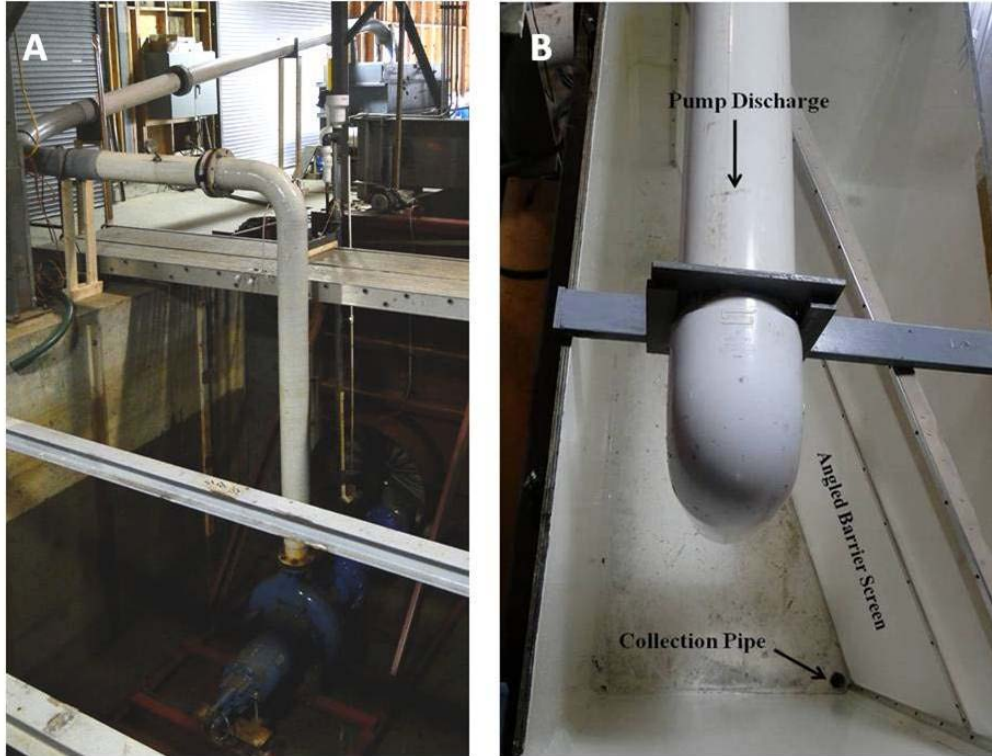
Figure 2-33 Discharge line from the pump to the collection box (A) and inside view of the collection box (B)
