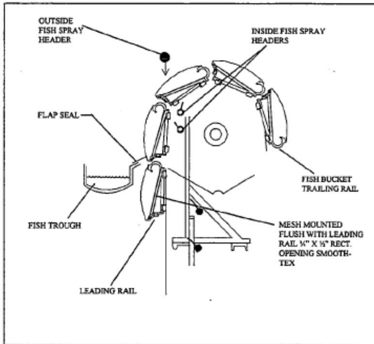
Figure 2-3 Section of a traveling water screen modified for fish protection (Ronafalvy et al. 2000)
