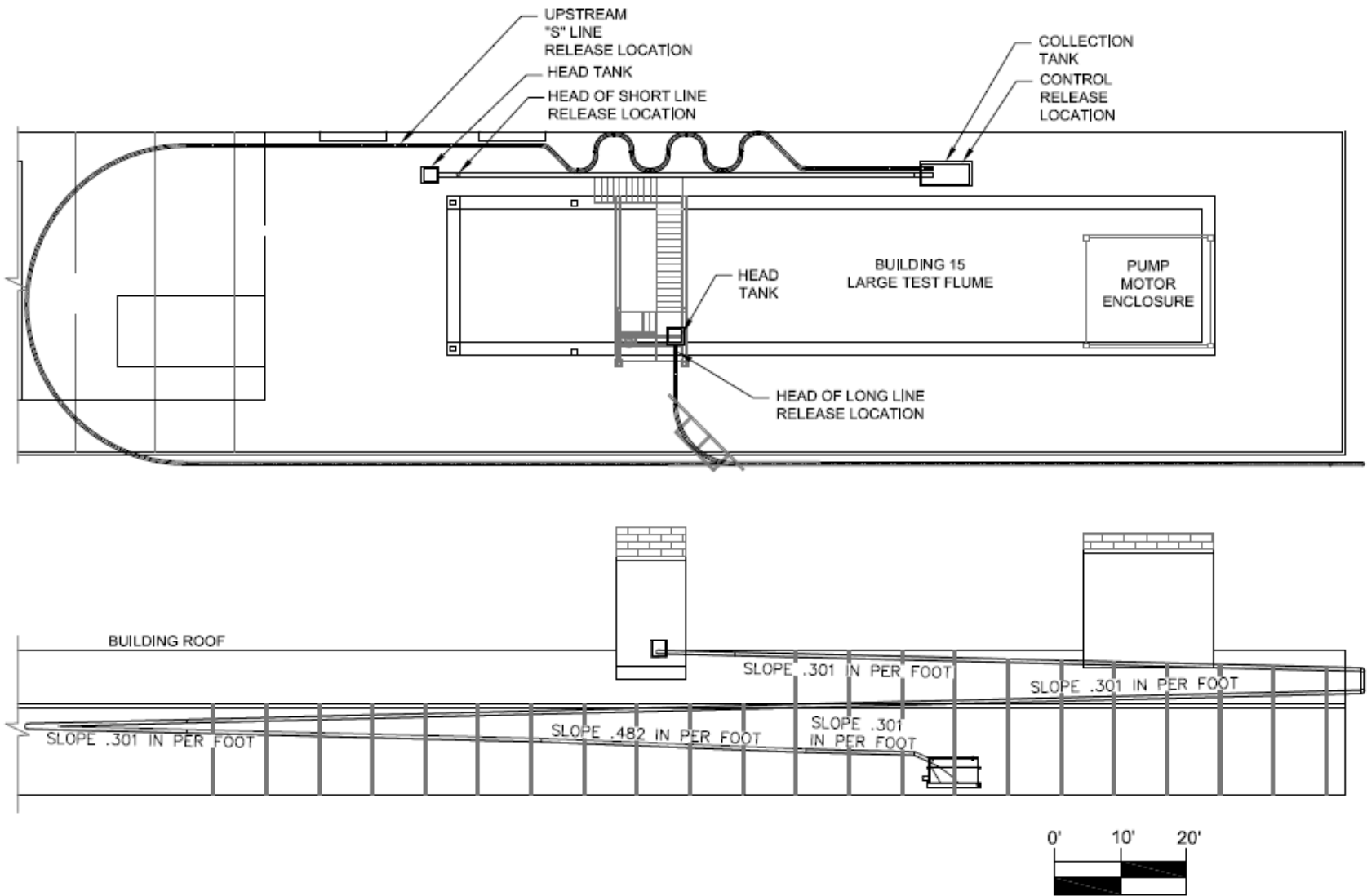
Figure 2-39 Plan and section view of the Phase II fish return line testing facility
