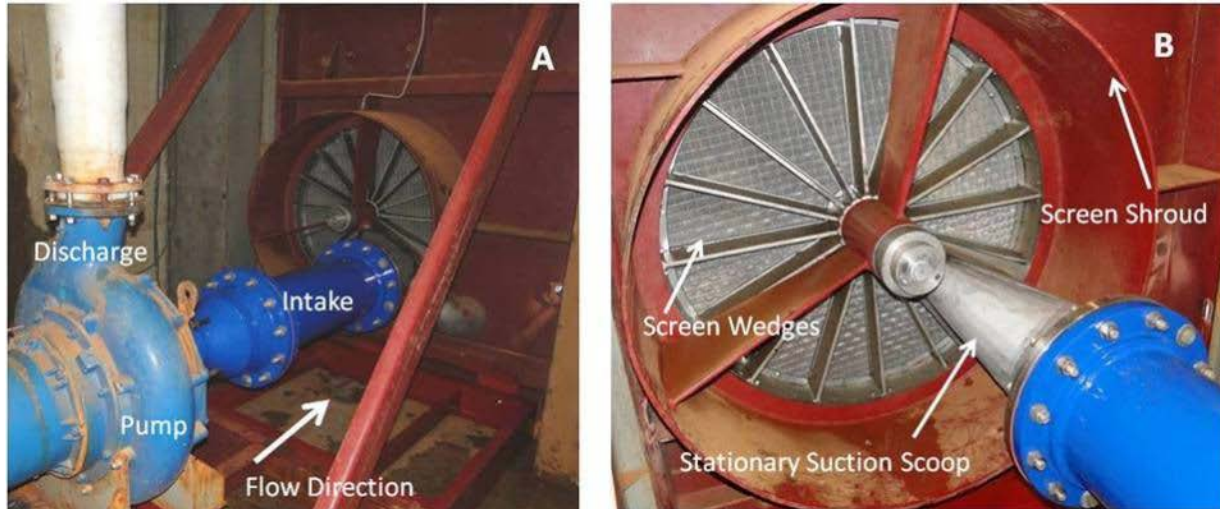
Figure 2-34 Prototype Beaudry WIP screen and pump
