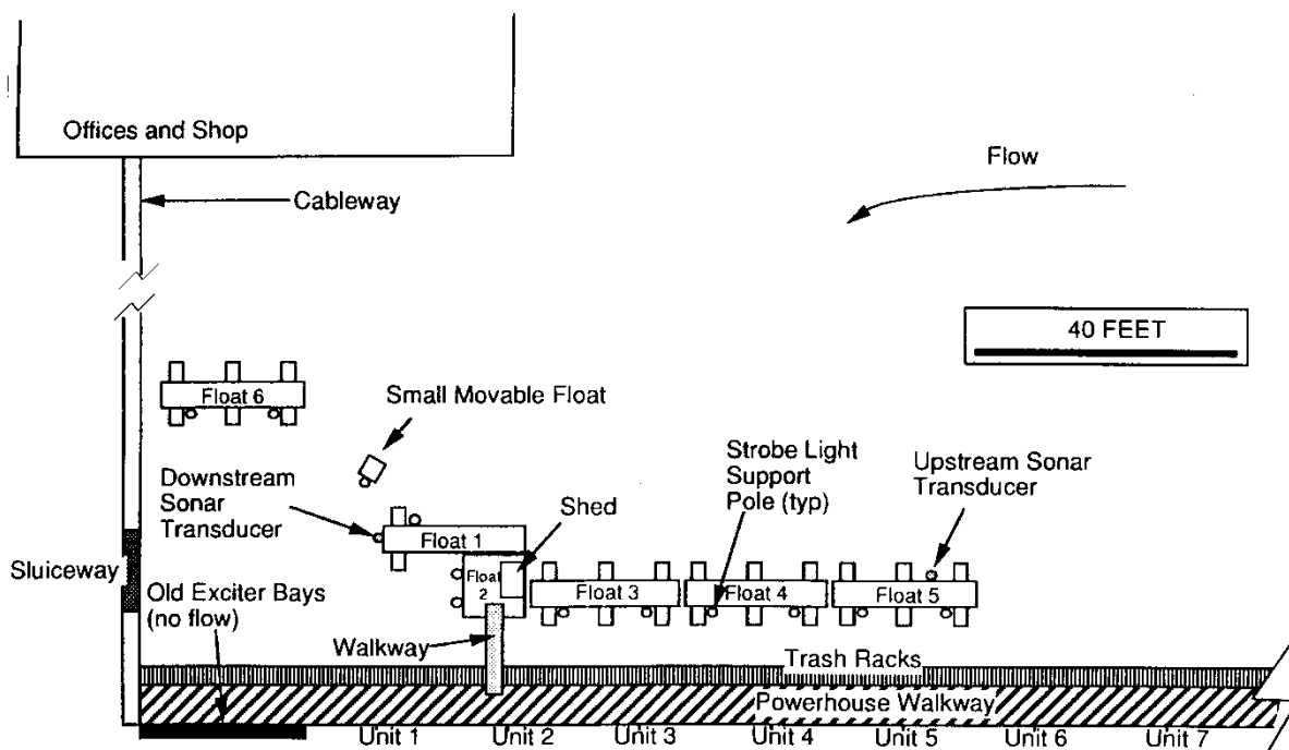
Figure 13-2 1991 forebay and float positions, York Haven Hydroelectric Project (Taft et al. 2001)
