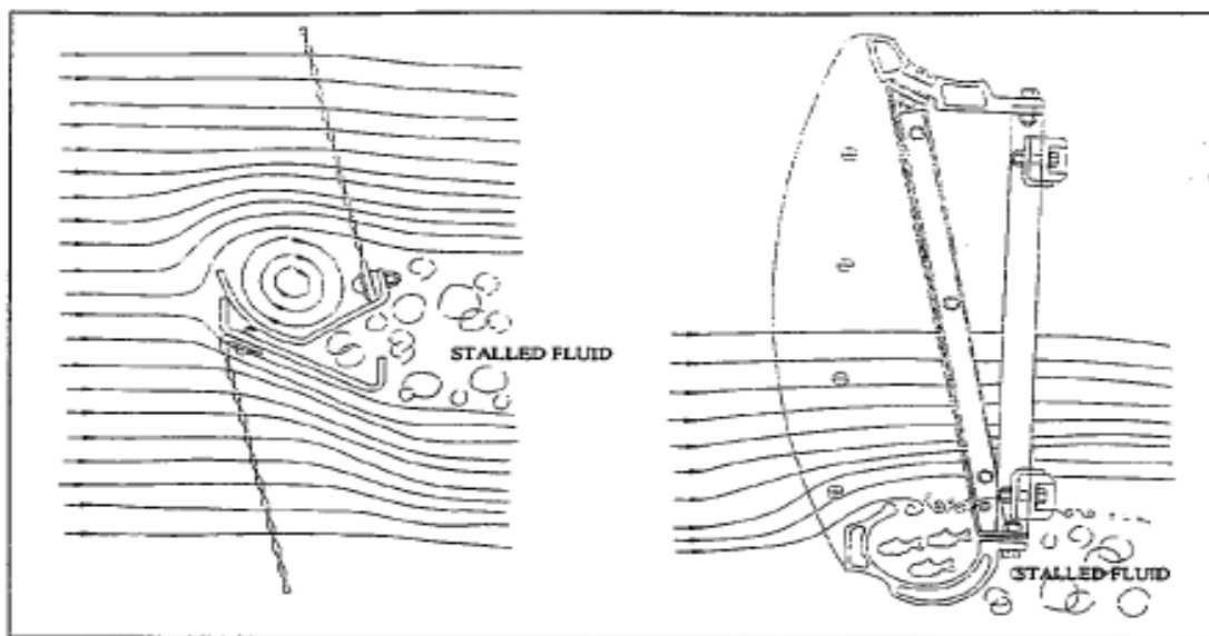
Figure 2-4 Section of an old fish basket design (left) and a new fish basket design (right) illustrating the flow field created by each (Ronafalvy et al. 2000)
