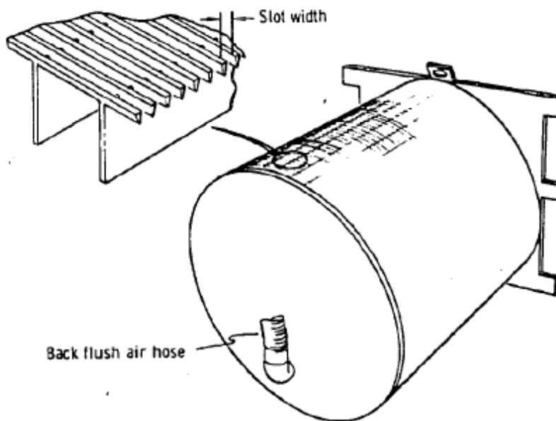
Figure 5-6 Drawing of a bulkhead-mounted screen with cut away of wedgewire configuration (Weisberg et al. 1987)
