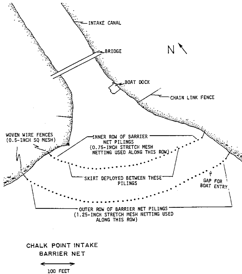
Figure 6-4 Chalk Point barrier net configuration (Loos 1986a, b)
