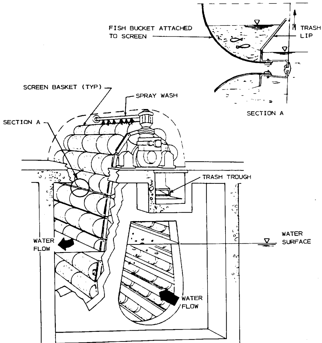
Figure 2-15 Center-flow (Passavant) screen (Murray and Jinette 1978)
