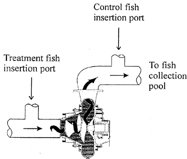
Figure 9-6 Cross-sectional view of the Hidrostal pump and fish injection ports (the fish protective impeller shroud is not shown in this drawing) (Helfrich et al. 2001).
