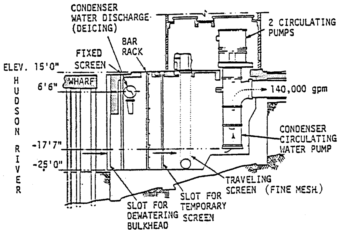
Figure 2-14 Section view of Indian Point Generating Station Unit 1 CWIS (EA 1977)
