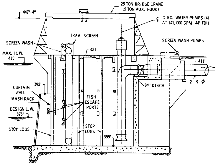
Figure 2-18 Section view of HGP intake structure (Page et al. 1977)
