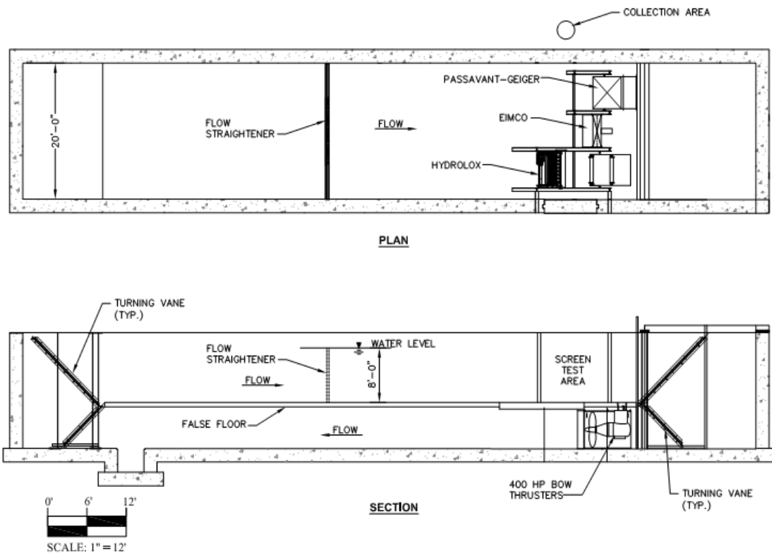
Figure 2-26 Plan and section of prototype-scale test flume (EPRI 2010a)
