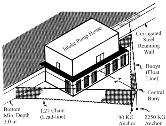
Figure 6-2 Bowline Point barrier net configuration (LMS 1978)
