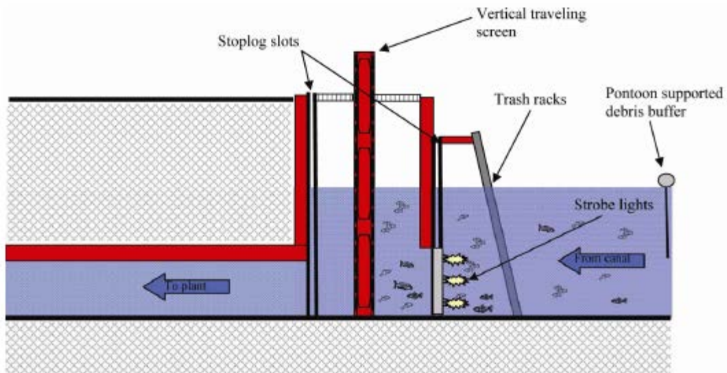
Figure 16-4 Location of the strobe light frames within the stoplog slots of Units 4-5 CWIS
