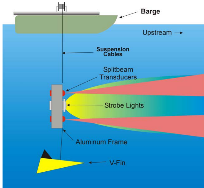
Figure 13-5 Deployment of strobe lights and hydroacoustic transducers from fixed barge (Simmons et al. 2002)
