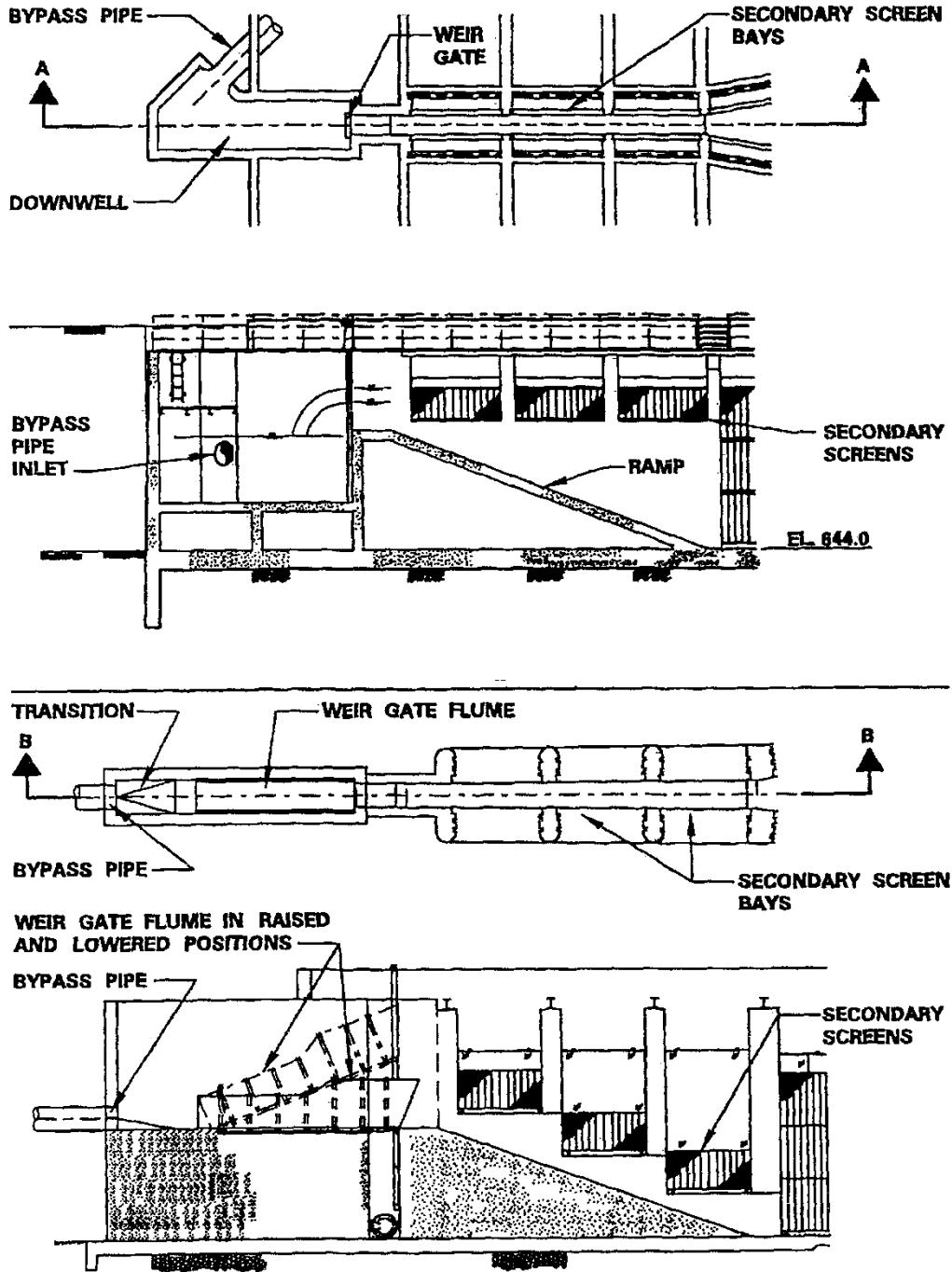
Figure 10-6 White River screen system — section view (Dorrtcague et al. 1996)
