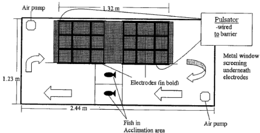
Figure 17-6 Overhead schematic of electric barrier test facility (Dawson et al. 2006)
