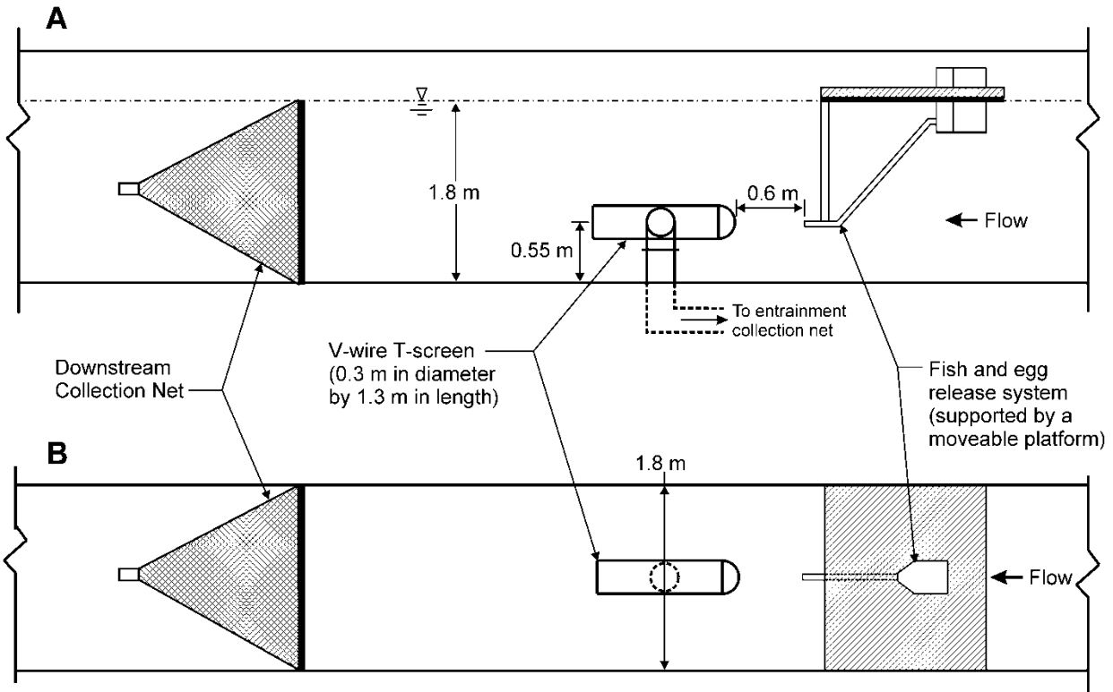
Figure 5-9 2002 wedgewire screen test facility (EPRI 2003)
