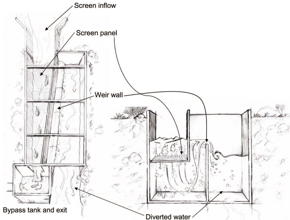
Figure 3-2 Plan and side conceptual views of Farmer screen (Mesa 2012)
