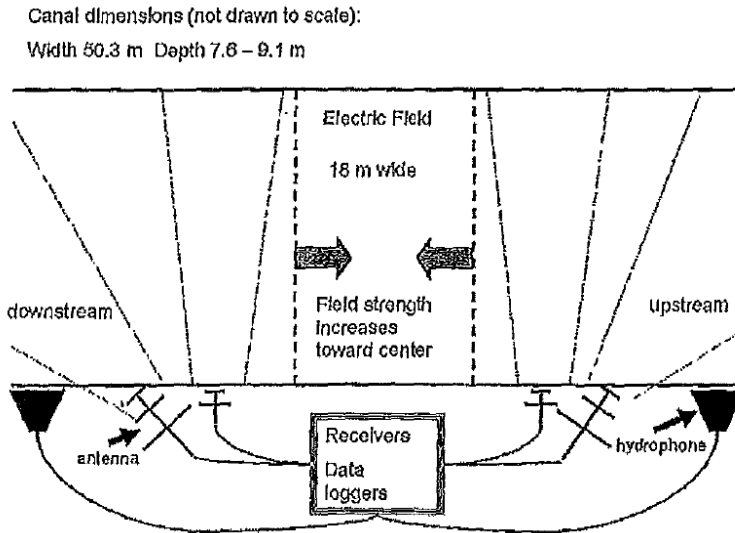
Figure 17-5 Arrangement of antennas and hydrophones at the barrier (Sparks et al. 2010)
