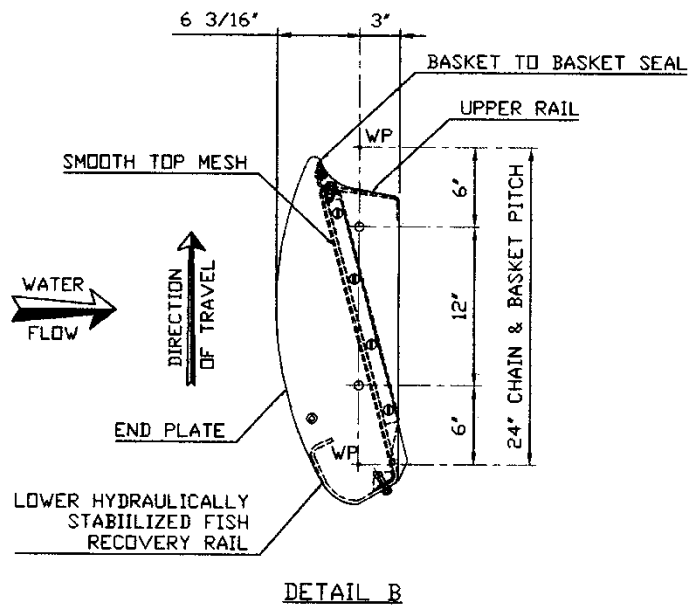
Figure 2-6 Modified dual-flow screen at Dunkirk Station (Beak 1988)
