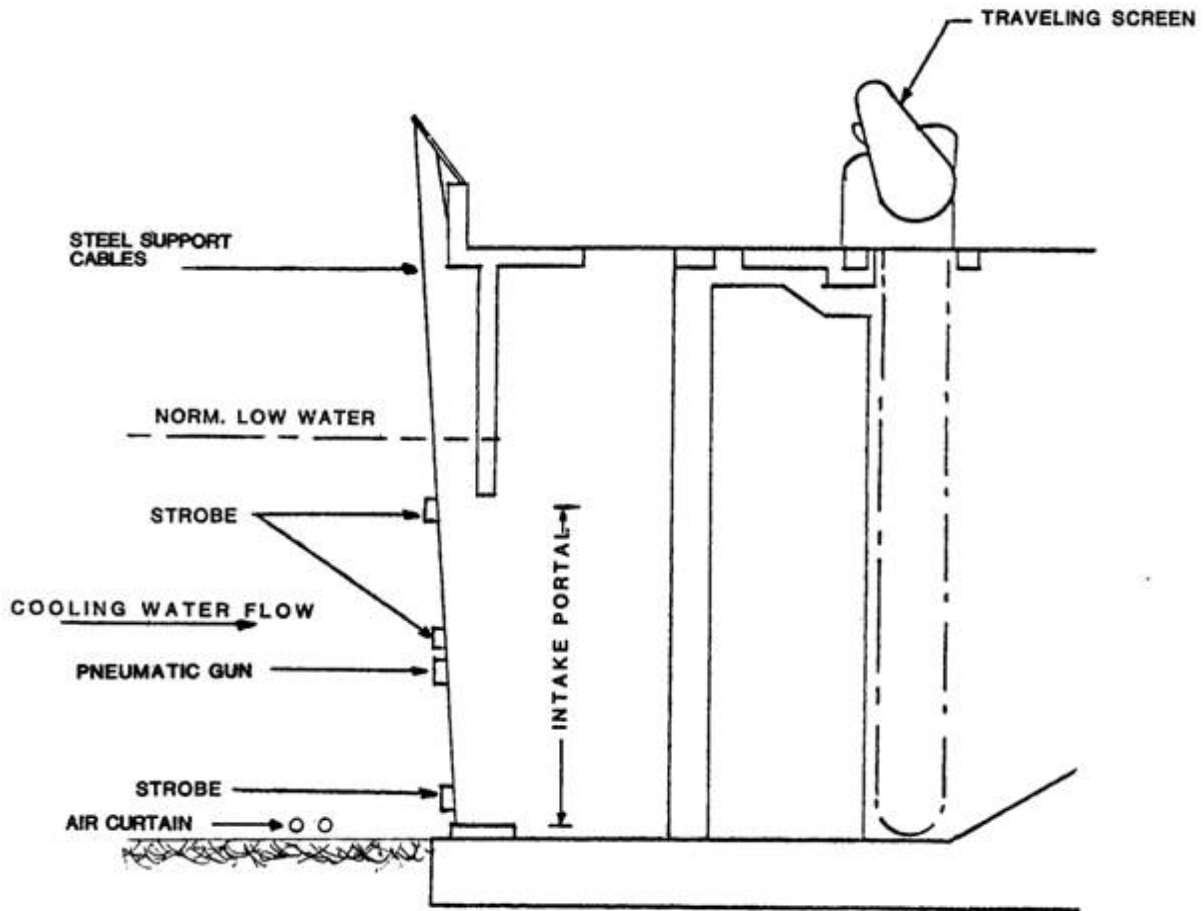
Figure 13-1 Roseton intake structure behavioral barriers — section (EPRI 1999)
