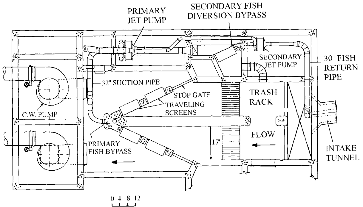
Figure 10-1 Oswego Unit 6 angled screen layout (LMS 1992)
