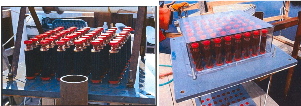
Figure 17-1 Top candle array of IMOD shown with (left) and without (right) the impingement enclosure box (Normandeau 2007).
