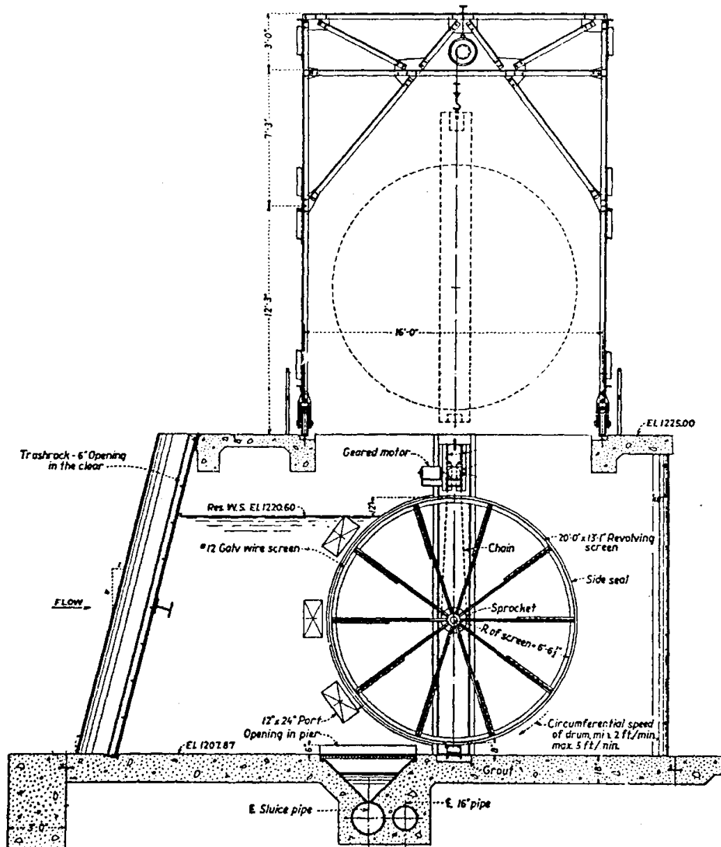
Figure 4-1 Typical drum screen (EPRI 1986a)
