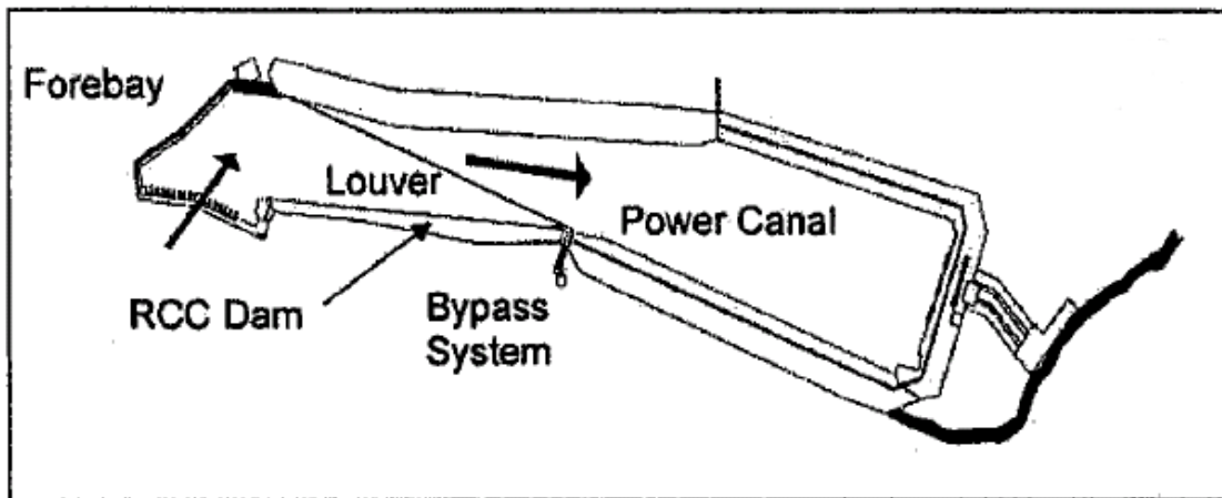
Figure 12-2 Schematic diagram of the Grand Falls Power Canal, showing louver line, bypass, and dam (Scruton et al. 2003)
