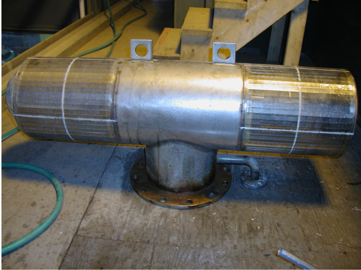
Figure 5-10 Johnson T-12 cylindrical wedgewire screen (white lines delineate sections of the screen for which impingement locations were recorded) (EPRI 2003)
