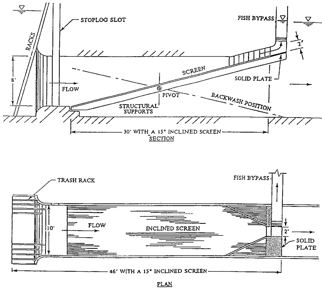
Figure 11-1 Modular inclined screen (Taft et al. 1995)
