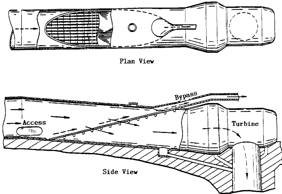
Figure 11-2 Eicher Screen (EPRI 1992a)
