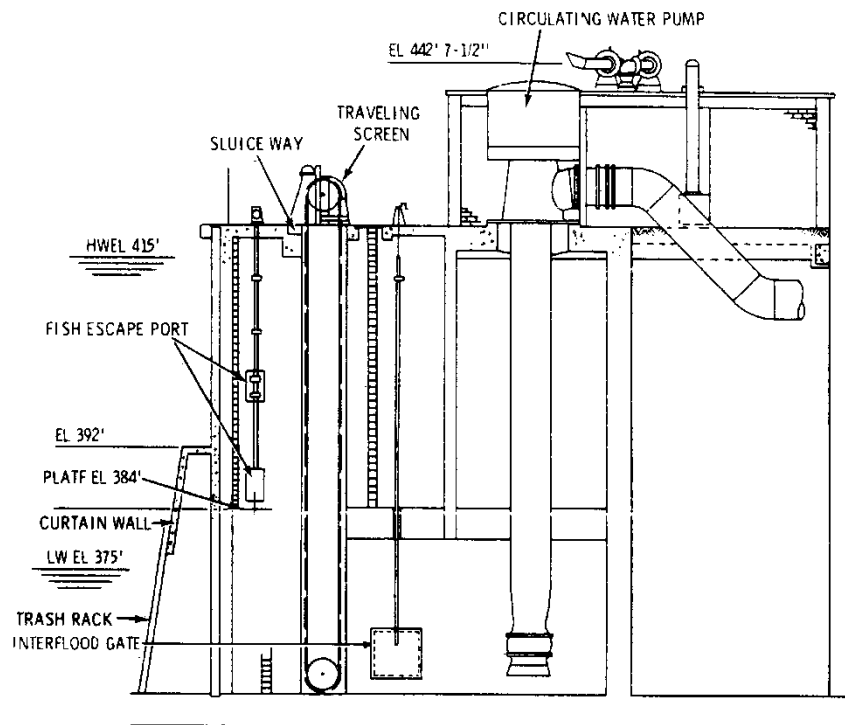
Figure 2-17 Section view of 100-N intake structure (Page et al. 1977)
