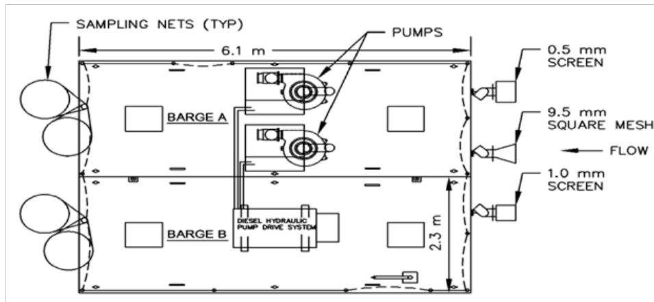
Figure 5-13 Floating test facility (barge) – plan view (Alden 2010)
