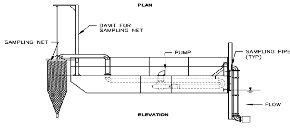
Figure 5-14 Floating test facility (barge) – elevation view (Alden 2010)
