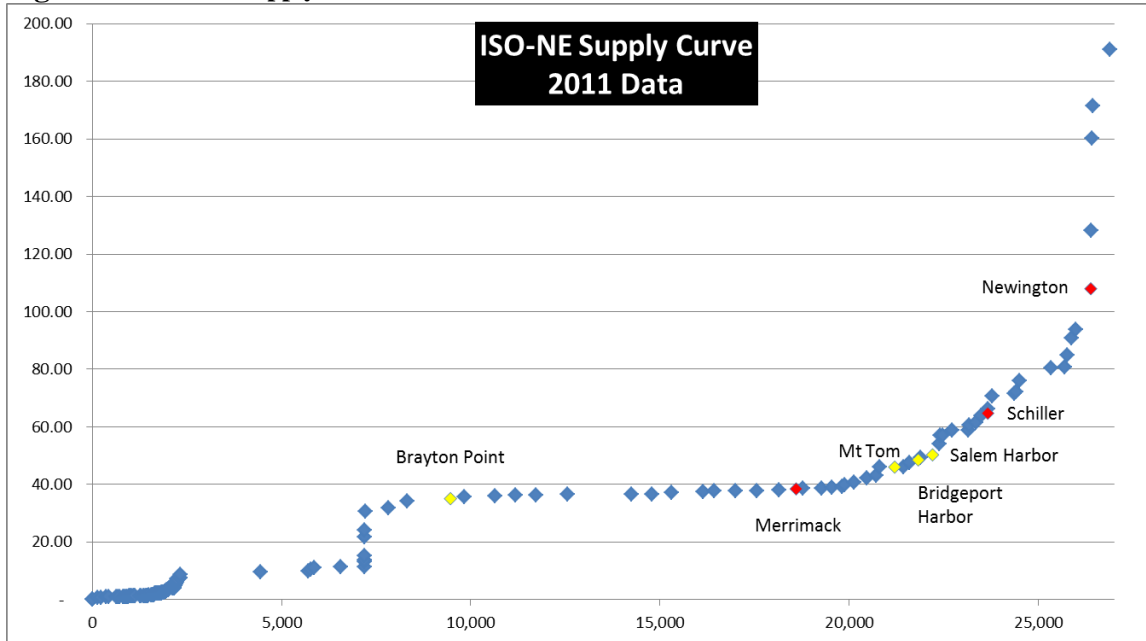
Figure 8: ISO-NE Supply Curve
