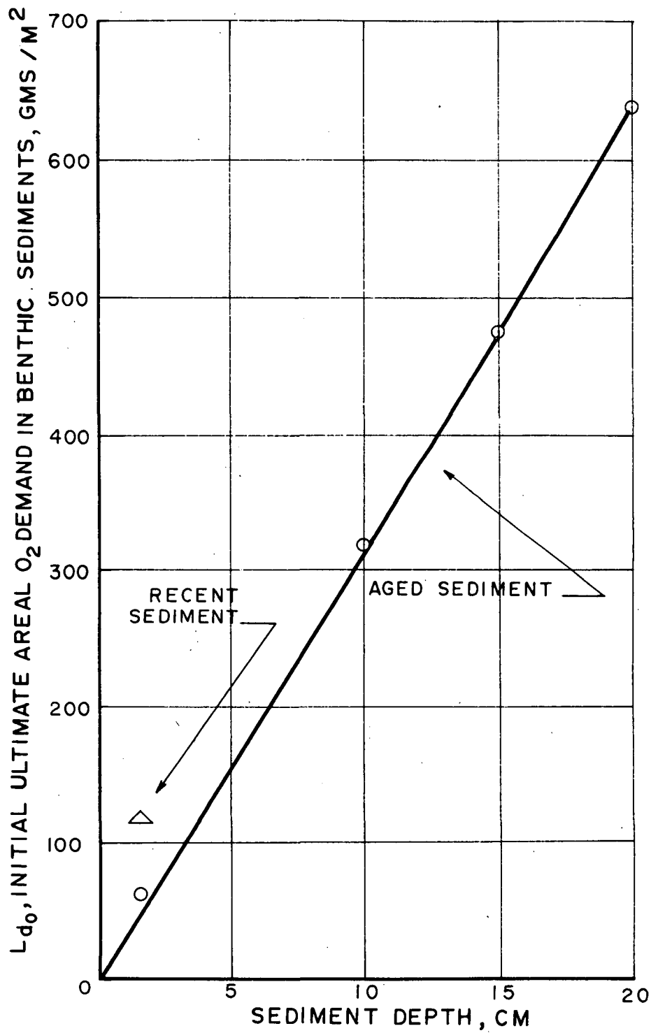
CALCULATED L_{d0} VS. SEDIMENT DEPTH
