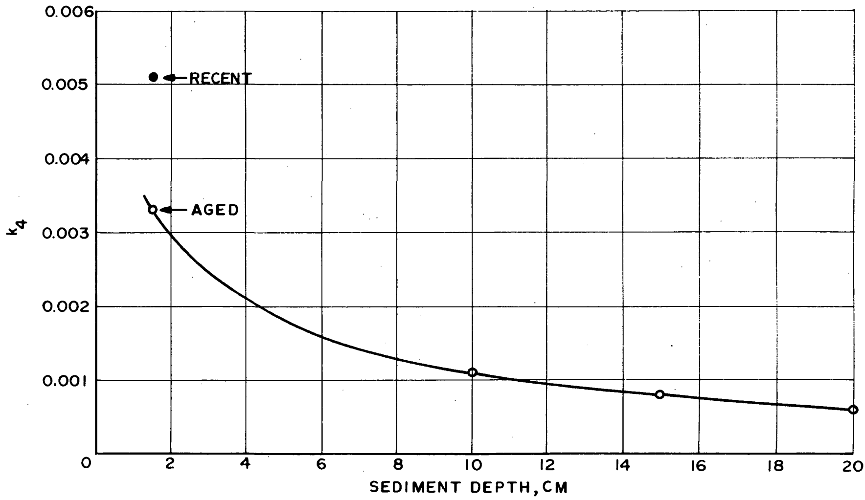
K_4 vs SEDIMENT DEPTH
