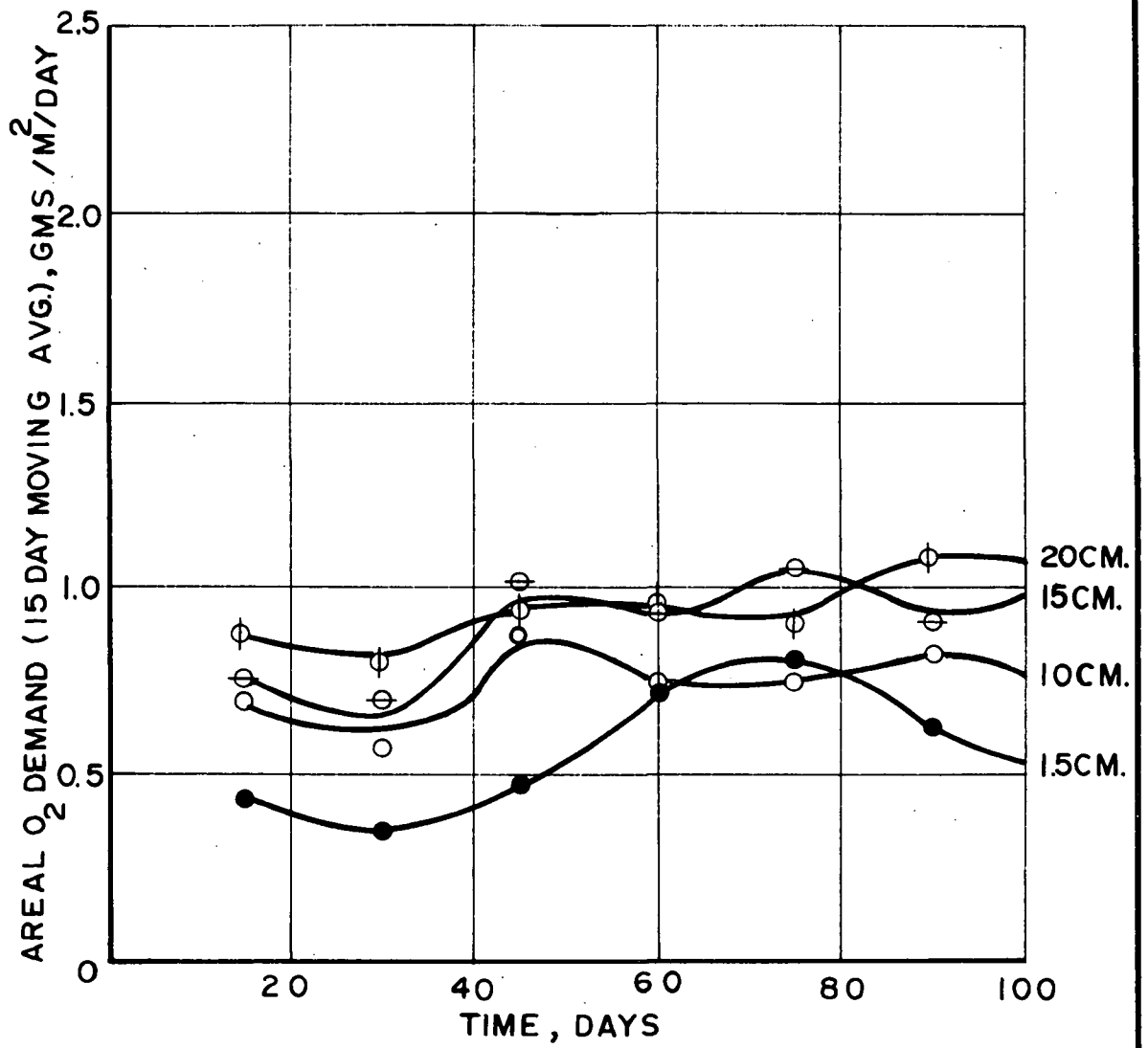
AREAL O_2 DEMAND OF AGED BENTHIC SEDIMENTS
