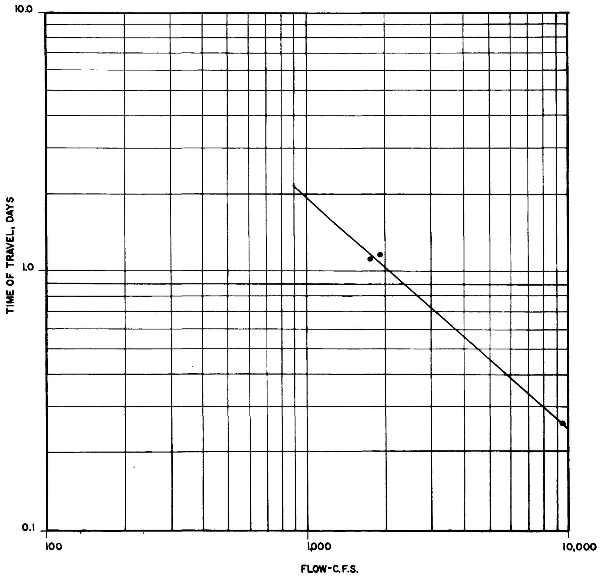
MERRIMACK RIVER TIME OF TRAVEL VS. FLOW - LAWRENCE TO LITTLE RIVER
