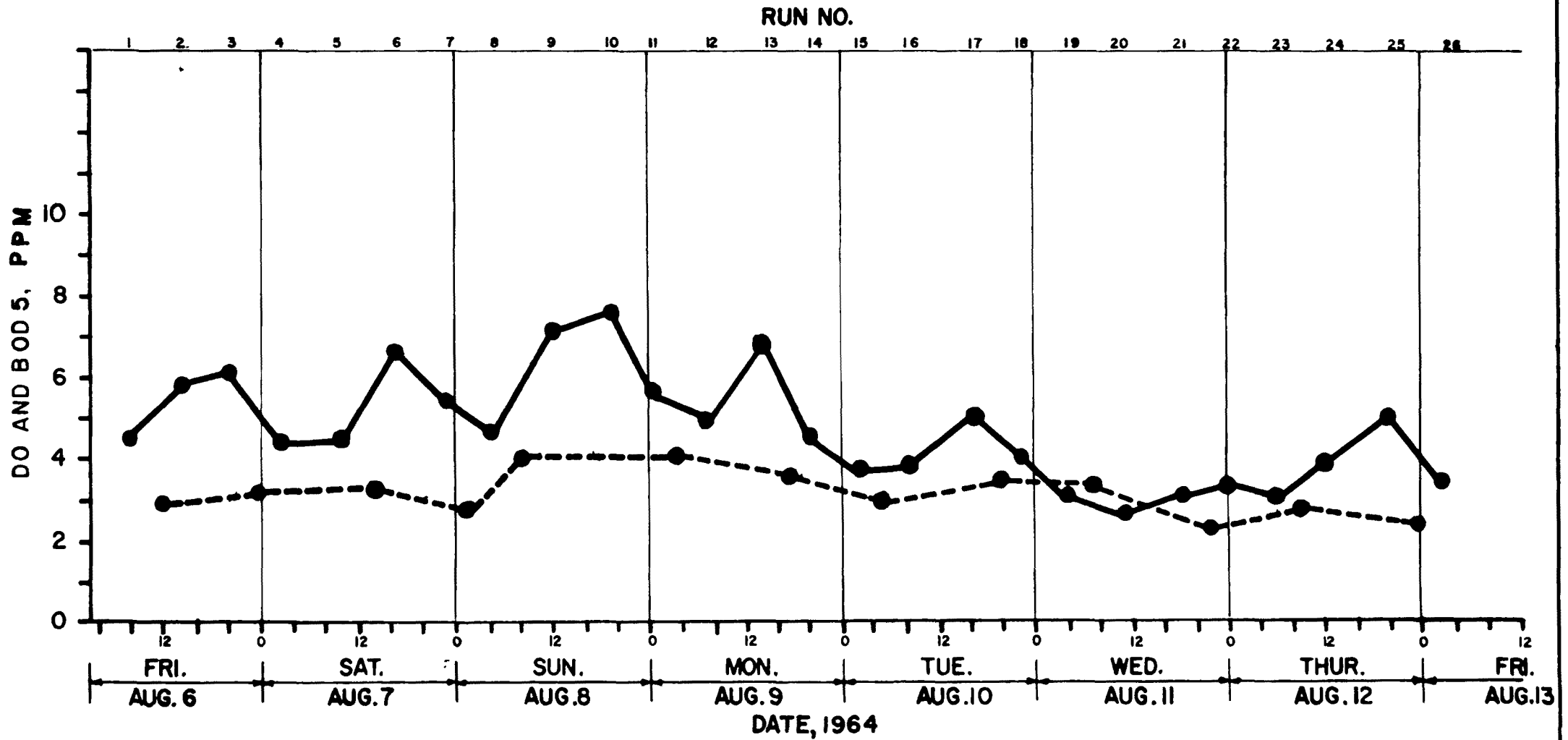
TYPICAL DISSOLVED OXYGEN & BOD PATTERNS IN THE MERRIMACK RIVER
