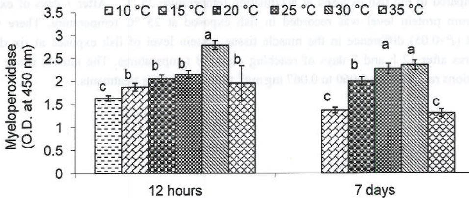
Fig. 2. Myeloperoxidase level of C. batrachus exposed to six different temperatures. Bars with different superscripts are significantly ( P<0.05 ) different ( n=6 ).
