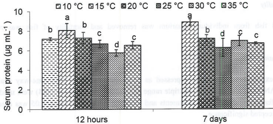
Fig.1. Effect of acclimation temperature on the serum protein level of C. batrachus . Bars with different superscripts are significantly ( P<0.05 ) different ( n=6 ).
