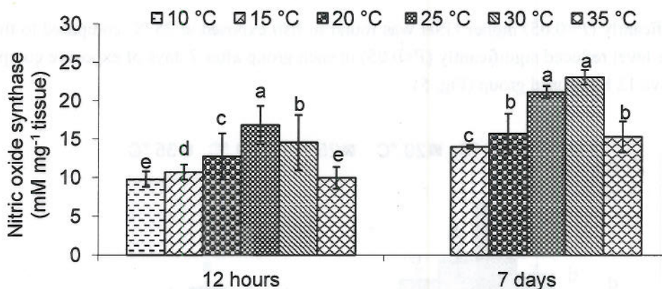
Fig. 3. Effect of acclimation temperature on the nitric oxide synthase of C. batrachus . Bars with different superscripts are significantly ( P < 0.05 ) different ( n=6 ).
