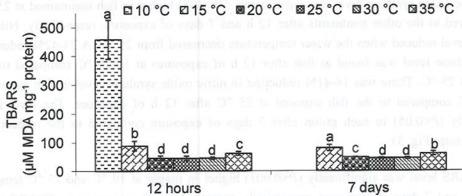
Fig. 4. Thiobarbituric acid reactive substance (TBARS) found in C. batrachus after exposure to six different temperatures. Bars with different superscripts are significantly ( P < 0.05 ) different ( n=6 ).
