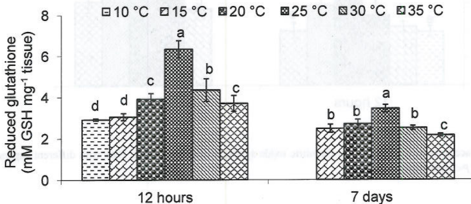
Fig. 5. Effect of acclimation temperature on reduced glutathione (GSH) of C. batrachus . Bars with different superscripts are significantly ( P < 0.05 ) different ( n=6 ).
