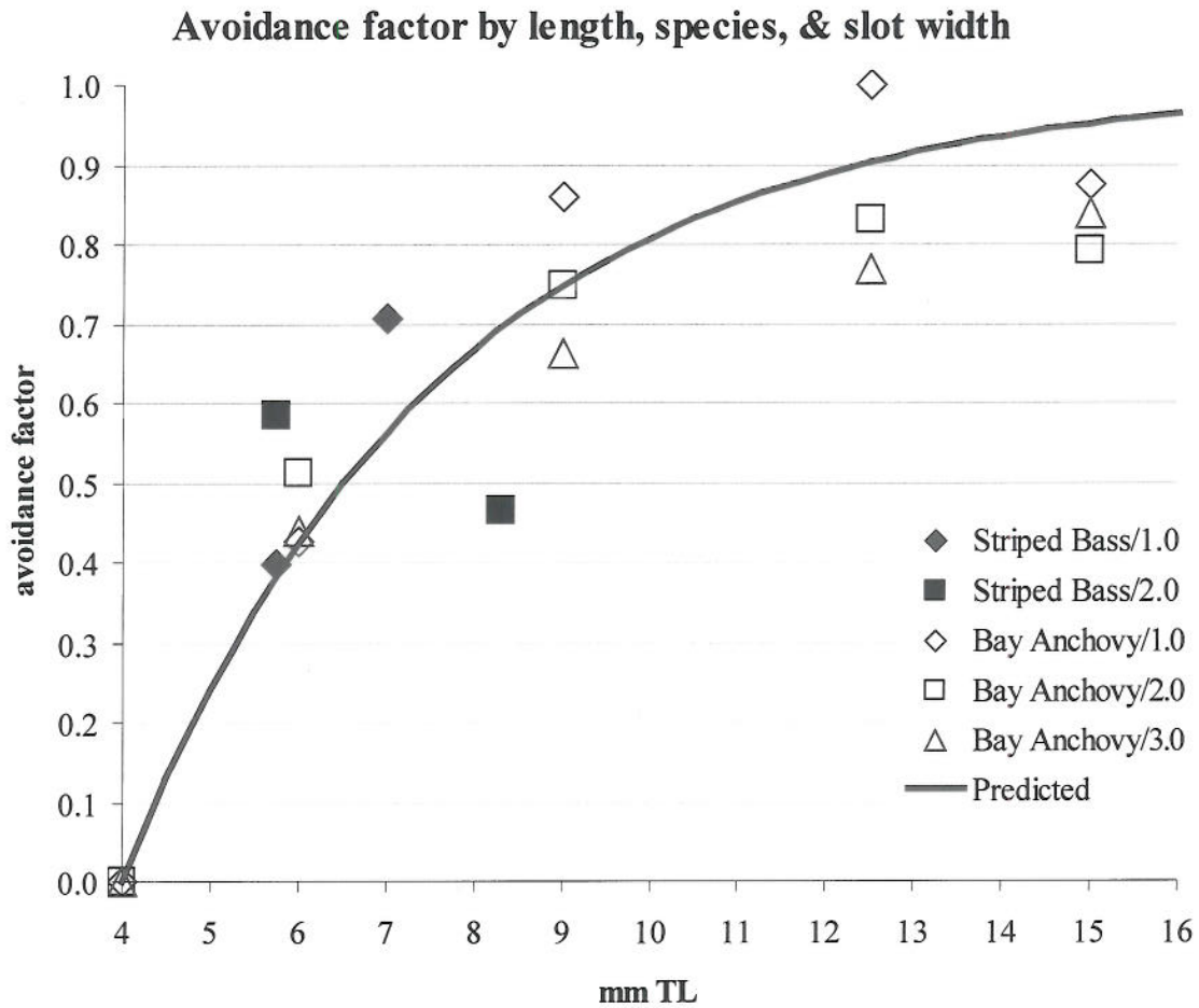
Figure 2-1. Observed and predicted relationship between length (mm total length) of striped bass or bay anchovy larvae and avoidance factor (the proportion avoiding entrainment) for cylindrical wedgewire screens with slot widths of 1.0 mm, 2.0 mm or 3.0 mm.
