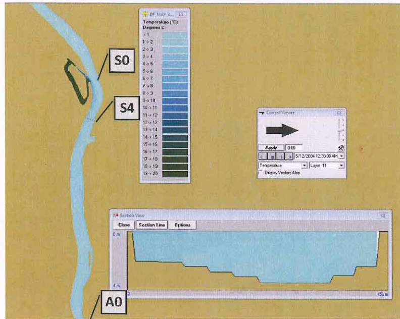
Figure 3-2. Model predicted delta temperature contours at 50 th percentile upstream ambient condition during the early spring biological period for an average year: 7-14 May 2004. Surface temperatures and cross section at S4 shown.
