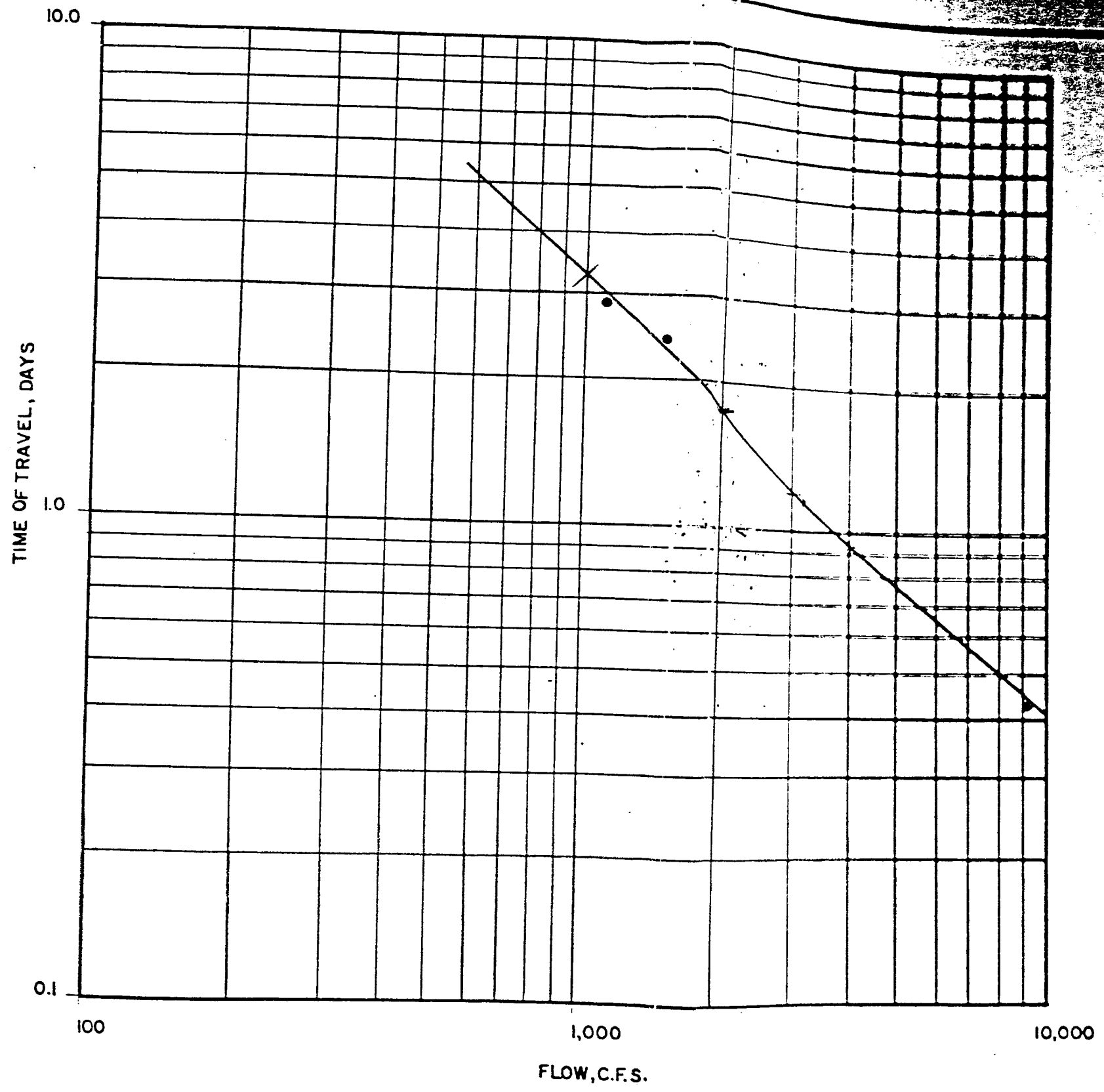
MERRIMACK RIVER TIME OF TRAVEL VS. FLOW - CONCORD RIVER TO LAWRENCE
