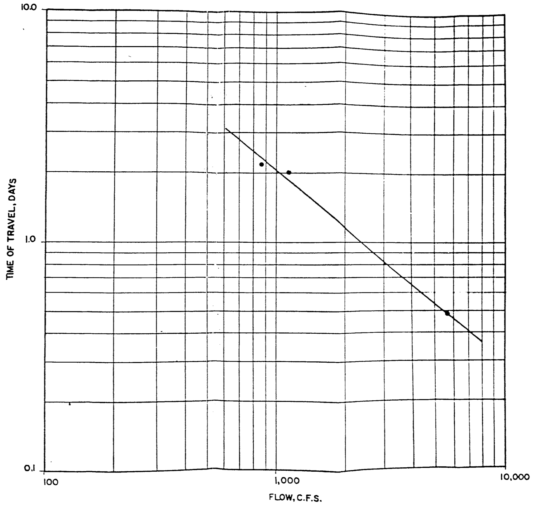
MERRIMACK RIVER TIME OF TRAVEL VS. FLOW - RT.3 BRIDGE, CONCORD TO HOOKSETT DAM
