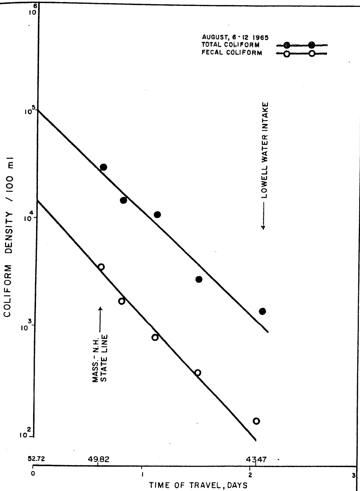
COLIFORM DENSITY DECLINE NASHUA TO LOWELL SUMMER
