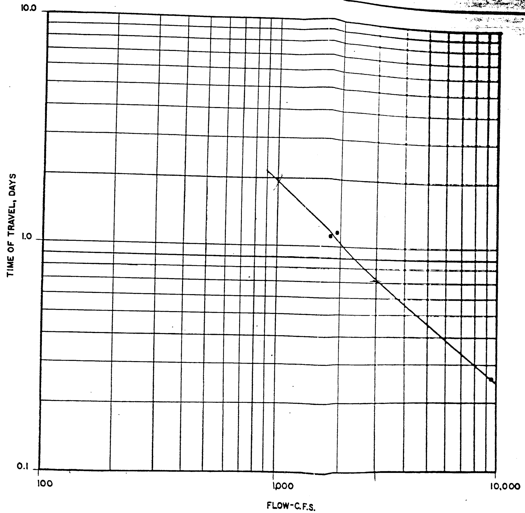
MERRIMACK RIVER TIME OF TRAVEL VS. FLOW - LAWRENCE TO LITTLE RIVER
