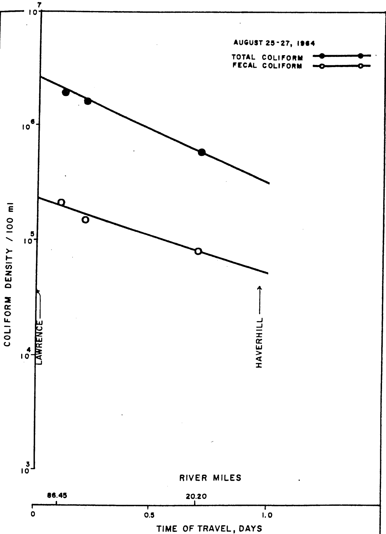
COLIFORM DENSITY DECLINE LAWRENCE TO HAVERHILL SUMMER
