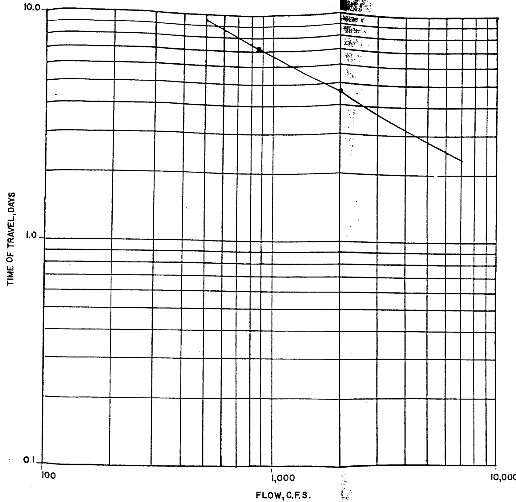
MERRIMACK RIVER TIME OF TRAVEL VS. FLOW - SEWALLS FALLS DAM TO RT. 3 BRIDGE, CONCORD
