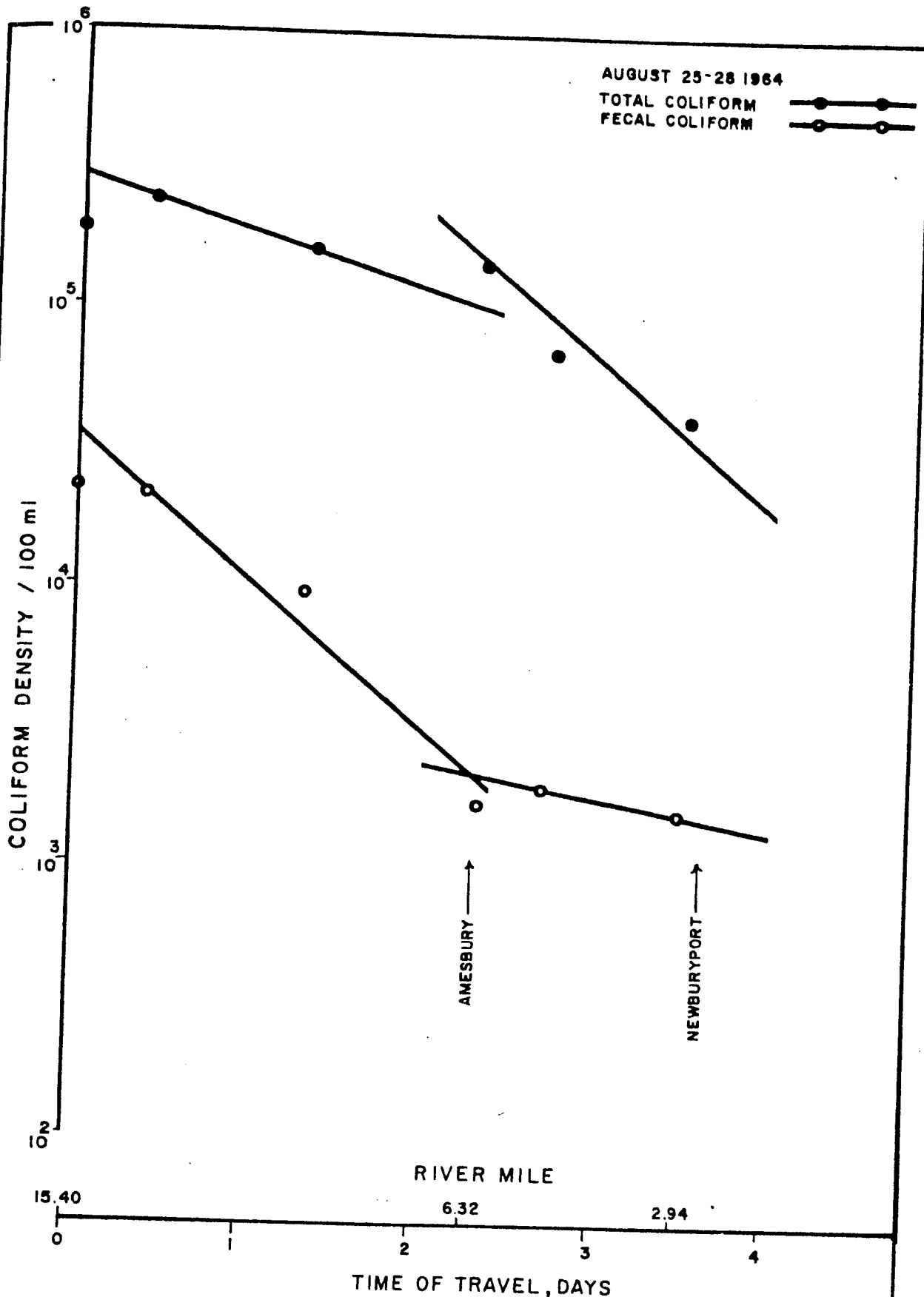
COLIFORM DENSITY DECLINE HAVERHILL TO NEWBURYPORT SUMMER
