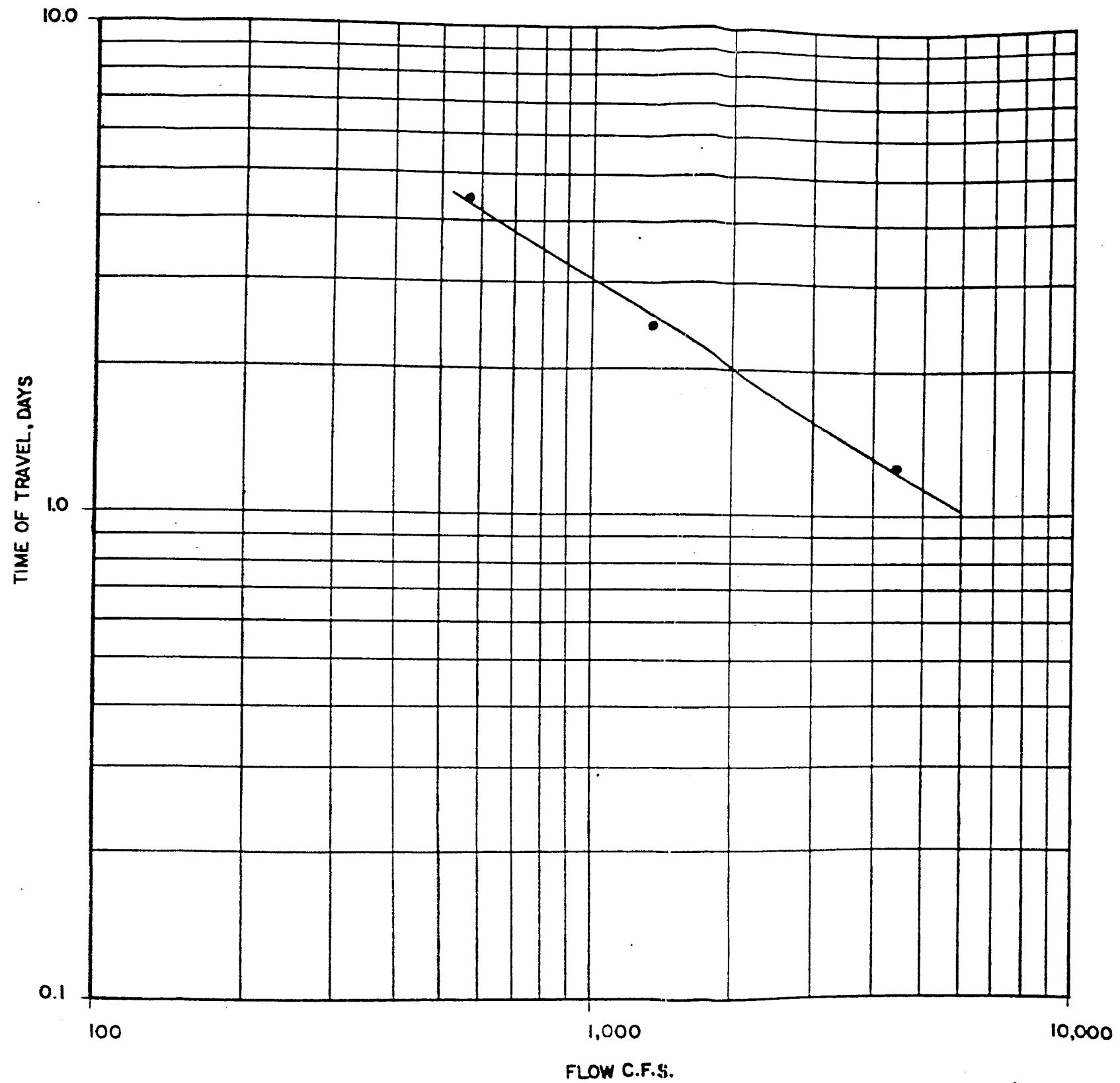
MERRIMACK RIVER TIME OF TRAVEL VS. FLOW - NASHUA RIVER TO CONCORD RIVER
