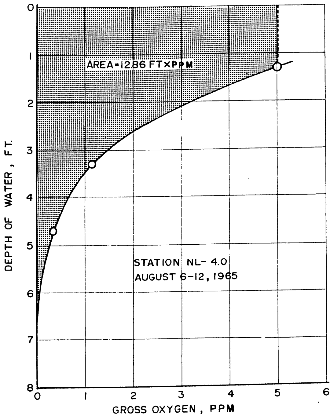
GROSS OXYGEN PRODUCTION VS. DEPTH
