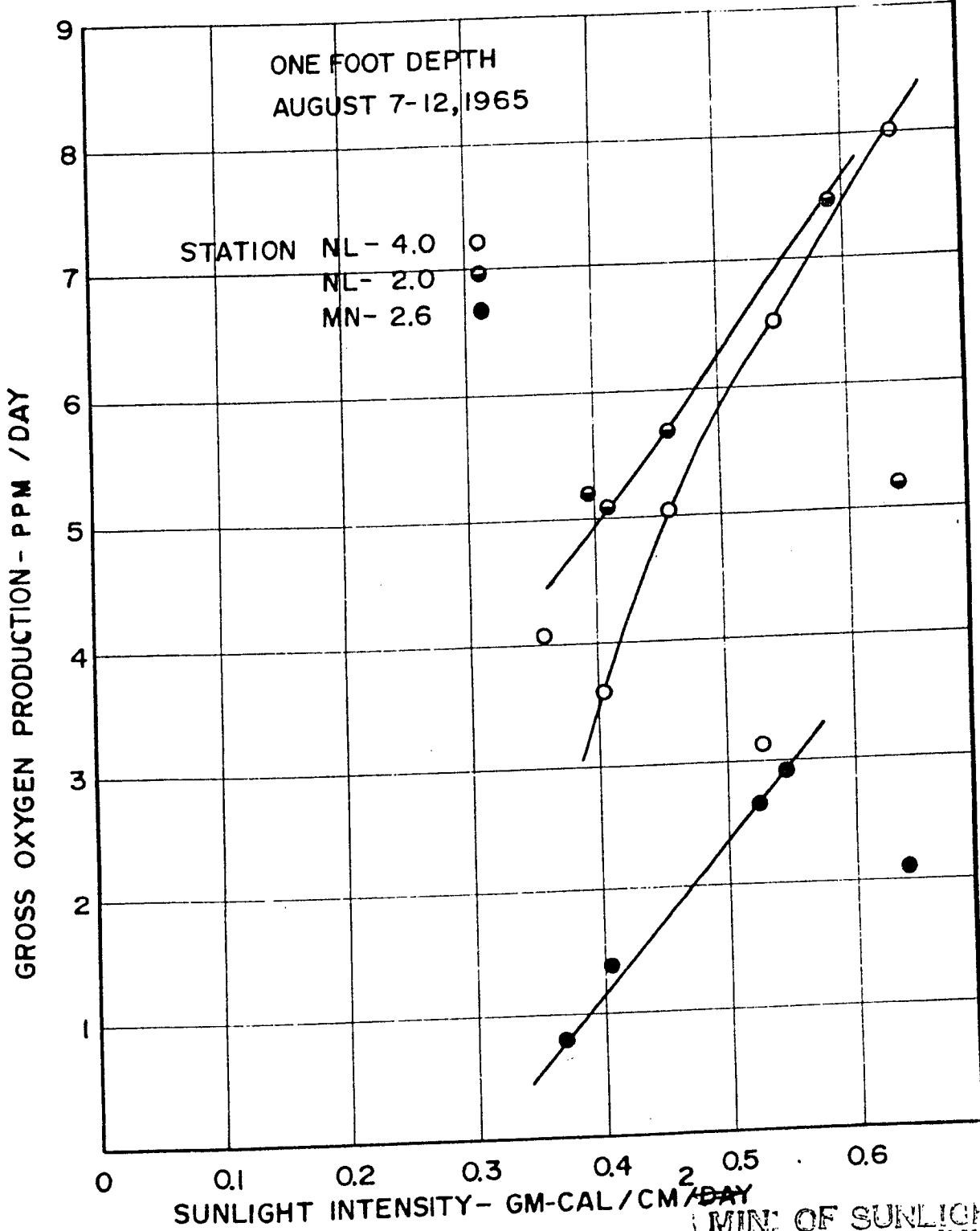
GROSS OXYGEN PRODUCTION VS. SUNLIGHT INTENSITY
