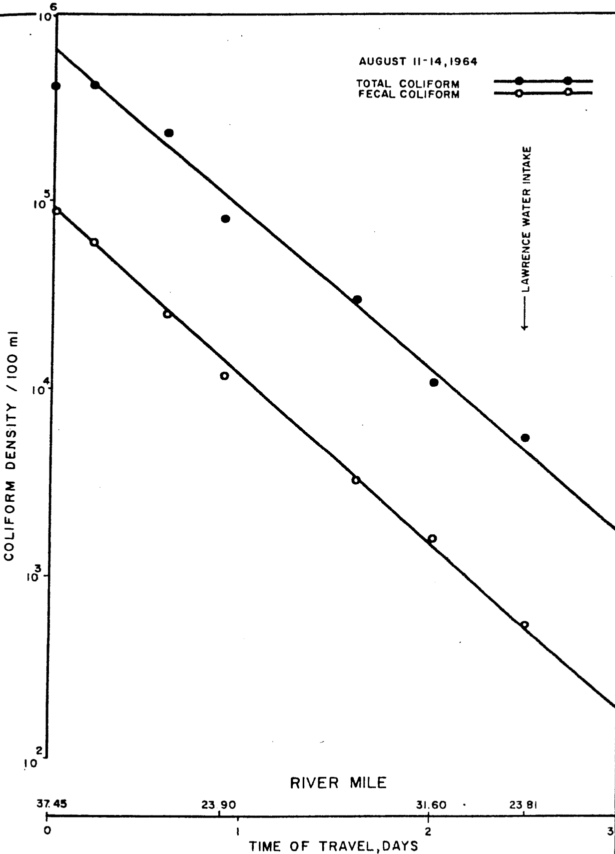
COLIFORM DENSITY DECLINE LOWELL TO LAWRENCE SUMMER
