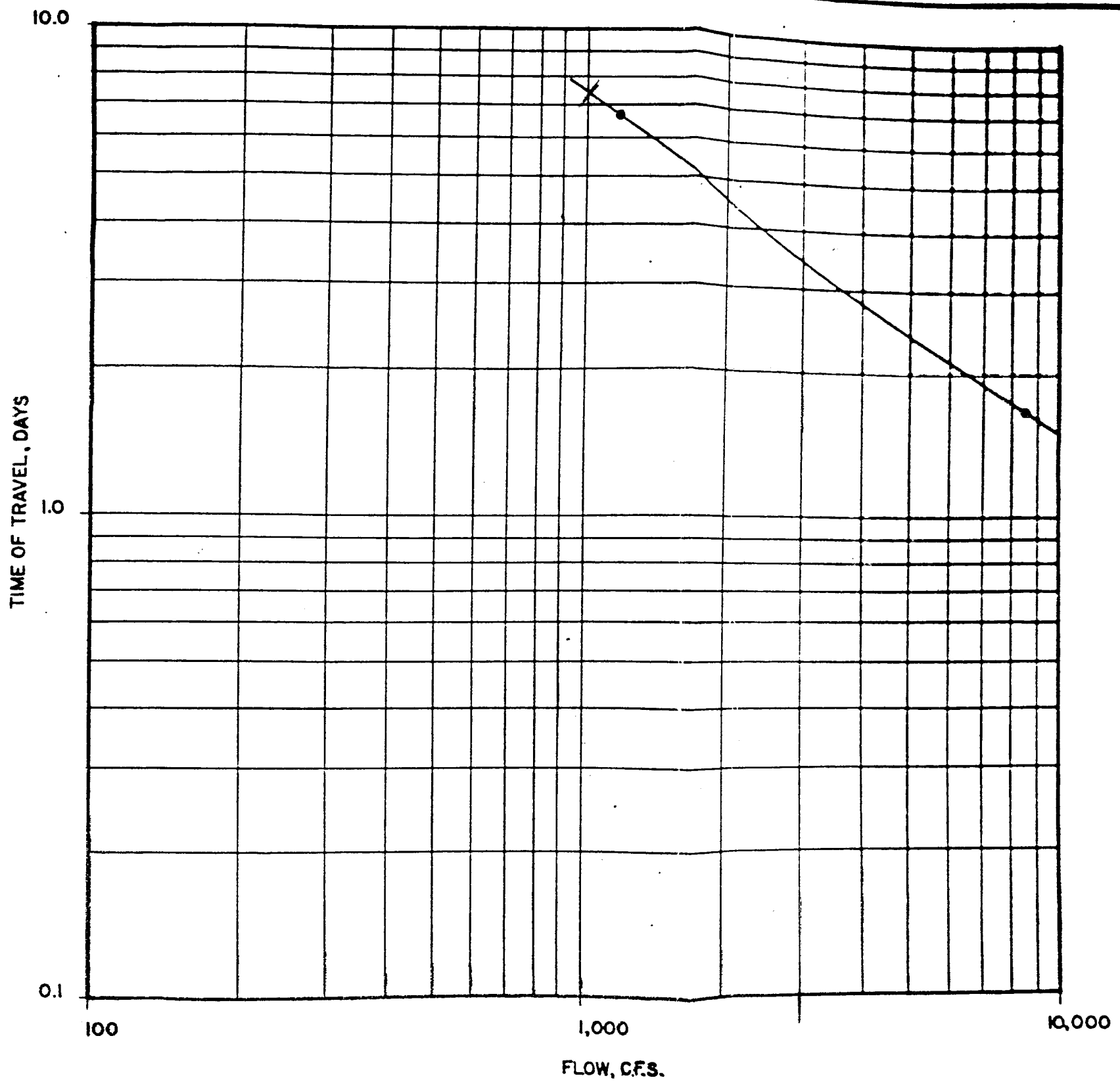
MERRIMACK RIVER TIME OF TRAVEL VS. FLOW - LITTLE RIVER TO NEWBURYPORT
