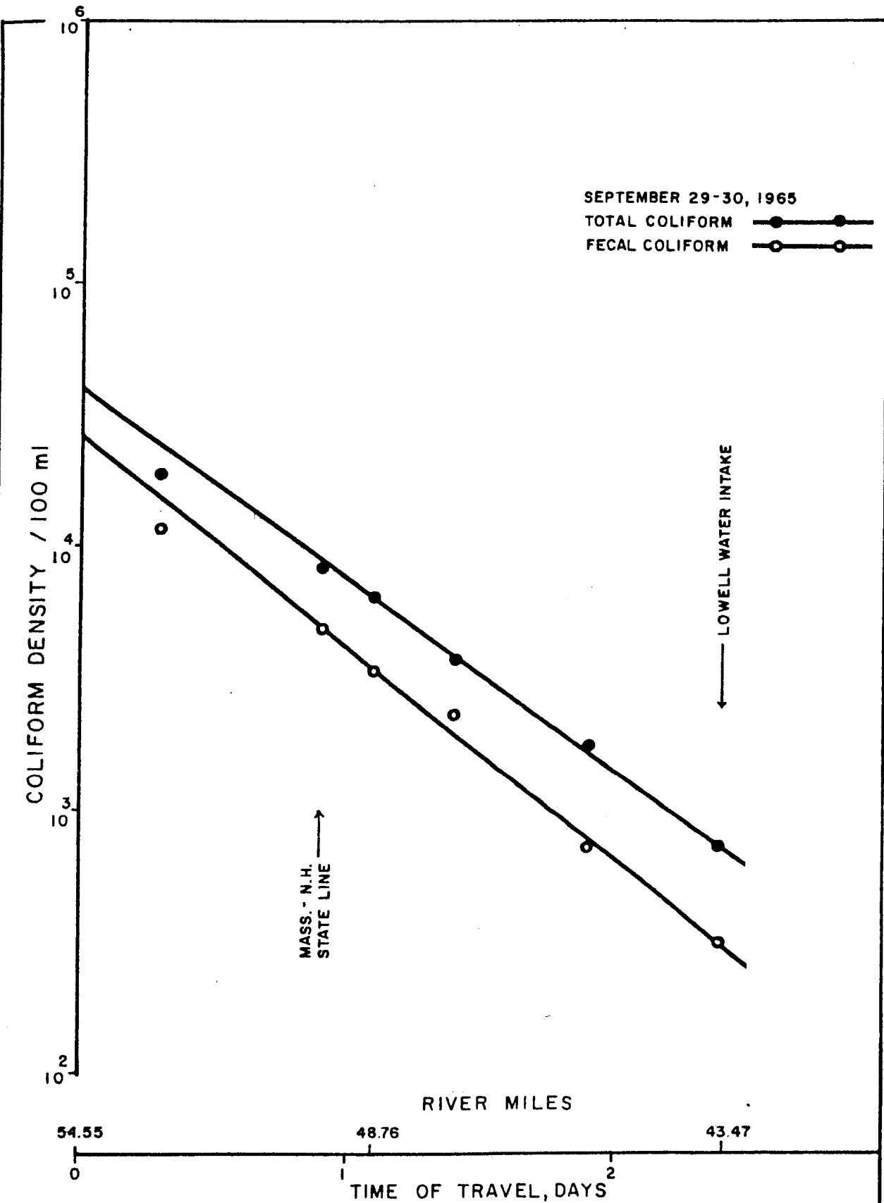
COLIFORM DENSITY DECLINE NASHUA TO LOWELL FALL
