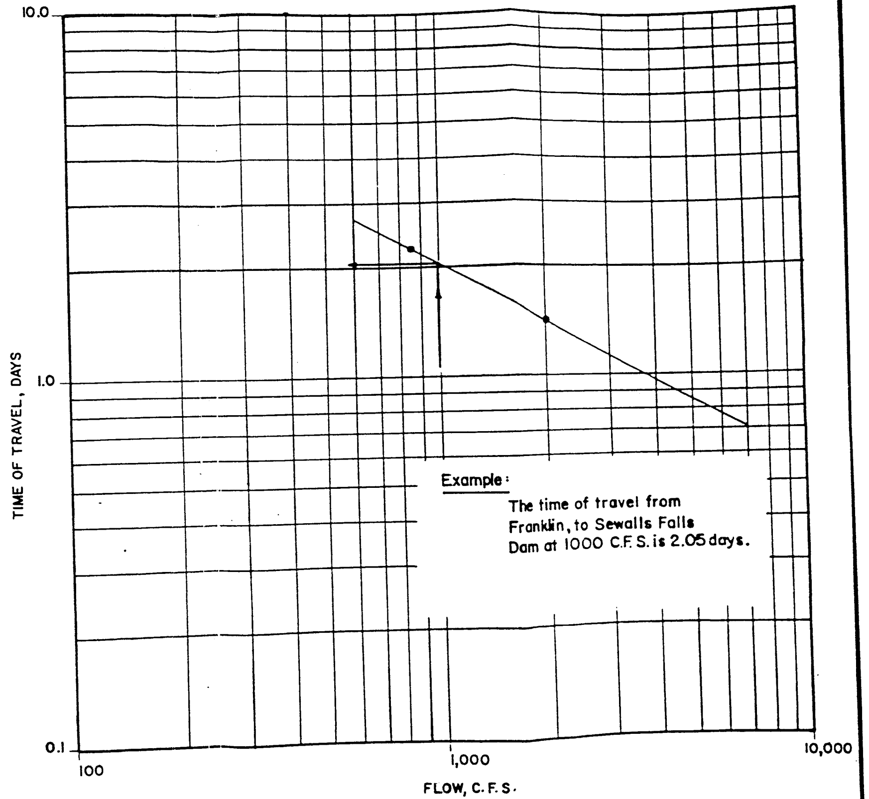
MERRIMACK RIVER TIME OF TRAVEL VS. FLOW - FRANKLIN, N.H. TO SEWALLS FALLS DAM
