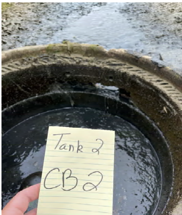
PHOTO 3: View of Minor Corroded/Damaged Stormwater intrusion at sidewall of Catch Basin.
