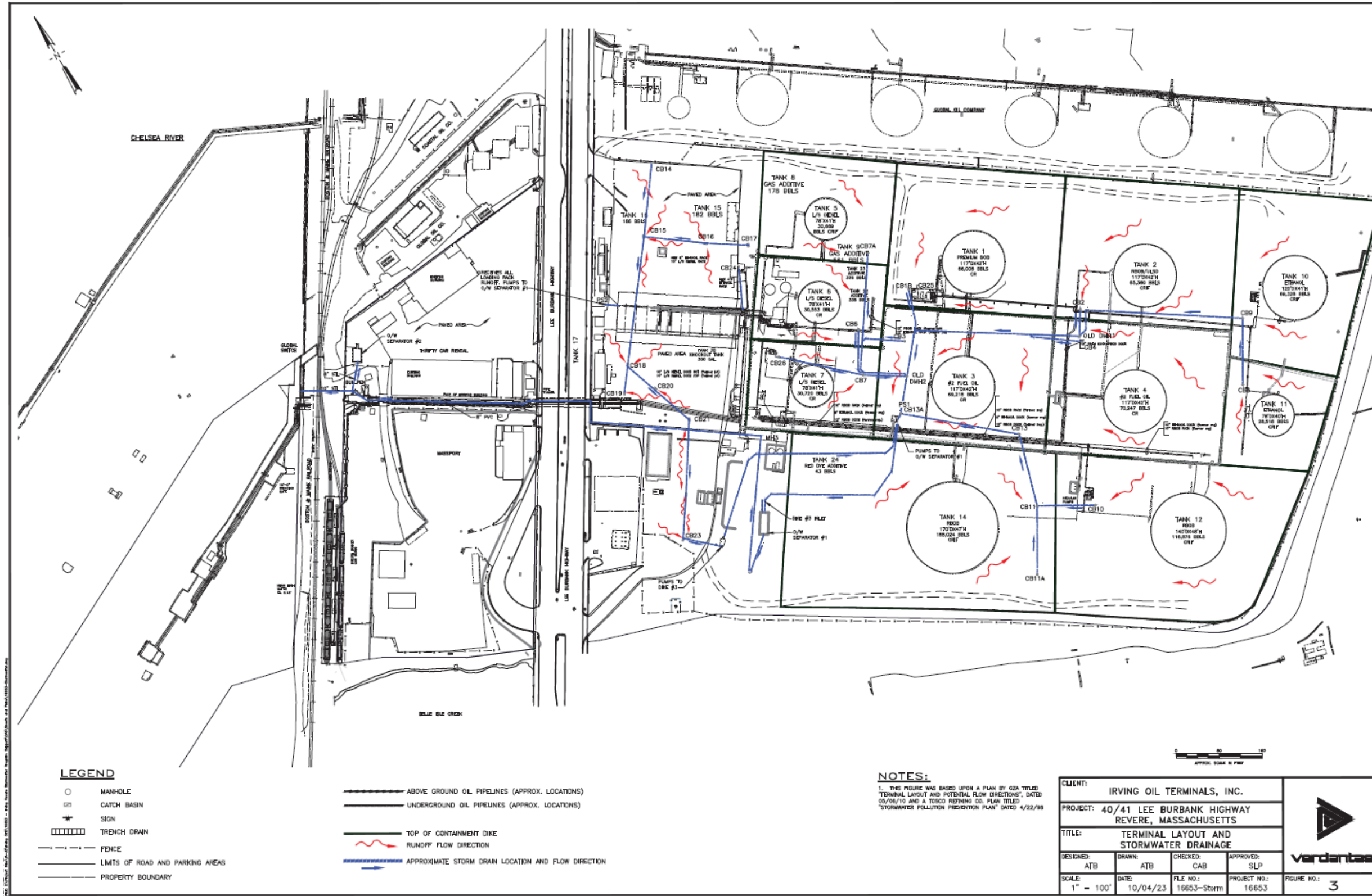
Figure 3: Terminal Drainage Plan
