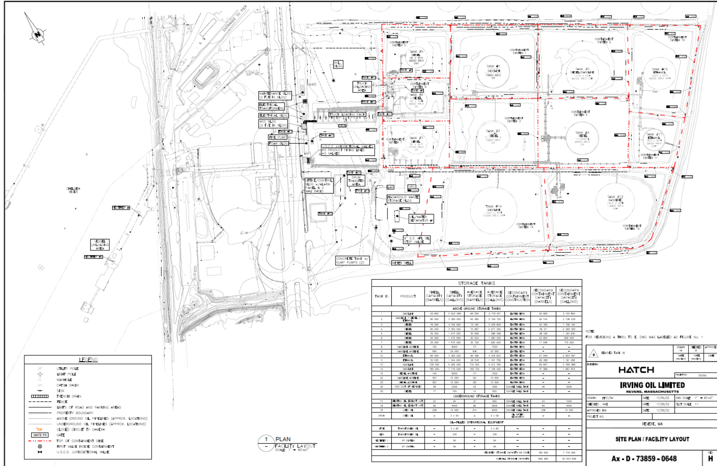
Figure 2A: Site Plan/Facility Layout
