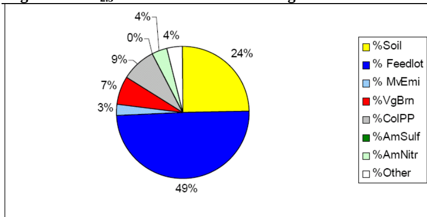
Figure 6. PM 2.5 Cowntown Monitor Average Source Contributions. 11
